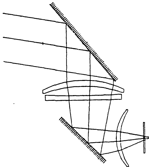
Fig 4.1(b) Common Module FLIR Full Azimuth Scan
