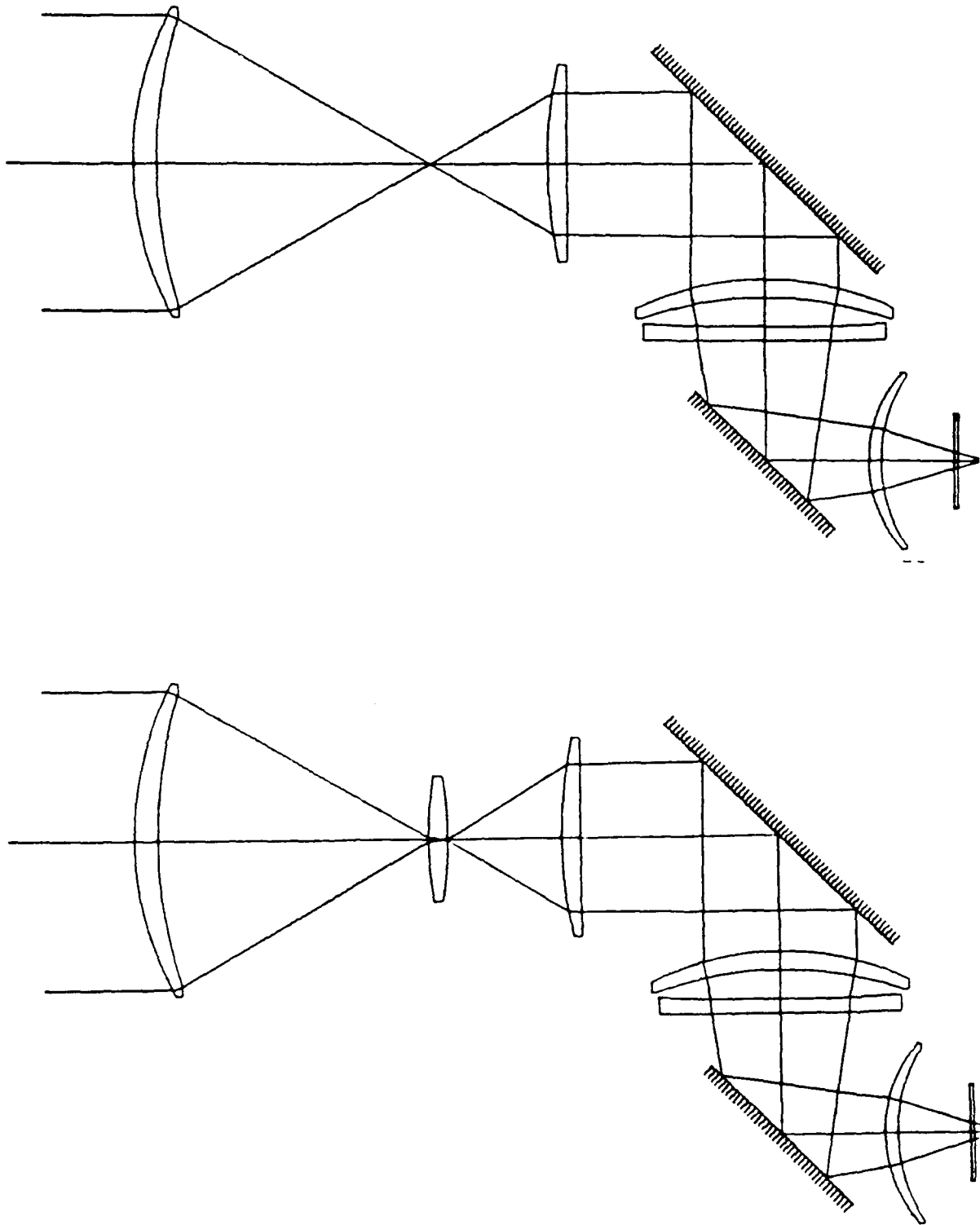
Fig 4.2 Narcissus of FLIR scanner
