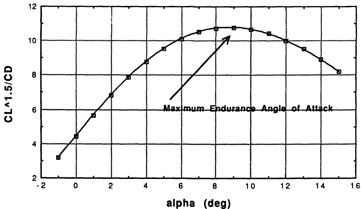
Figure 5.11 C_L^{3/2} / C_D versus Angle of Attack
