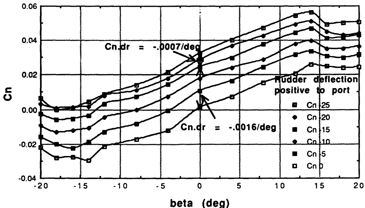
Figure 4.20 Yaw Moment Coefficient at 6° AOA
