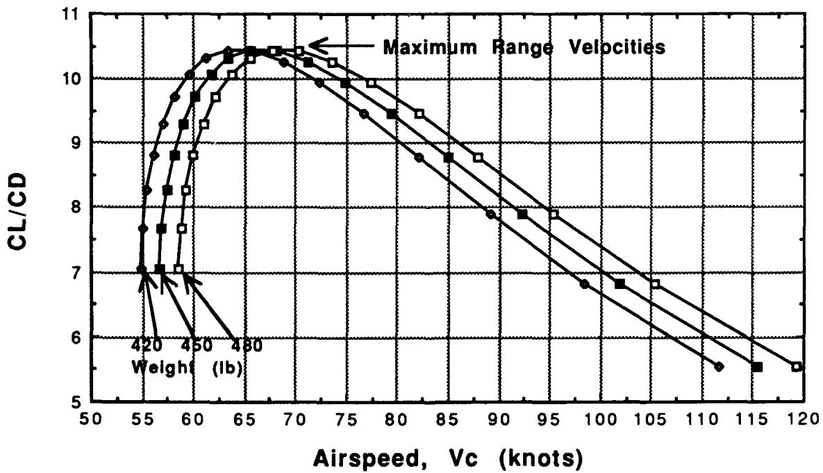
Figure 5.10 CL / CD versus Airspeed
