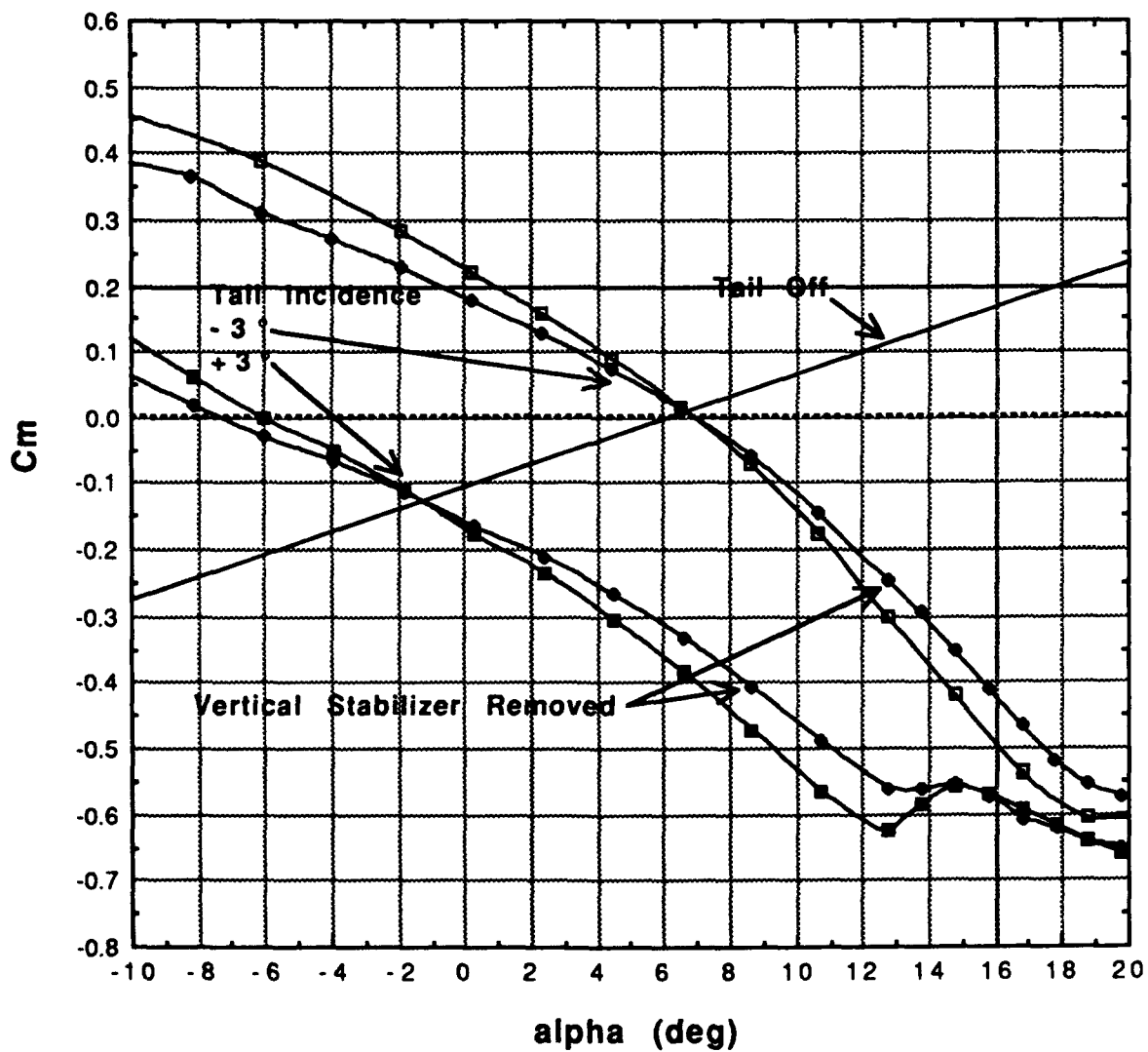
Figure 4.13 Finding Horizontal Tail Zero Angle of Attack
