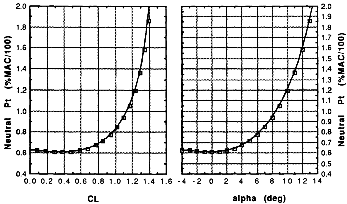
Figure 4.9 Stick Fixed Neutral Point
