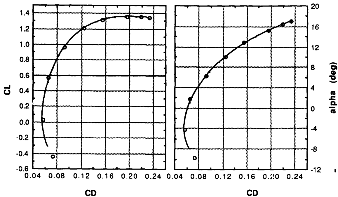
Figure 5.3 Drag Polar
