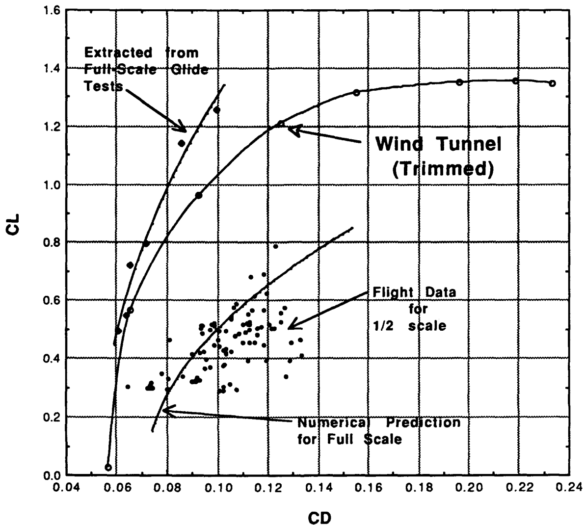
Figure 6.2 Drag Comparison
