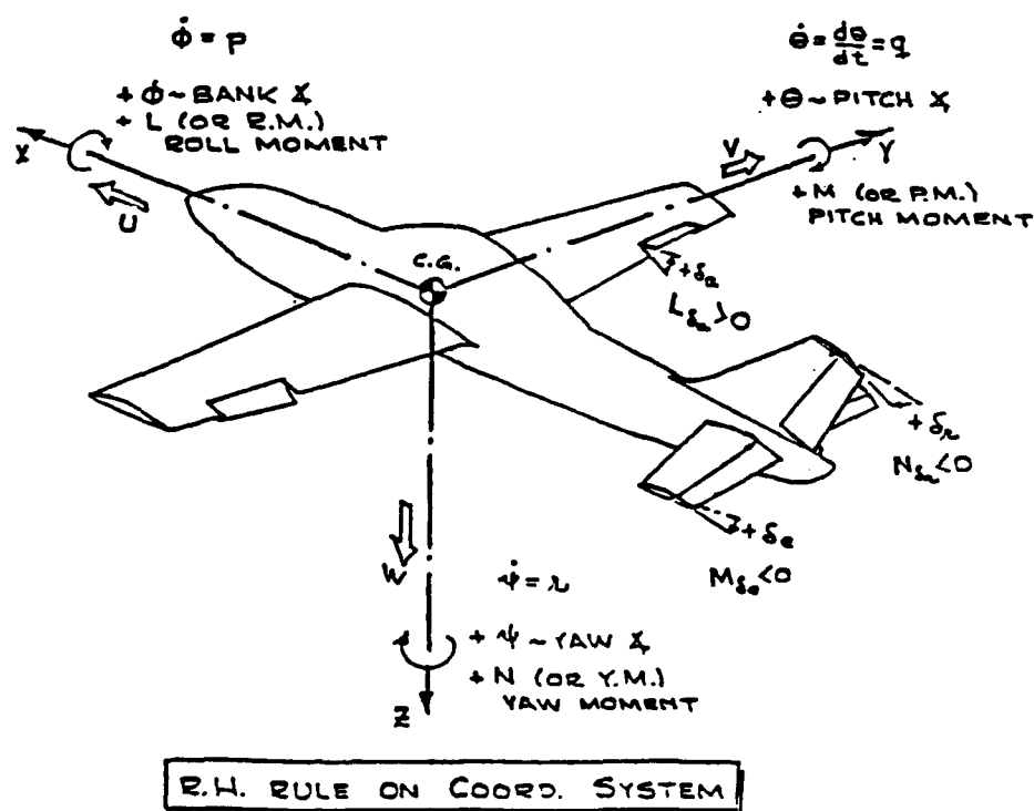
Figure 4.1 Coordinate System
