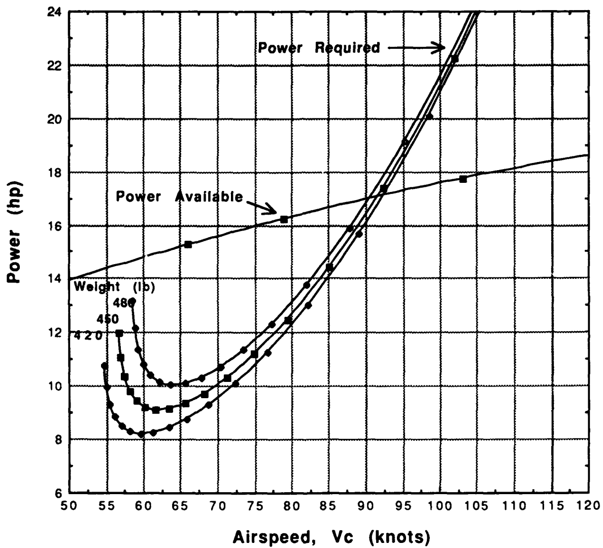
Figure 5.7 Power Curve (5000 Feet)
