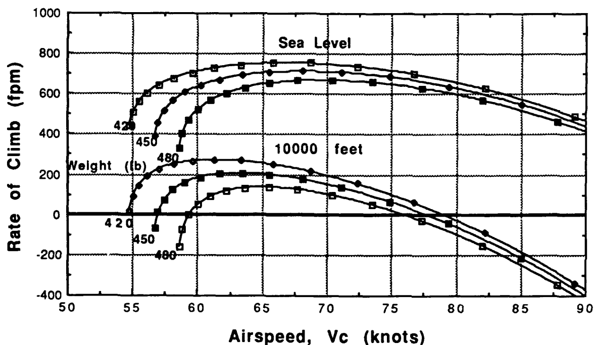
Figure 5.13 Rate of Climb
