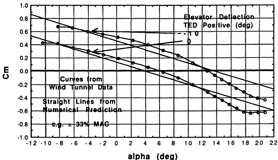
Figure 6.3 Pitching Moment Coefficient Comparison
