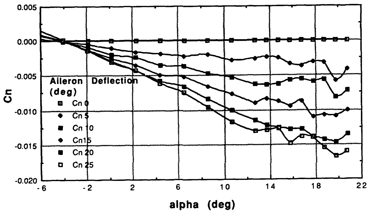
Figure 4.17 Yaw Moment Coefficient due to Aileron Deflection
