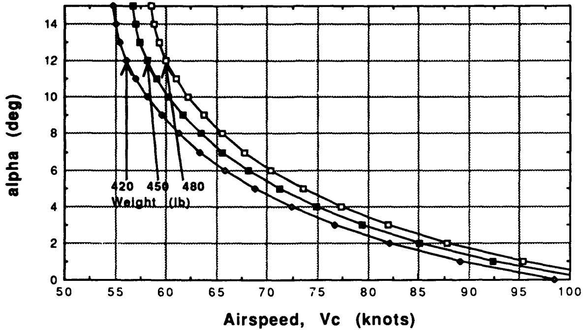
Figure 5.18 Angle of Attack versus Airspeed
