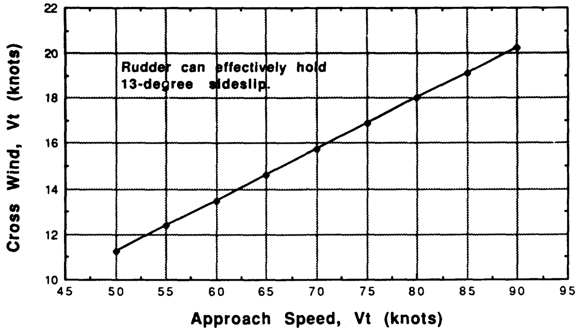
Figure 5.17 Crosswind Limitation versus Approach Speed
