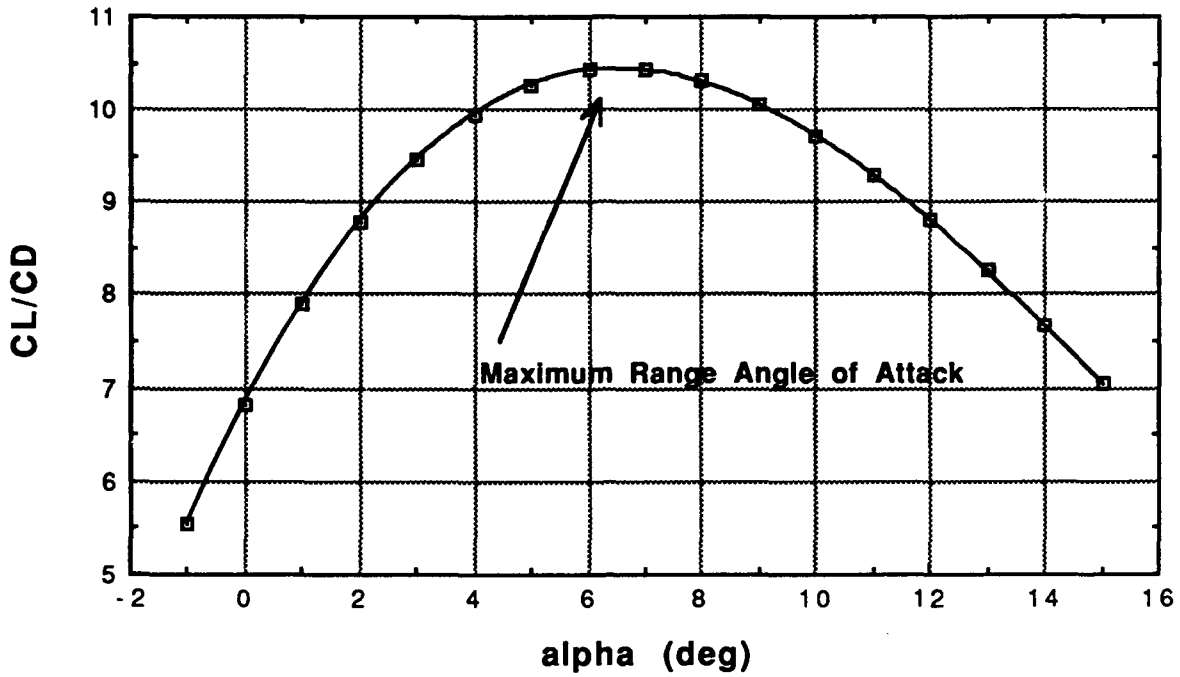
Figure 5.9 CL / CD versus Angle of Attack
