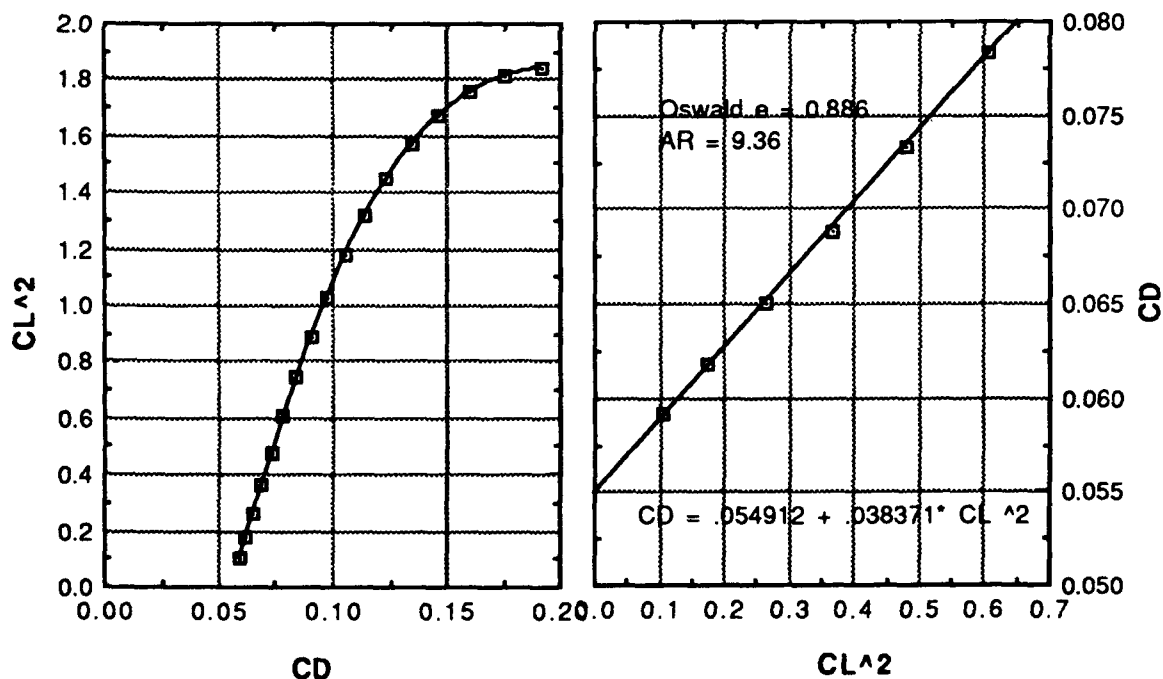
Figure 5.4 C_D versus C_L^2
