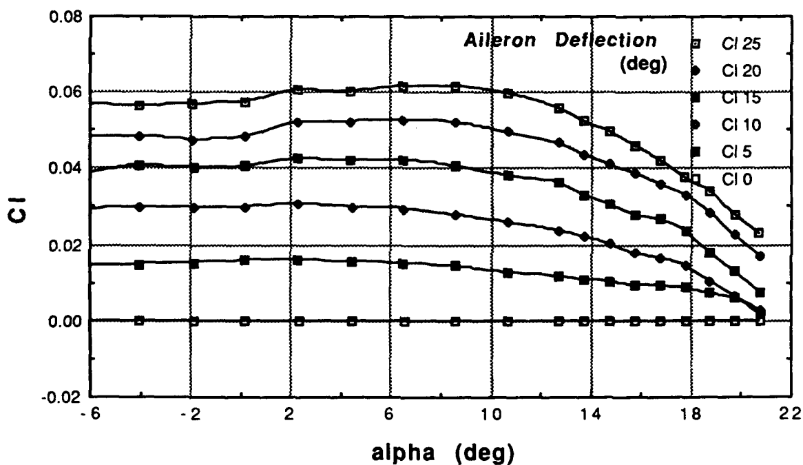
Figure 4.16 Roll Moment Coefficient due to Aileron Deflection
