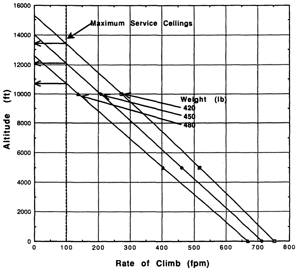
Figure 5.14 Maximum Rate of Climb
