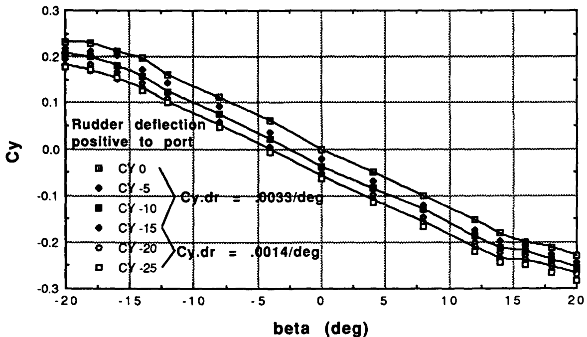
Figure 4.19 Side Force Coefficient at 6^\circ AOA
