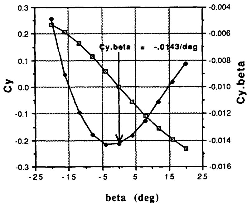
Figure 4.15 Side Force Coefficients at 6° AOA
