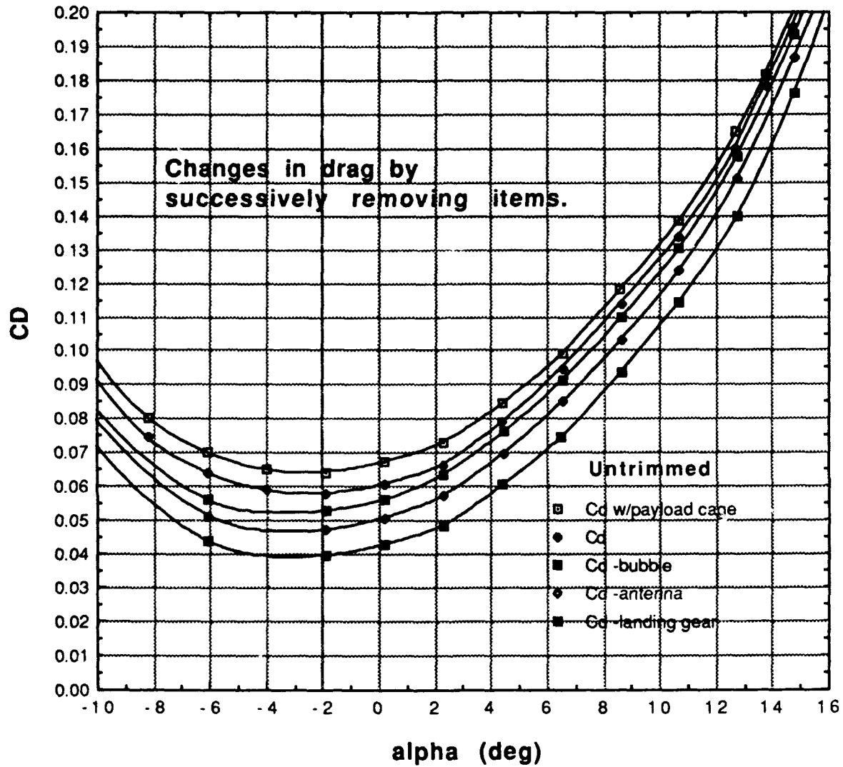
Figure 5.19 Drag Buildup (Untrimmed)
