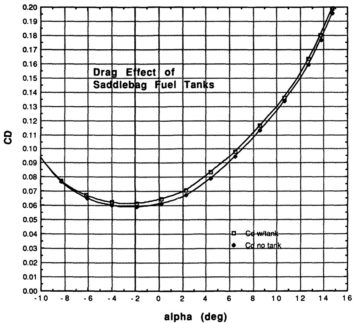
Figure 5.21 Drag Comparison of External Fuel Tank
