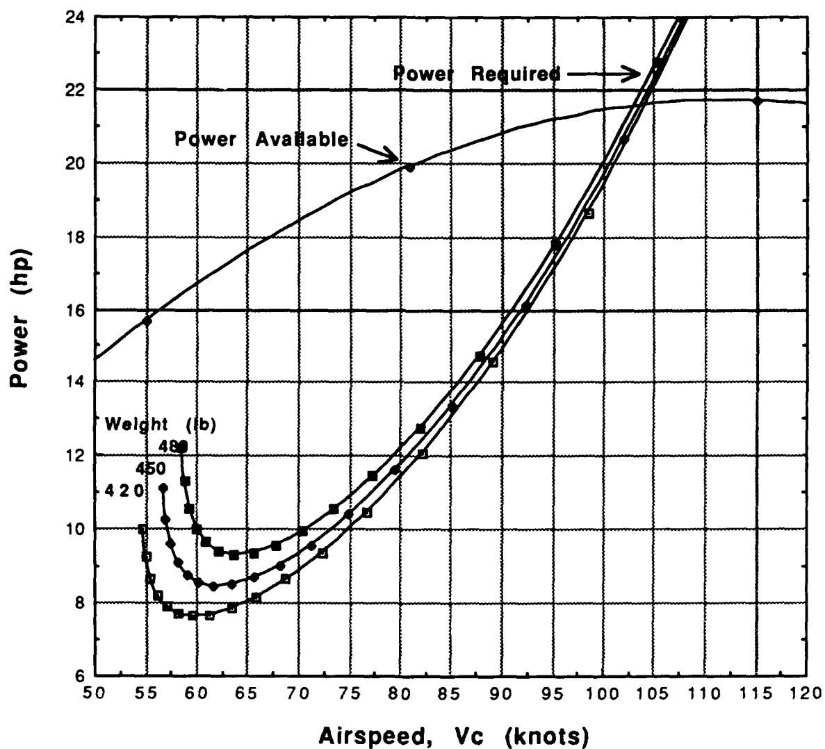
Figure 5.6 Power Curve (Sea Level)
