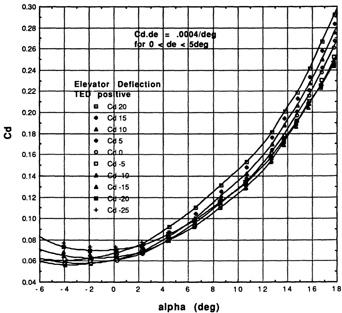
Figure 4.7 Drag Coefficient for Various Elevator Deflections
