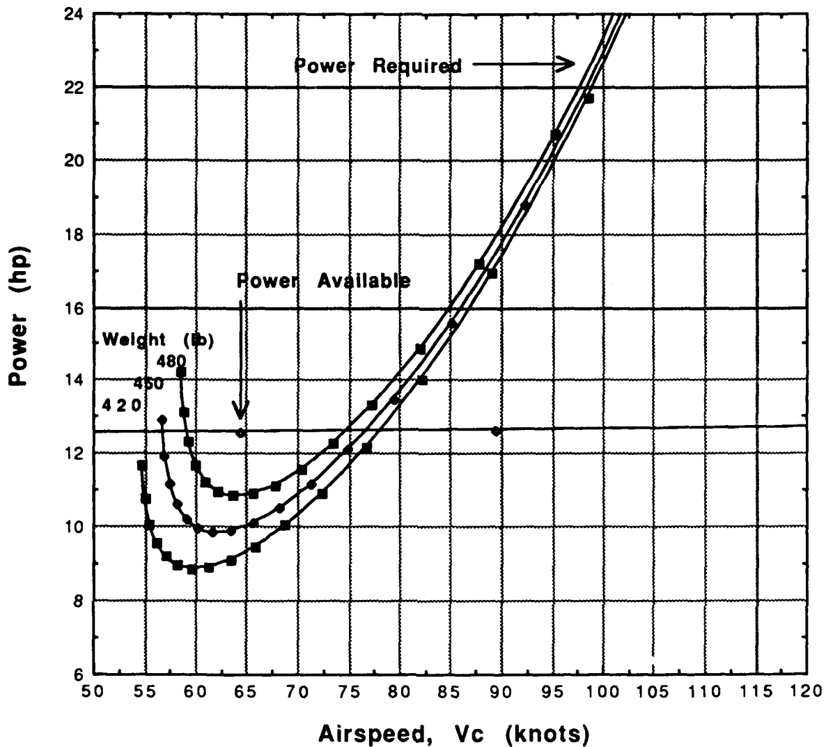
Figure 5.8 Power Curve (10000 Feet)
