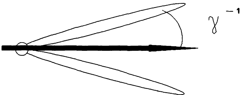
Figure 15: The relationship of the peak cones to \gamma^{-1} .
