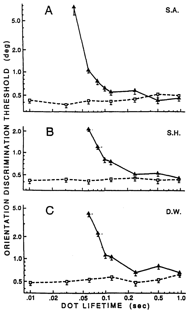
Figure 3. Orientation discrimination threshold (ordinates) versus dot lifetime (abscissae) for a dotted bar defined by relative motion ( \blacktriangle ) and for the same dotted bar defined by luminance contrast ( \square ). The vertical bars mark one standard error. Presentation duration was 1.0 sec throughout. Dot speed was 0.68 deg/sec, so the relative dot speed was 1.4 deg/sec. A, subject 1. B, subject 2. C, subject 3,
