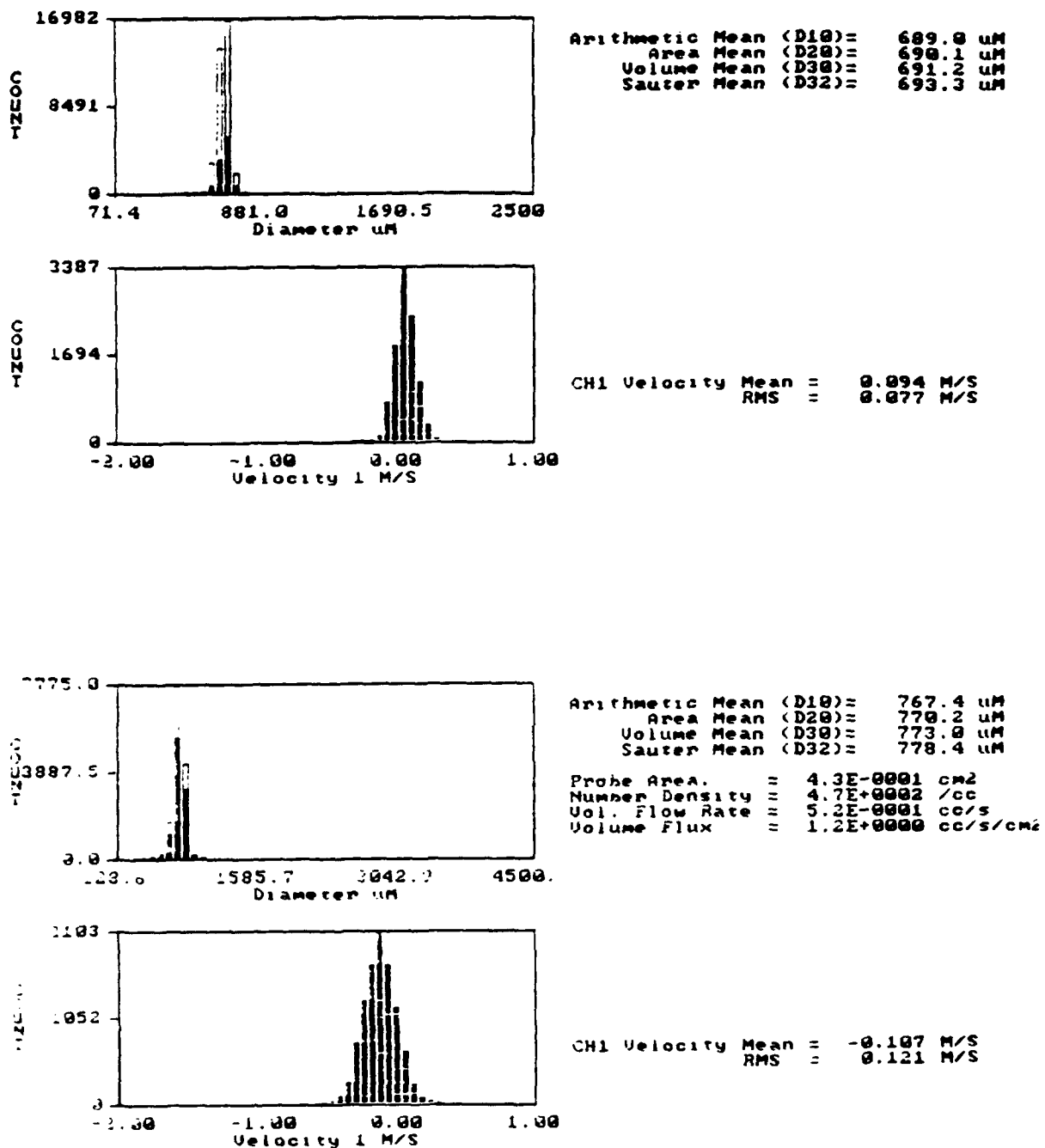
Figure 2.6.22: Results obtained with the PDPA multiangular detection system in the measurement of spherical bubbles. Top: results from the first receiver; bottom: results from the second receiver. Photograph yielded D_{10}=730 \mu\text{m} Void fraction = 0.114.
