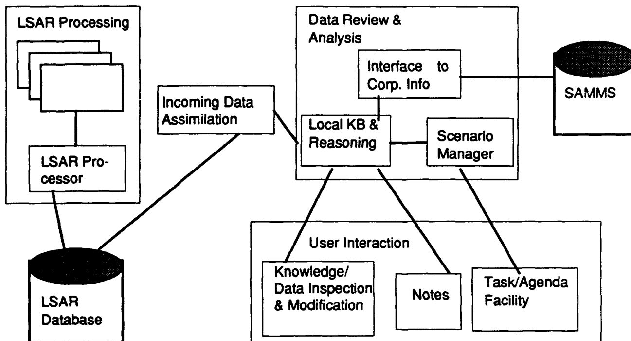
Fig. 1: The DRAMA Architecture
