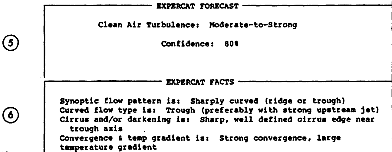
Figure 9. Abbreviated versions of screens used in sample forecast.
