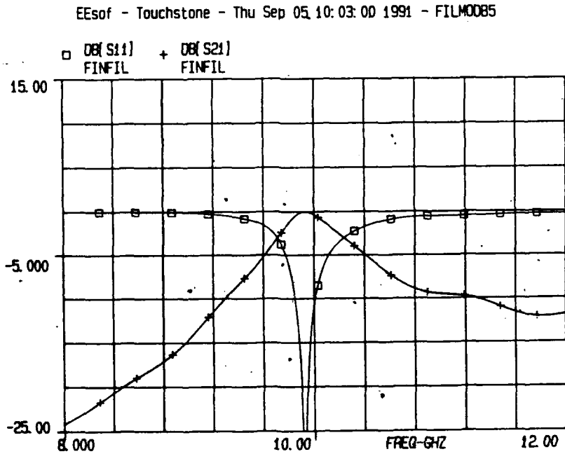
Figure 14. Filter 4 Frequency Response from Model B: W/B = 0.5
