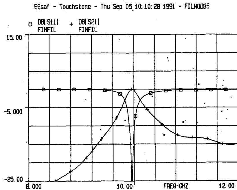
Figure 16. Filter 5 Frequency Response from Model B: W/B=0.5
