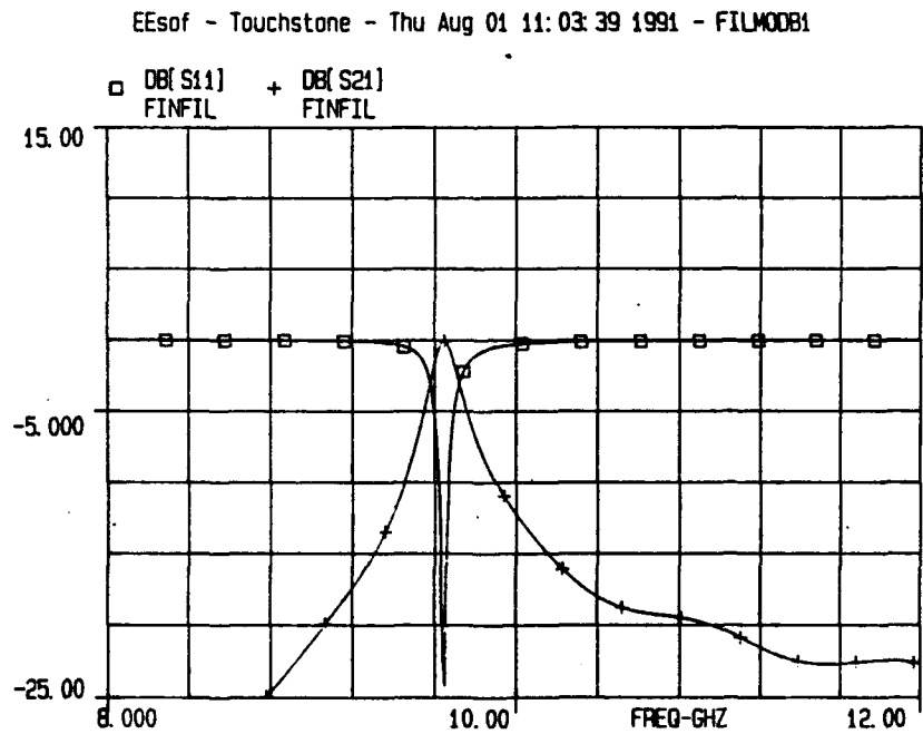
Figure 28. Filter 11 Frequency Response from Model B: W/B=0.1
