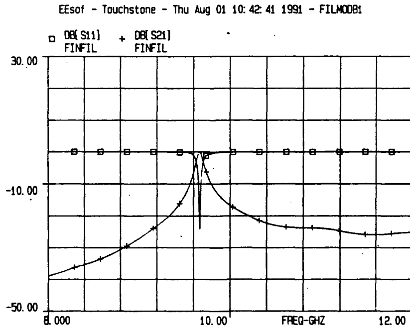
Figure 30. Filter 12 Frequency Response from Model B: W/B=0.1
