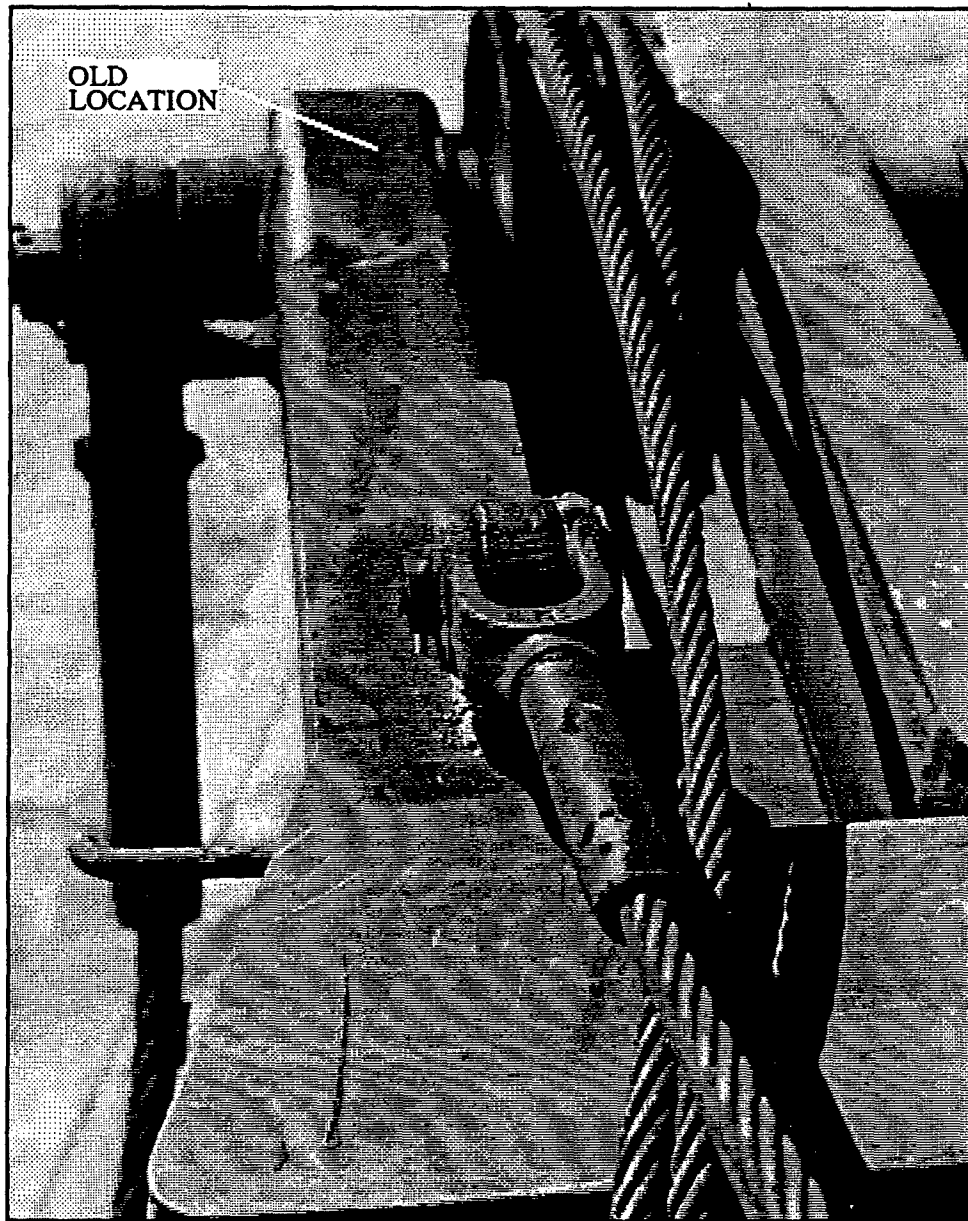
Figure 22 - Relocated Dead-man
