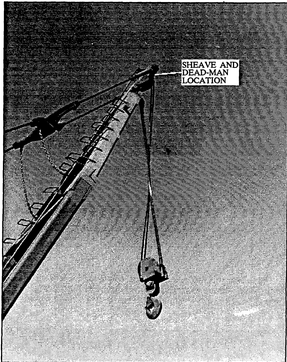
Figure 21 - Cable Twist
