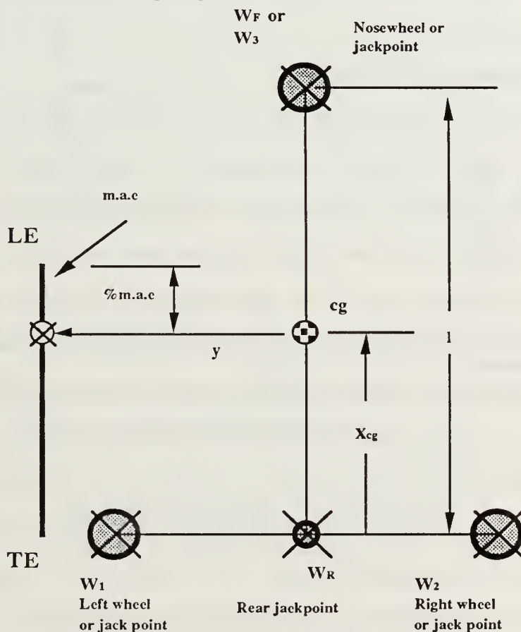
Figure 24 Center of gravity determination.
