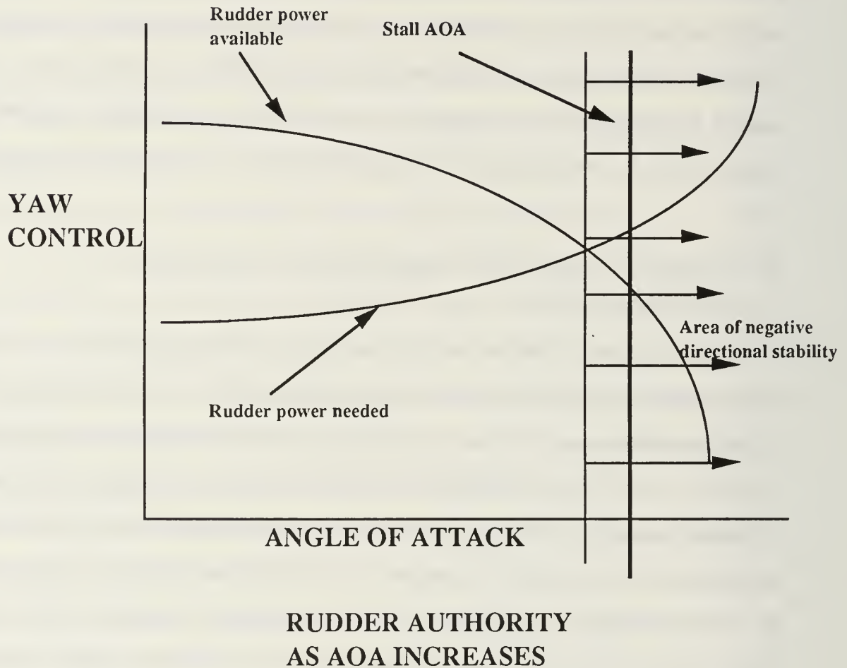
Figure 1 Generic yawing moment versus angle of attack.
