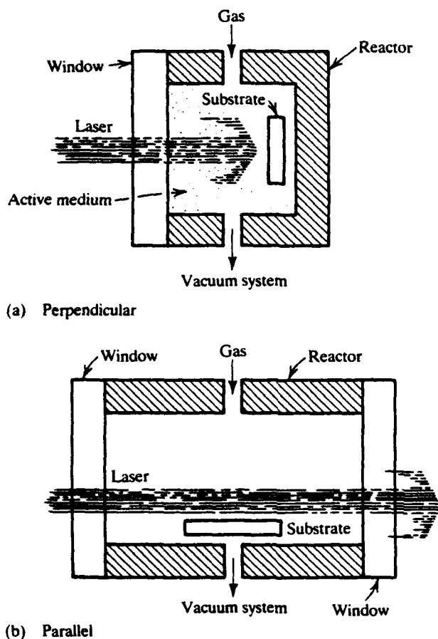
Fig. 3. (a) Perpendicular (or normal incidence) and (b) parallel geometry configurations typically used in laser photodeposition. Because of their lower intensities, ultraviolet lamps can irradiate the substrate (configuration (a)) without inducing a significant rise in surface temperature.
