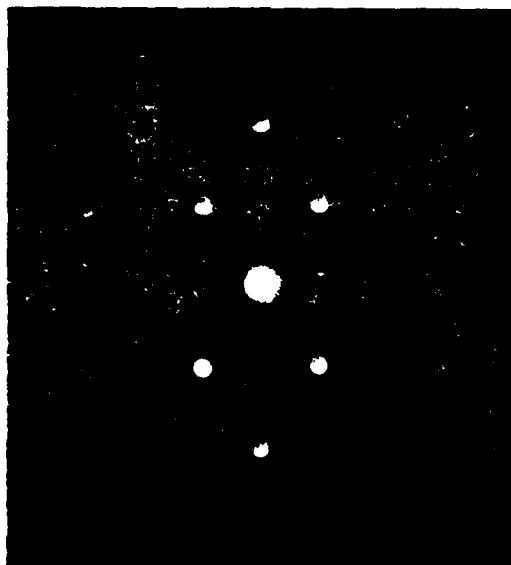
FIG. 14. [0\bar{1}1] convergent beam electron diffraction pattern of the \sim 800\text{-\AA} -thick epitaxial Ge film for the sample of Figs. 12 and 13.
