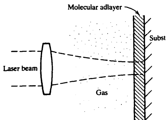
Fig. 1. Diagram illustrating the three media—gas, adlayer, and substrate—that are generally present in a photodeposition reactor. The optical and chemical properties of these three play a key role in determining the nature of the reactions that culminate in film growth and in the metallurgical and electrical properties of the deposit. Although the laser is shown irradiating the substrate, films are often grown with the optical beam directed parallel to the surface (adapted from Ref. 14).
