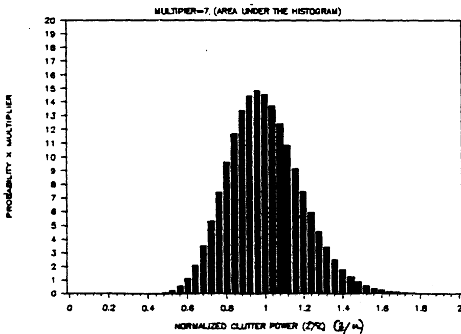
(b) GAMMA DENSITY (SHAPE FACTOR(K)=27.5)
