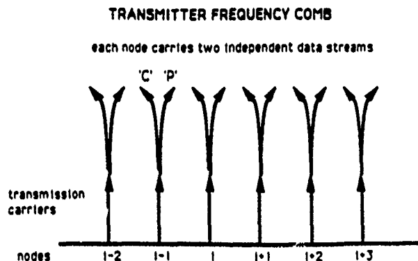
Figure 2: The node transmitter must be capable of multiplexing two independent data streams onto the same lightwave carrier.
