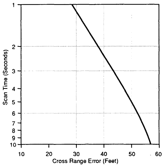
Figure 11. Cross-Range Error versus Scan Time
