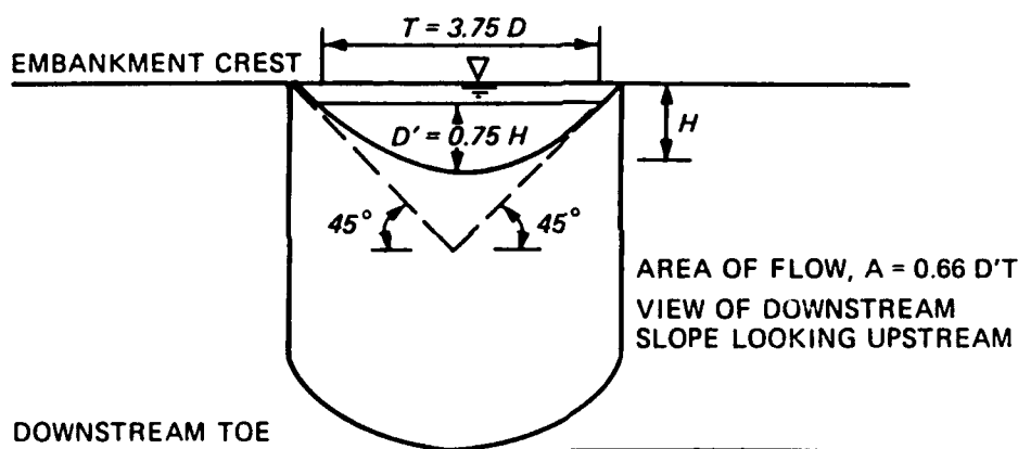
Figure 23. Breach configuration for Harris and Wagner hypothesis
