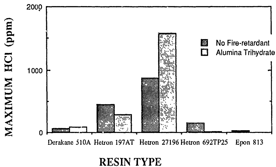
Figure 9. Effect of Added Fire Retardant on the Concentration of HCl_{max} (ppm).
