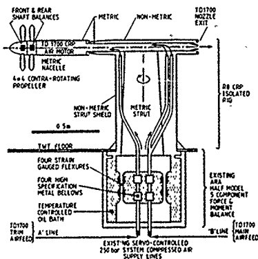
FIG 42(a) AIR-DRIVEN SMALL PROPELLER R/C IN ARA TRANSONIC TUNNEL (FROM REF.105)
