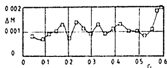
Typical Mach number deviations during a polar
