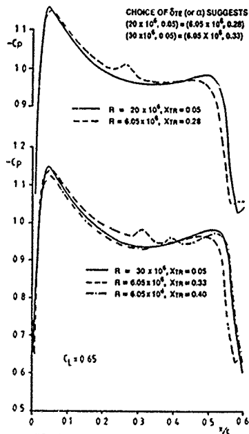
FIG 36c APPLICABILITY OF \delta_{TE} CRITERION C_L = 0.65
