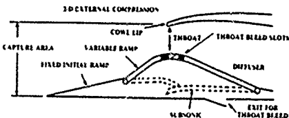
Fig. 32 Variable inlet geometry
