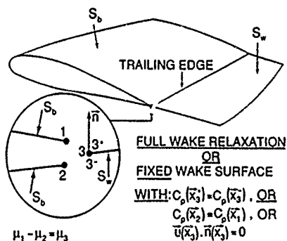
Fig. 3.14 Kutta conditions
