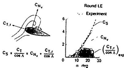
Fig. 30 Relationship between vortex normal force and residual thrust, A = 1.0 , \Delta = 76^\circ , t/c = 0.1 , FFA 104-5601 airfoil
