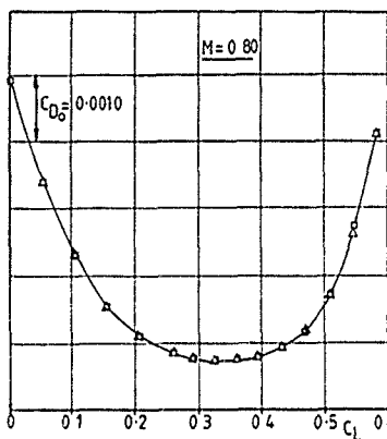
FIG 1 REPEATABILITY STANDARD WITHIN A GIVEN TEST (ARA TRANSONIC TUNNEL, FROM REF 15)
