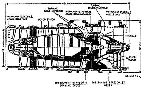
FIG 52 CROSS-SECTIONAL VIEW OF CHAPS (FROM REF. 133)
