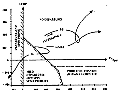
Fig. 23 Departure susceptibility.
