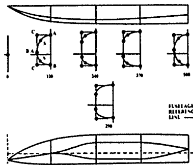
Fig. 47 Typical fuselage lofting
