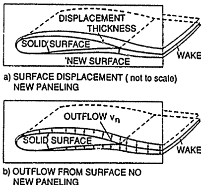
Fig. 8.3 Simulation of boundary-layer effects
