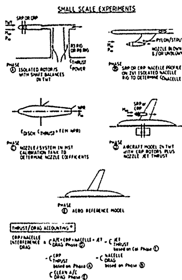
FIG 42(d) TYPICAL MODEL TEST PROGRAMME FOR TURBOPROP PROPELLER PERFORMANCE (FROM REF.105)
