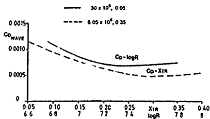
FIG 36(d) CONSEQUENCE OF FAILURE TO SIMULATE SUPERCritical FLOW DEVELOPMENT (FROM REF. 86)
