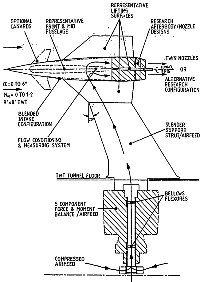
FIG 49 NEW RIG FOR AFTERBODY PERFORMANCE TESTING
