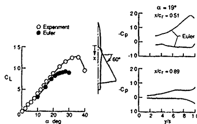
Fig. 41. Euler solution, F-106B, M \approx 0.3
