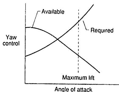
Fig 76 Typical yaw control requirements for maneuvering
