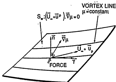
Fig. 3.13 Partial wake relaxation - Force on wake
