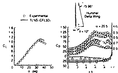
Fig. 43 Thin layer N-S solution, A = 1 \delta , M \approx 0 , R_nu = 0.95 \times 10^6
