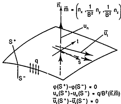
SOURCE DISTRIBUTION
