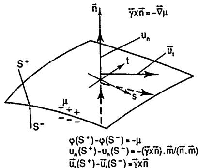
DOUBLET DISTRIBUTION
