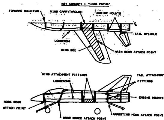
Fig. 26 Structural arrangement.
