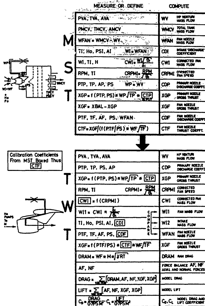
FIG 39 BOOKKEEPING PROCEDURE (FROM REF.9)
