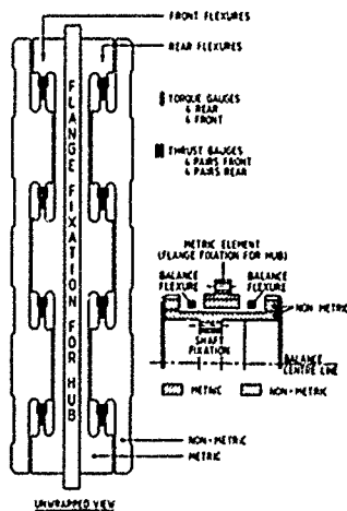
FIG 42(c) BALANCE DESIGN FOR CONTRA-ROTATING PROPELLER
