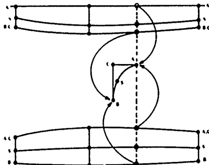
Fig. 46 Cross section development from longitudinal control lines
