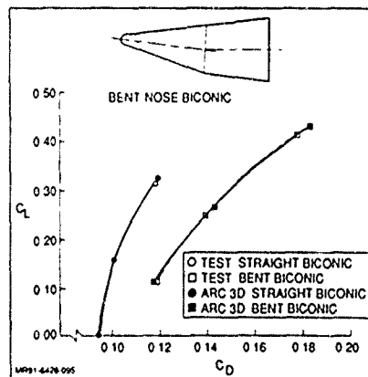
Fig. 87 Straight &amp; Bent Biconic Drag Polar at Mach 6.0
