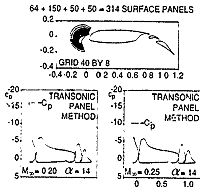
Fig. 9.1 Application of field panel method to 4-component airfoil section (Ref. 41)
