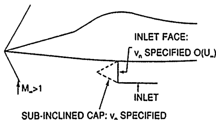
Fig. 3.15 Inlet modeling in supersonic flow
