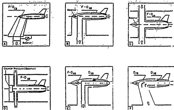
FIG 51 A' (ERBODY TEST RIGS (FROM REF. 12))
