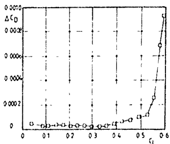
Errors in C_D due to Mach number deviations
