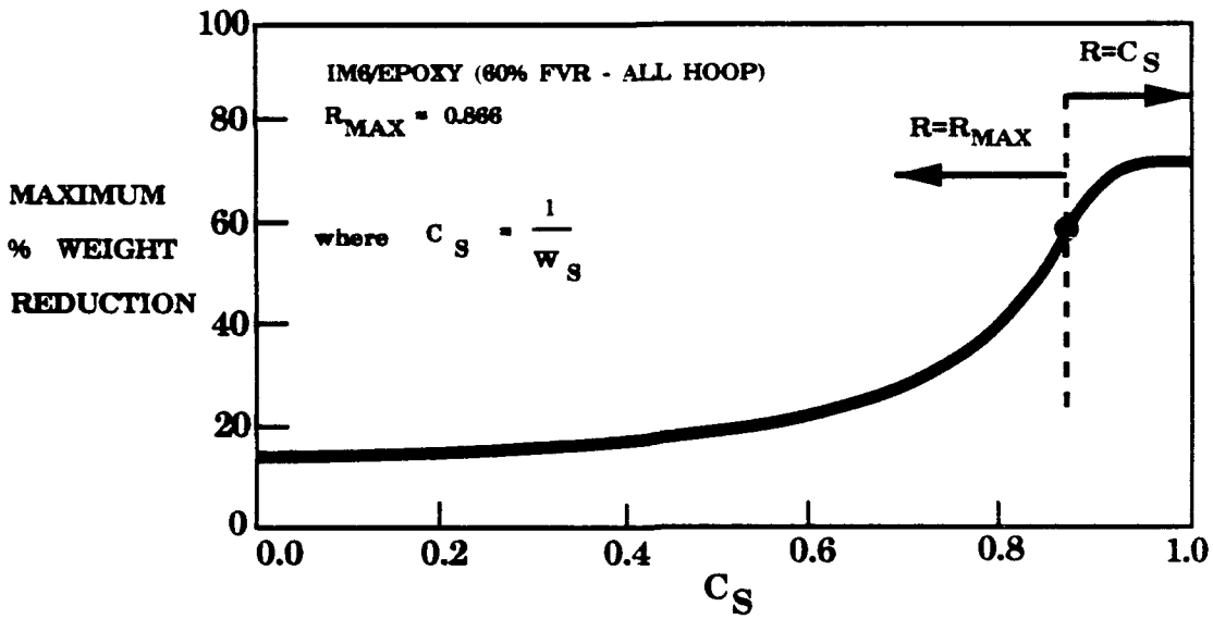
Figure 2. M%WR as a function of C_S for equivalent compound cylinders using IM6/epoxy to replace material from the outer diameter of a steel IMC.
