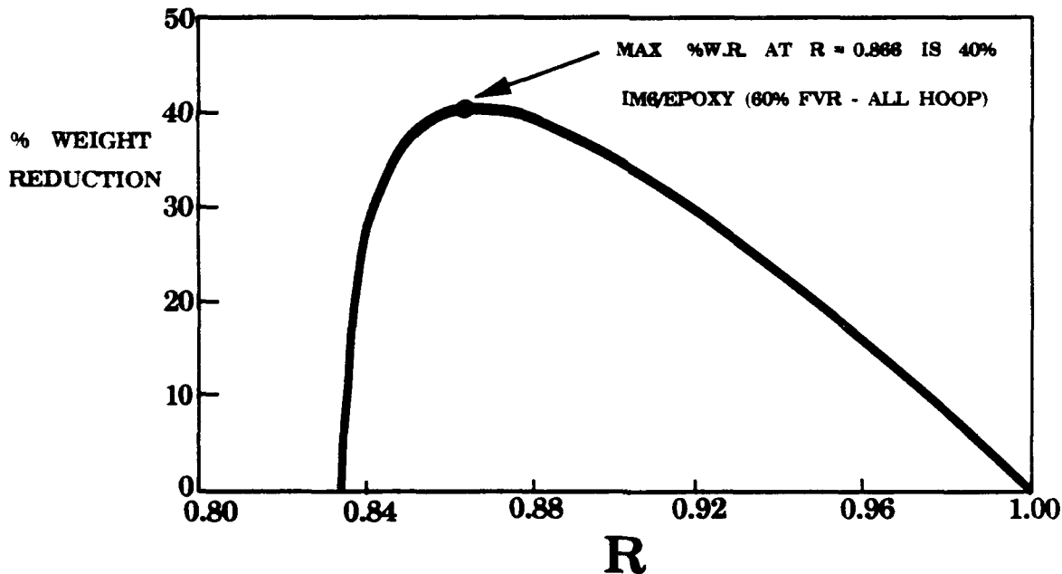
Figure 1. %WR versus R for equivalent compound cylinders using IM6/epoxy to replace material at the outer diameter of steel IMC with W_s = 1.255 .
