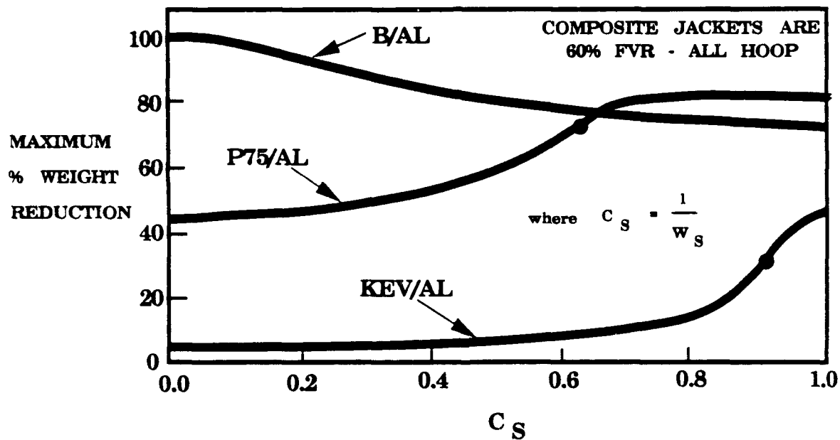
Figure 3. M%WR as a function of C_s for equivalent compound cylinders using three composite materials to replace material at the outer diameter of a steel IMC.
