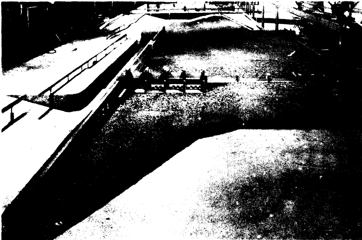
Figure 2. 1:40-scale model of original design looking downstream
