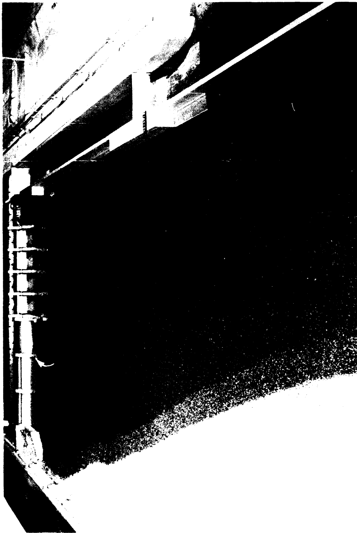
Photo 1. One hinge gate open; pool el 122; tailwater el 95; with the 69-ft separation
