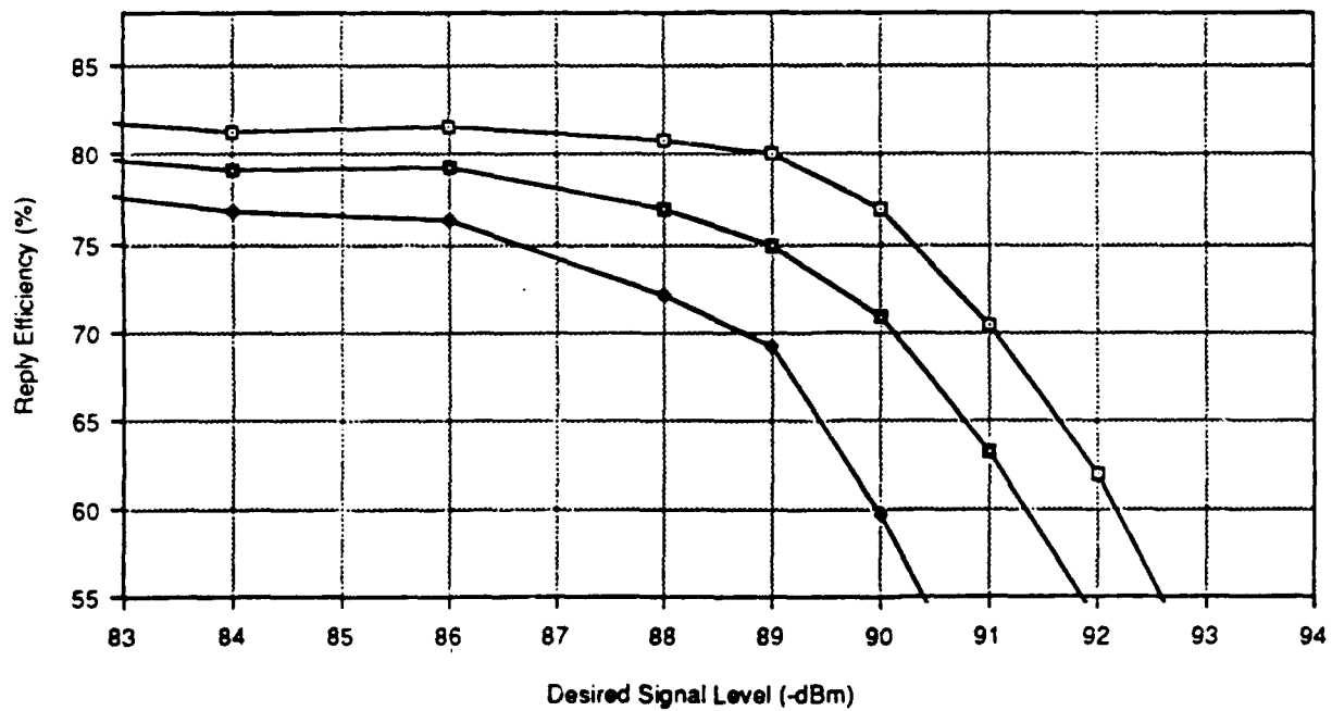
Figure 6-6. AN/TRN-41 TACAN Beacon Test Results, Osan AB, Korea, Channel 96X. JTIDS 1000 watts, TSDF Varied. Received JTIDS Signal Level at -34 dBm.
