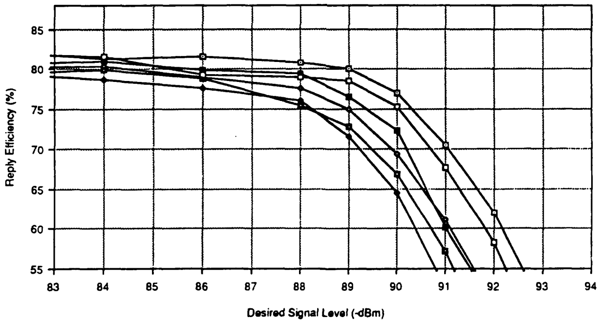
Figure 6-4. AN/TRN-41 TACAN Beacon Test Results, Osan AB, Korea, Channel 96X. JTIDS 200 watts, TSDF Varied. Received JTIDS Signal Level -40 dBm.
