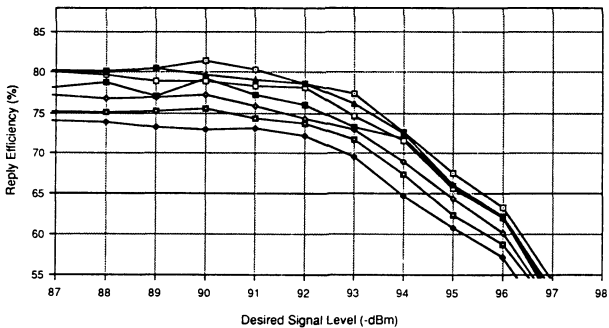
Figure 6-2. AN/GRN-20B TACAN Beacon Test Results, Osan AB Korea, Channel 94X. JTIDS TSDF 50 percent at 200 watts. Received JTIDS Signal Level Varied.
