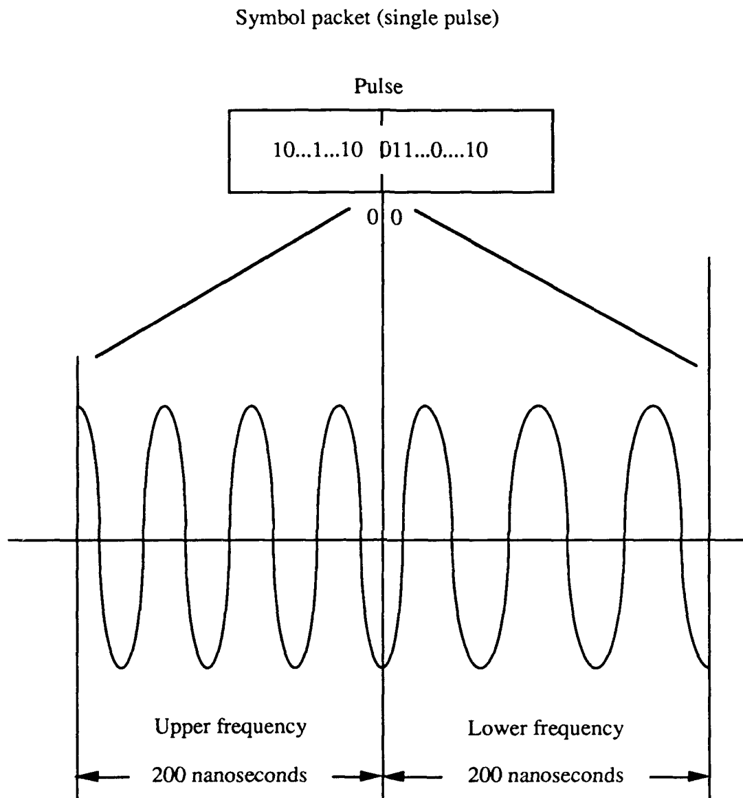
Figure 2-2. JTIDS Pulse Structure
