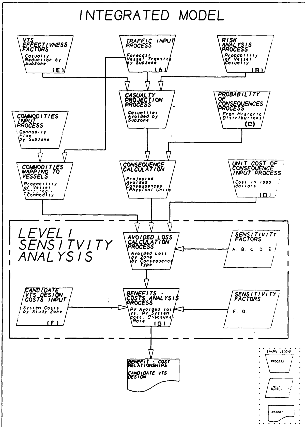
FIGURE 8-2. SENSITIVITY ANALYSIS
