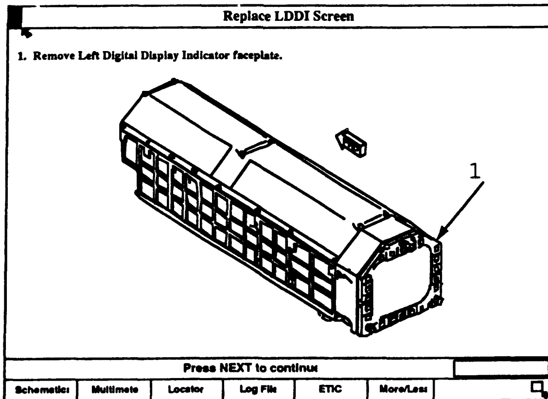
Figure 12. Procedural Screen.
