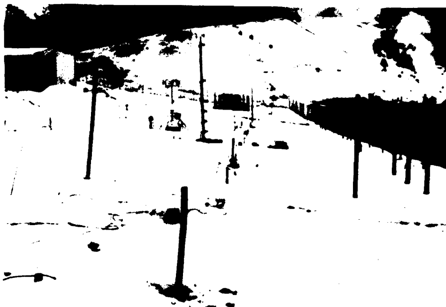
Figure 5. View of the sensor array looking south (i.e., towards the acoustic source). In the foreground, a vertical component geophone 90 m away from the source is visible. The snow platform, with microphone, power supply and vertical component geophone, is visible along with the geophone installed in undisturbed snow to the right. The large tower is 60 m from the source. A portion of the FERF, with garage door, is visible to the left. This building, and others in the vicinity, cause acoustic reflections to appear on the recorded signals.
