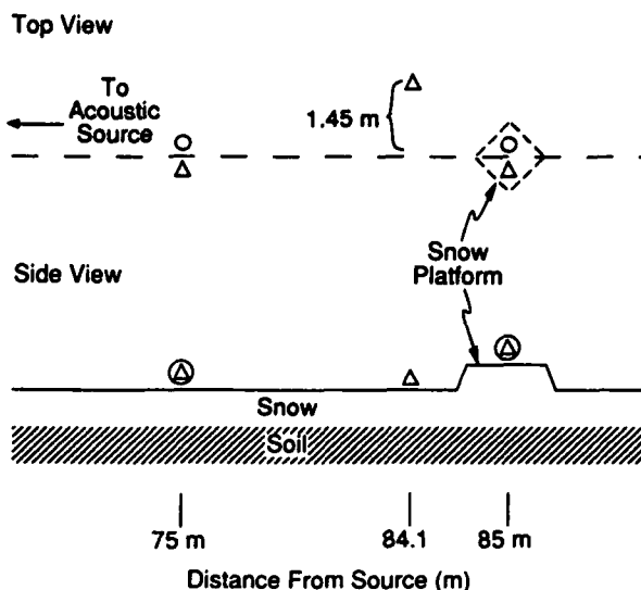
Figure 2. Schematic view (not to scale; circles denote microphones, triangles denote geophones) of the sensors used to record the data. (Top) plan view of the sensor layout; (bottom) cross-sectional view.
