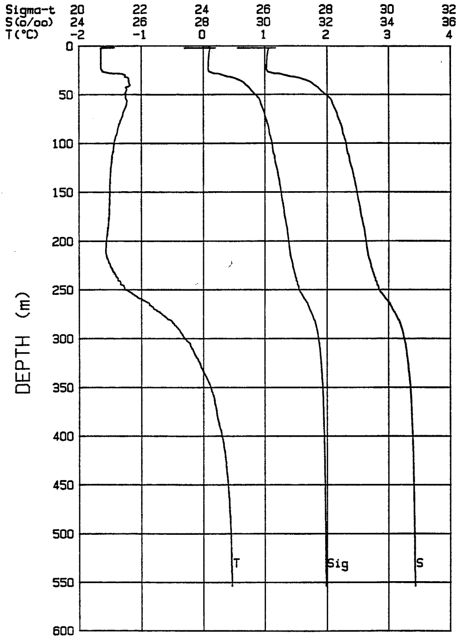
Figure 7. STD profile.
