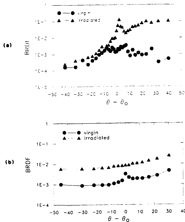
FIGURE A-4. BRDF OF MARTIN BLACK BEFORE AND AFTER 0.6 cal/cm 2 ELECTRON IRRADIATION. a) Measurement was made on the BRO FASCAT instrument at a wavelength of 10.6 microns. b) Measurement was made on the BRO FASCAT instrument at a wavelength of 633 nm.
