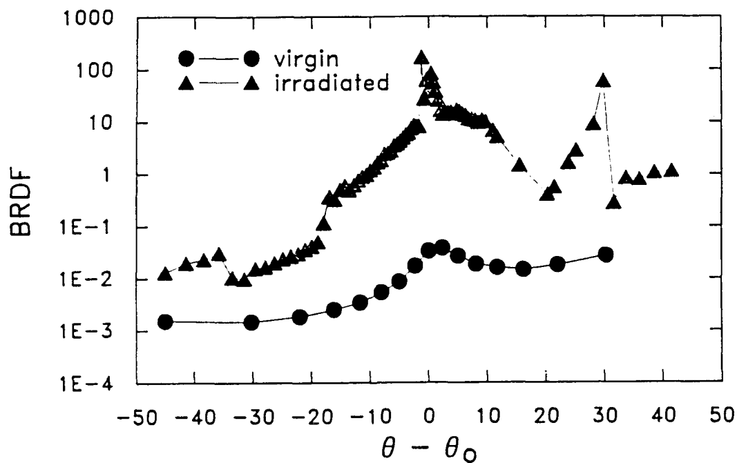
FIGURE A-5. BRDF OF BALL BLACK BEFORE AND AFTER 0.6 cal/cm 2 ELECTRON IRRADIATION. Measurement was made on the BRO FASCAT instrument at a wavelength of 633 nm.
