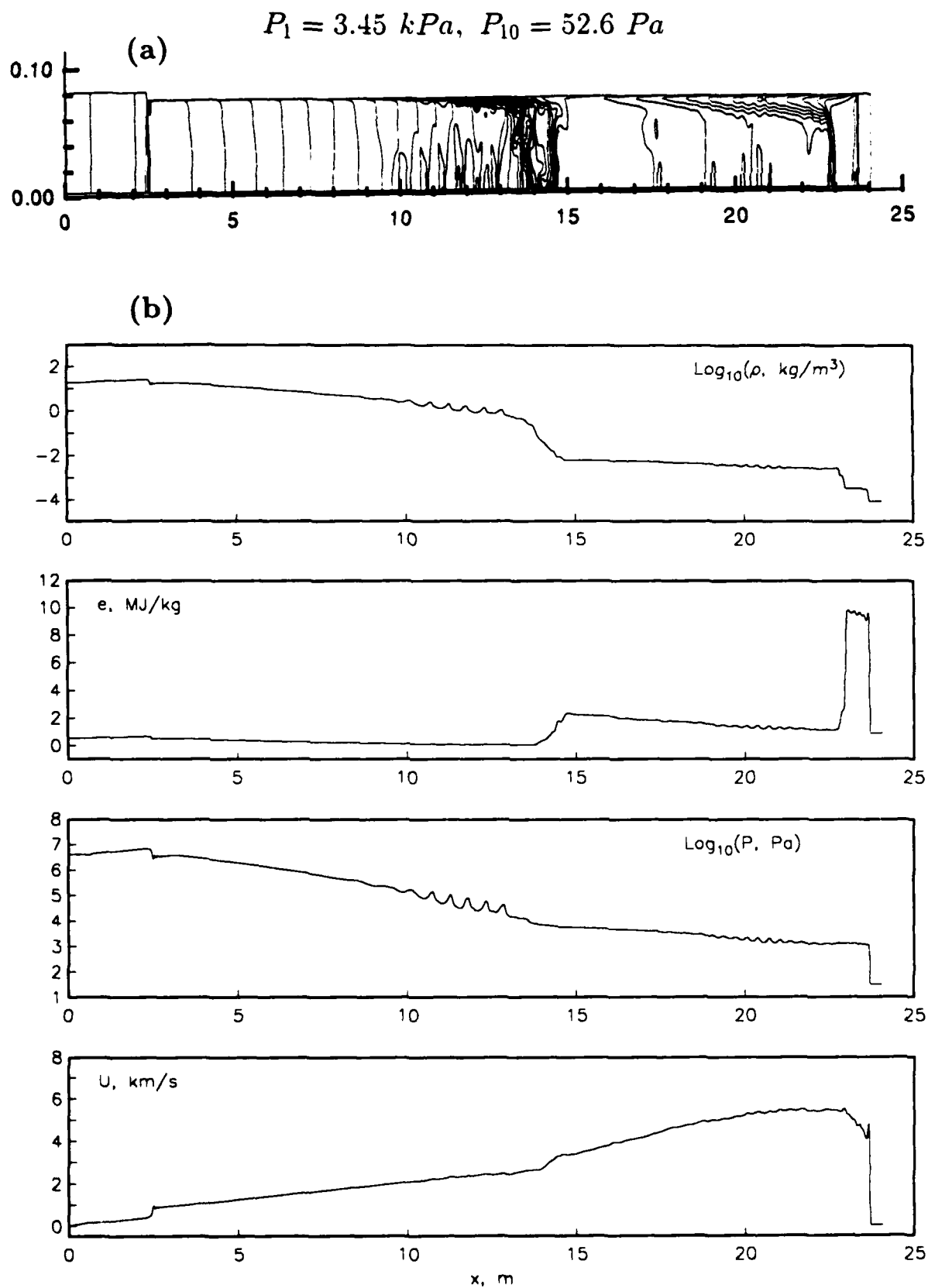
Figure 30: Properties along the axis at t = 4.5 \text{ ms} for case 4: (a) density contours; (b) other properties as labelled.
