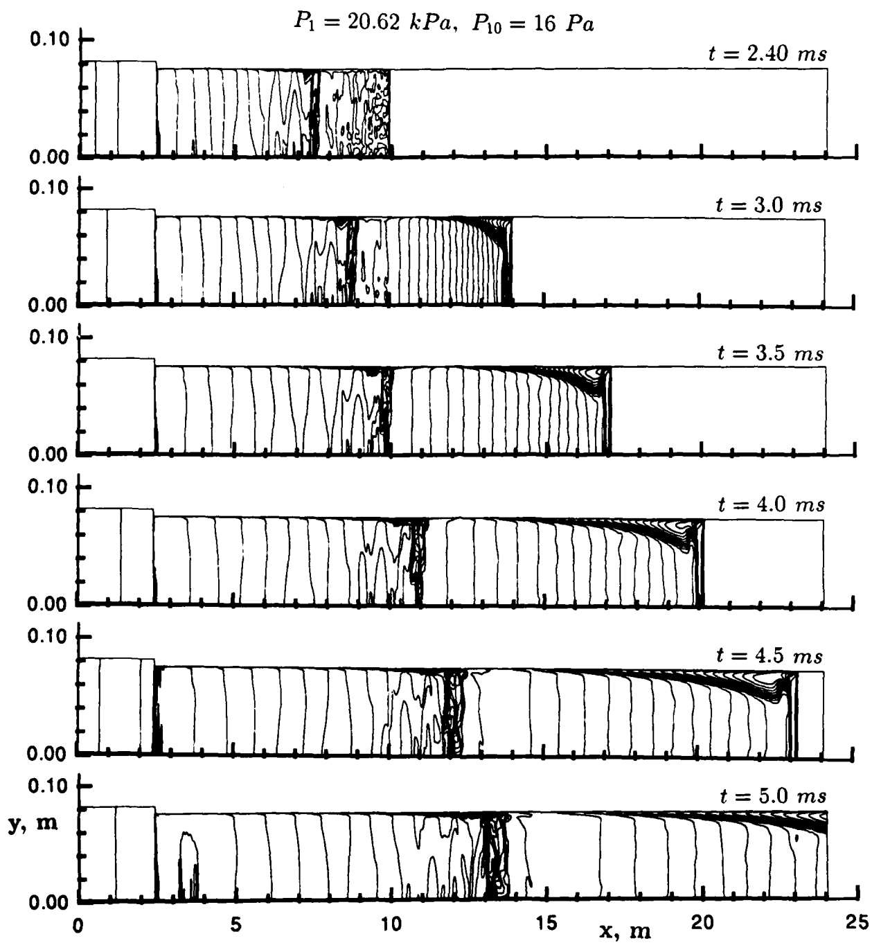
Figure 18: Density contours showing the unsteady expansion of the test gas for case 2.
