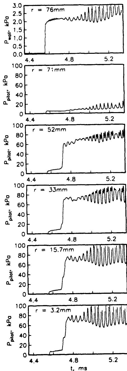
Figure 32: Comparison of wall pressure and pitot pressure with experiment (case 4, x = 24 \text{ m} ). The experimental data is taken from Shinn and Miller (1978).
