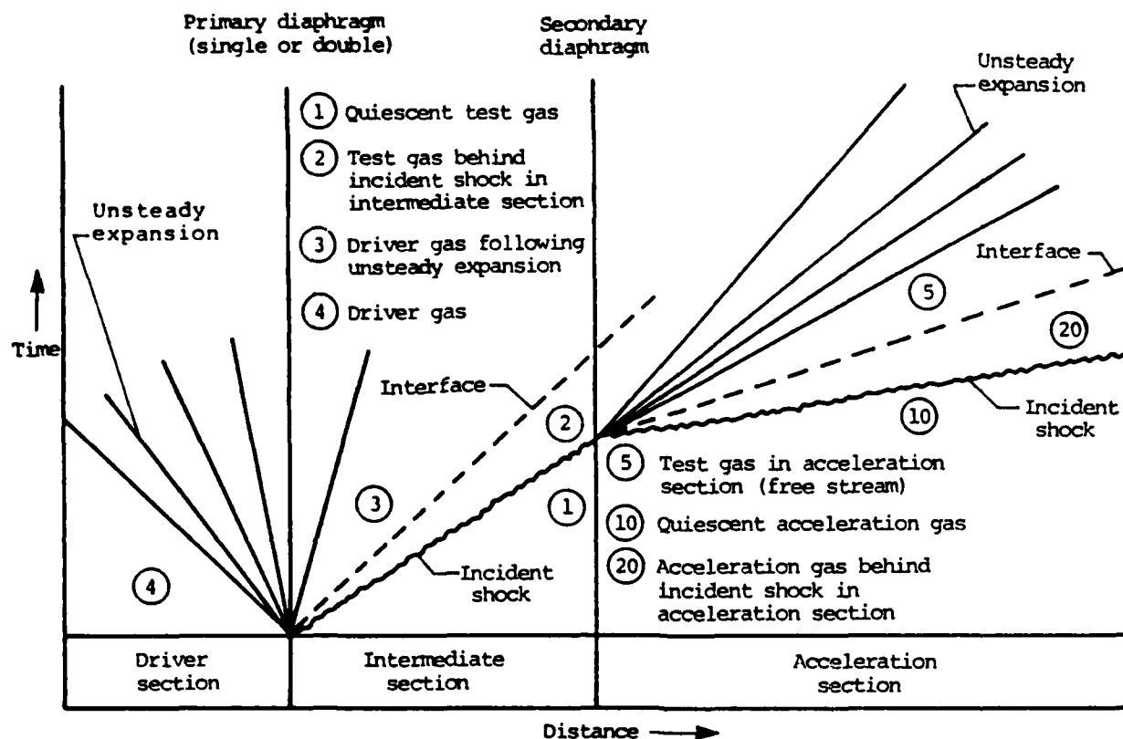
Figure 1: Conceptual wave diagram for the operation of the NASA Langley expansion tube. The numbers refer to the states of the gases as defined by Trimpi (1962).
