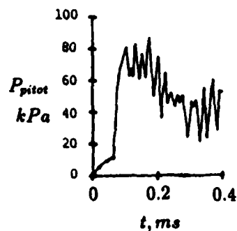
Figure 32: Comparison of wall pressure and pitot pressure with experiment (case 4, x = 24 \text{ m} ). The experimental data is taken from Shinn and Miller (1978).
