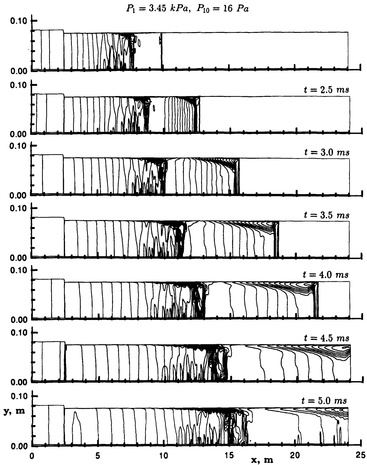
Figure 35: Density contours showing the unsteady expansion of the test gas for case 1a.
