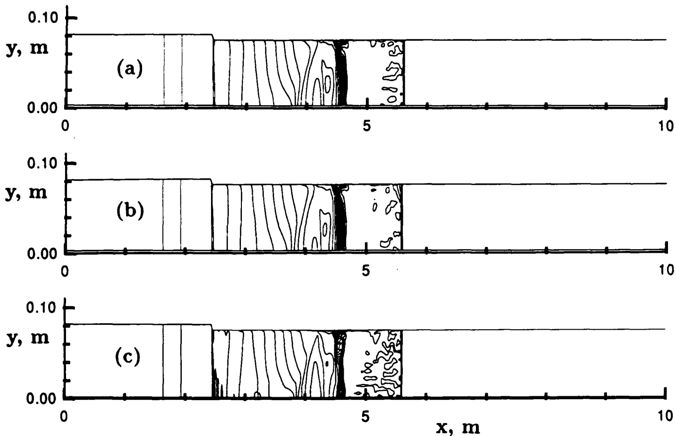
Figure 3: Comparison of the density fields at t = 2.0 ms for case 2: (a) 1604 \times 20 grid, Euler time-stepping; (b) 1604 \times 20 grid, predictor-corrector time-stepping; (c) 2406 \times 30 grid, Euler time-stepping.
