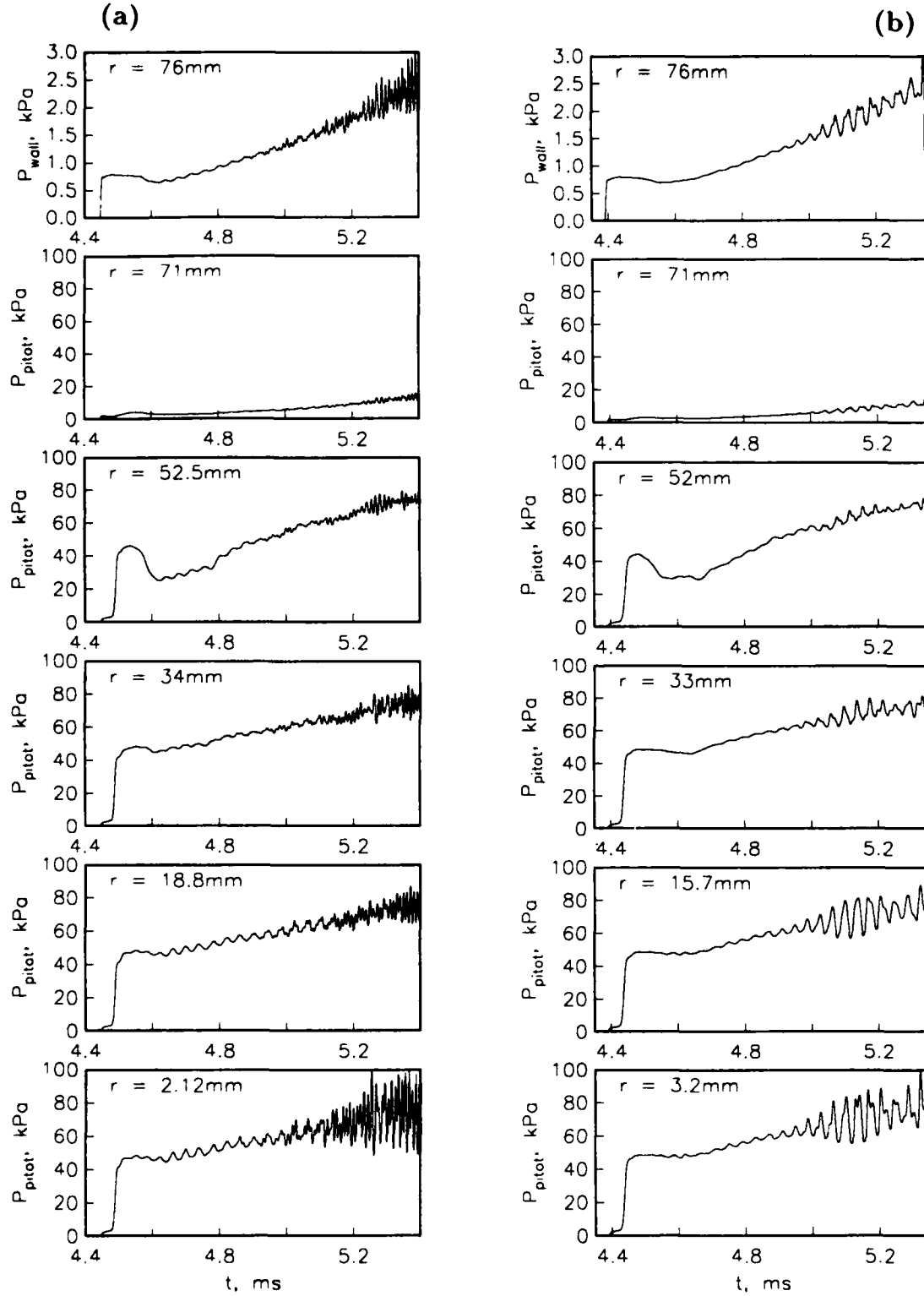
Figure 37: Comparison of Pitot histories at x = 24 \text{ m} for (a) 2406 \times 30 grid and (b) 1604 \times 20 grid.
