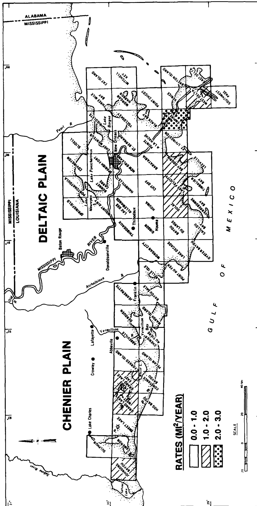
Figure 2c. Summary of land loss rates in square miles per year for time period 3 (1974 to 1983)
