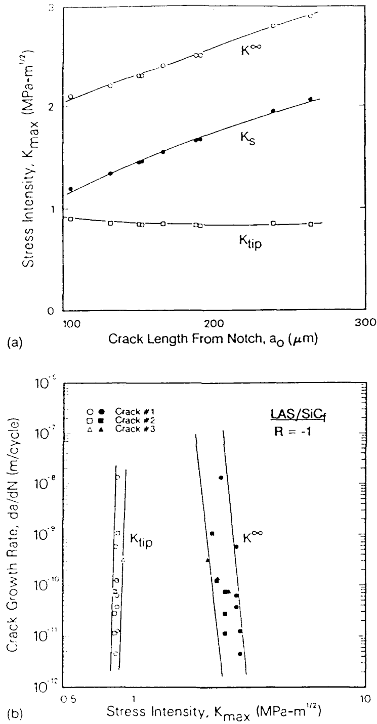
Fig. 4.8. (a) Predicted variation in shielding stress intensity, K_s , due to crack bridging (Eq. 3a), and effective (near-tip) stress intensity, K_{\text{tip}} , with measured crack size from notch, over the range of nominal stress intensities, K_{\infty} , utilized in the experiments. (b) Corresponding plot of the short-crack growth rate data for LAS/SiC f from Fig. 4.7 with K_{\text{tip}} , showing the expected positive power-law dependency of growth rates on stress intensity.
