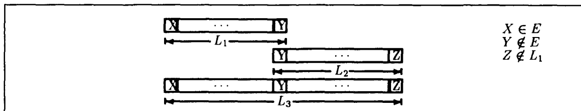
Figure 16. General Application of the join Function.
