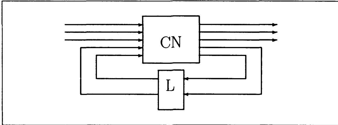
Figure 14. Huffman Model.
