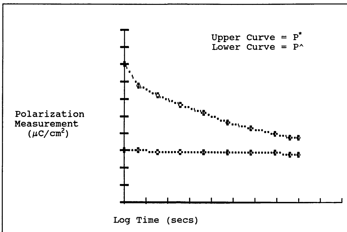
Figure 17. DP is the Difference Between P^* and P^
