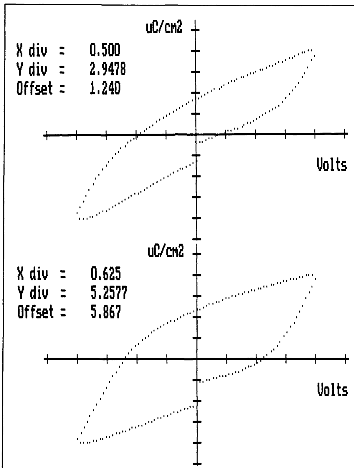
Figure 51. Hysteresis Loops for Sample 0/20/80 Pt/Pd, Applied Voltage Equal ( V_{57\%} , V_{71\%} )
