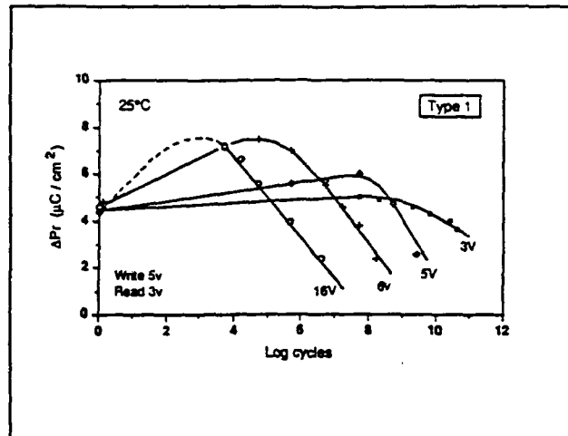
Figure 8. "Fatigue: effect of cycling voltage" (52:281)
