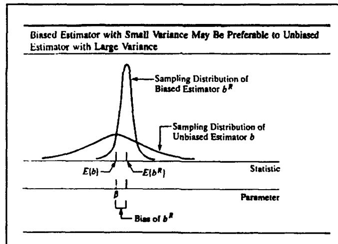
Figure 22. Tradeoff Between Bias and Variance (13:412)
