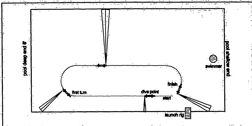
Figure 6.11 NPS AUV test track using left transducer only. Note swimmer target.
