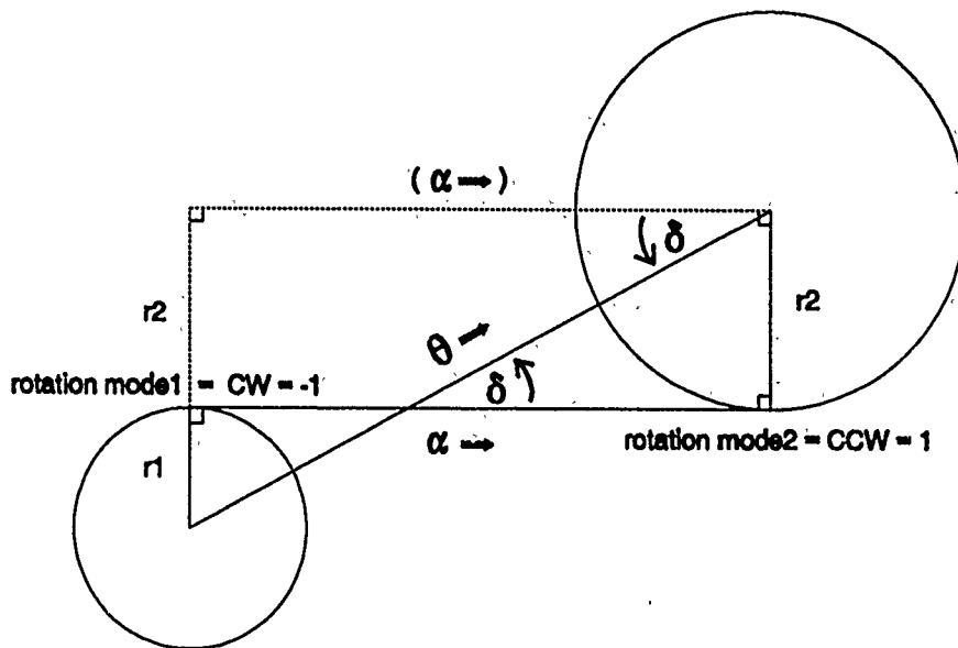
Figure 7.6 Determination of circle cross-tangents and external tangents
