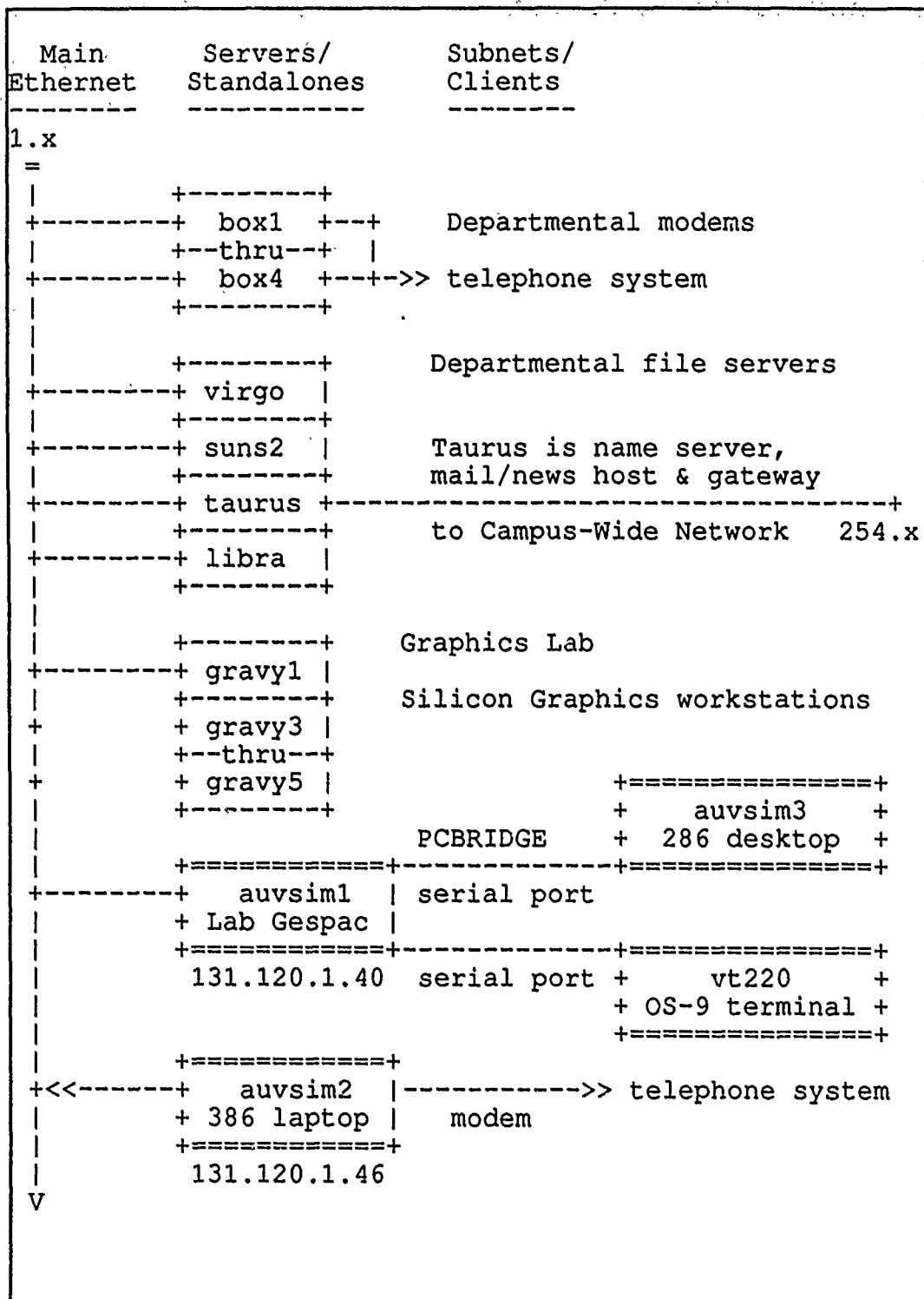
Figure 5.2 NPS Computer Science Department Network portion of NPS AUV Integrated Simulator data network (part 1)
