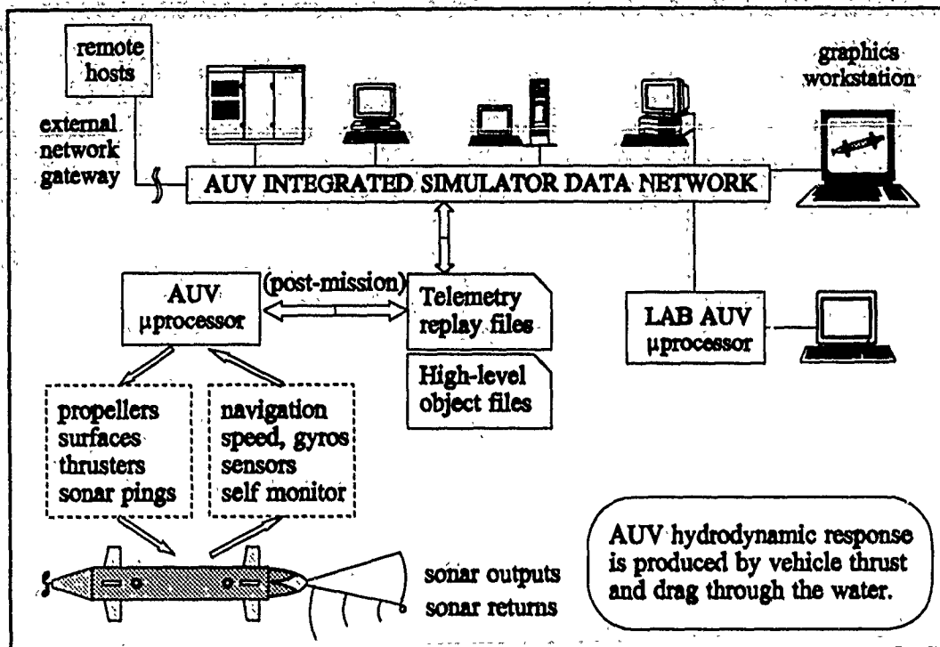
Figure 3.1 Integrated simulator network physical connectivity
