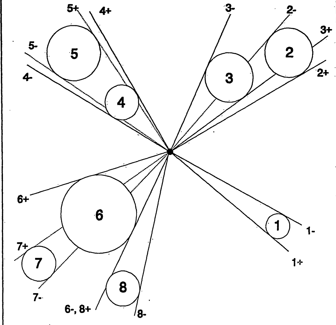
Figure 7.9 Sweep visibility determination from point to all circles
