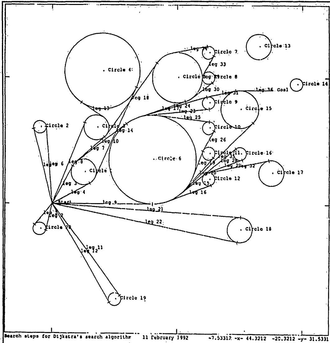
Figure 7.15 Search steps displayed for Dijkstra's search algorithm
