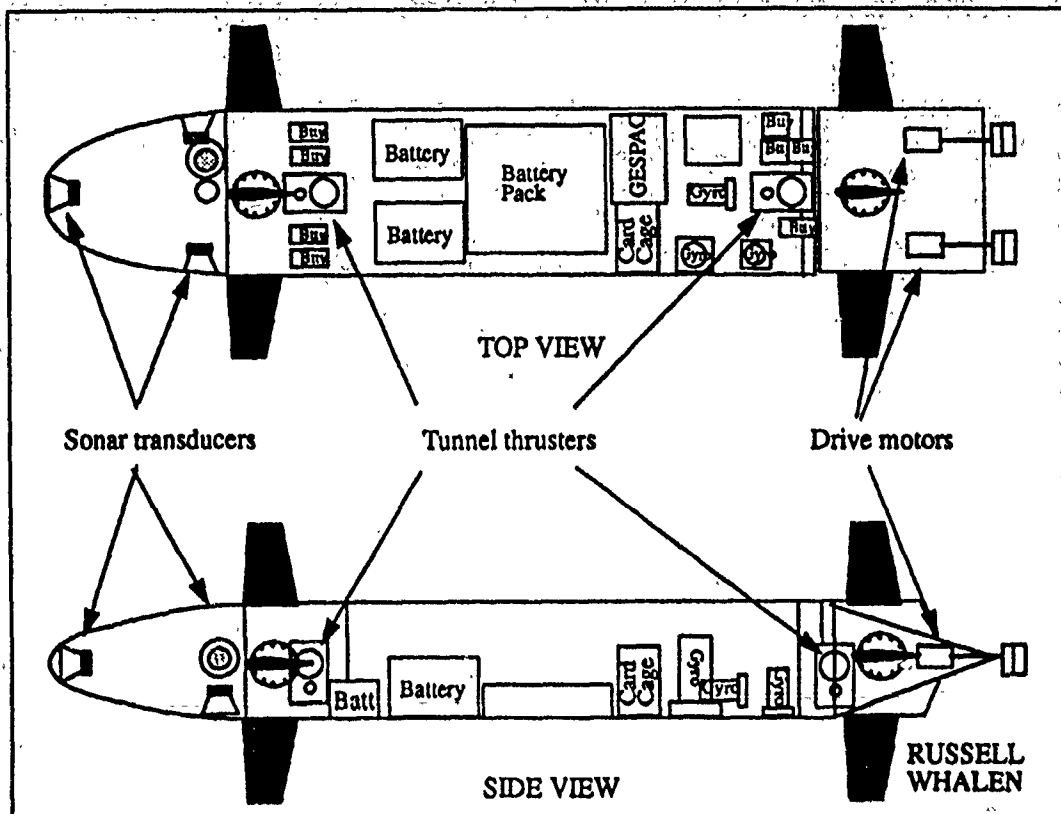
Figure 2.5 General schematic of the NPS AUV. Note the twin screws, four sonar transducers forward, and eight plane surfaces
