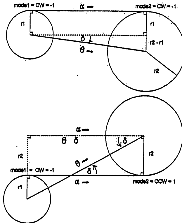
Figure 5: Cross and External Tangents
