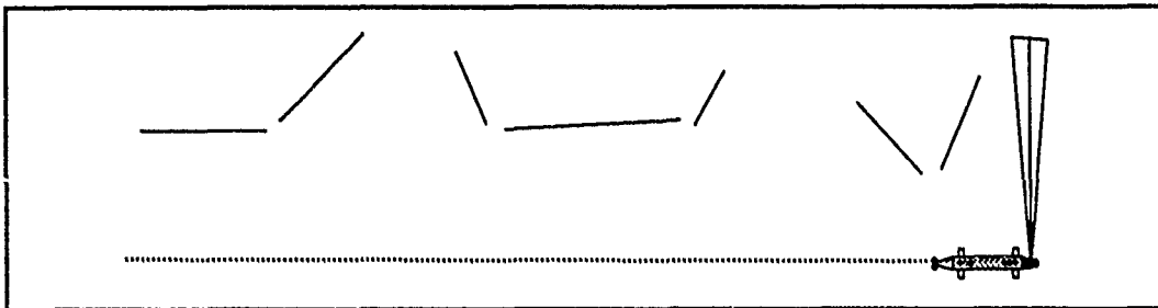
Figure 6.4 Examples of convex regression line segments
