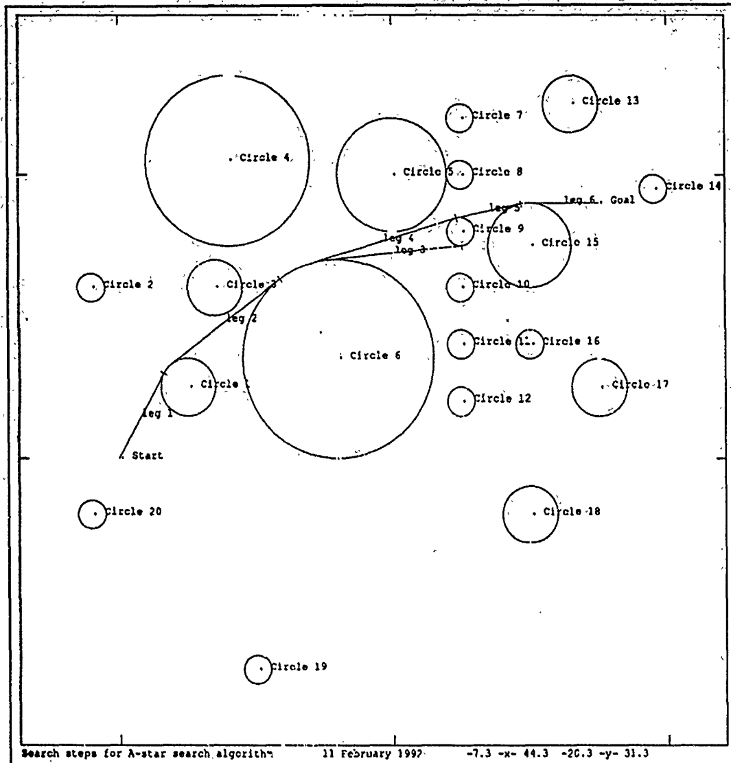
Figure 7.16 Search steps displayed for A* search algorithm
