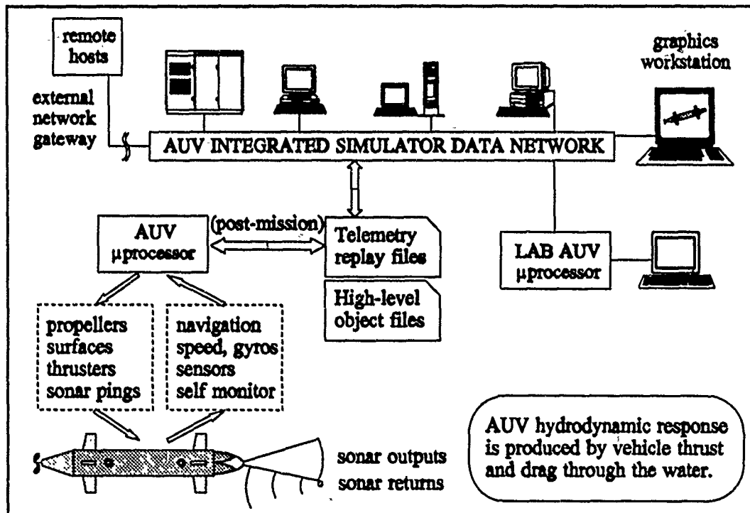
Figure 3.2 Integrated simulator logical connectivity using actual AUV
