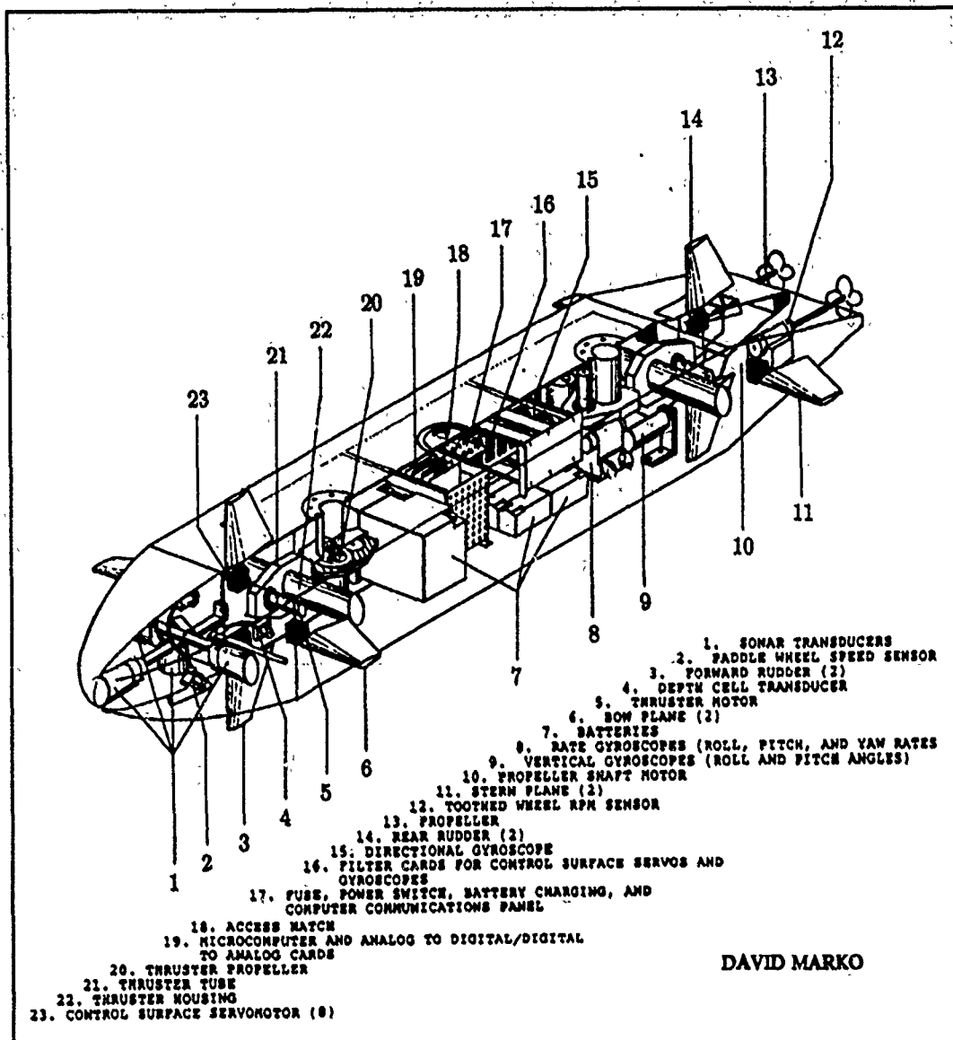
Figure 3.7 General schematic of NPS AUV to scale
