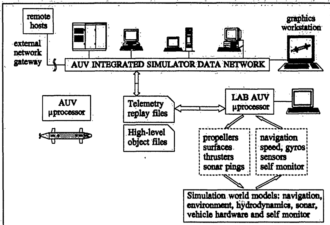
Figure 3.3 Integrated simulator logical connectivity using laboratory AUV
