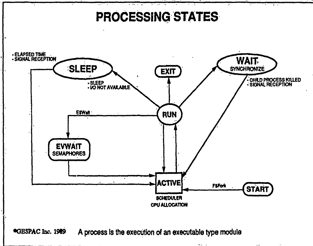
Figure 8.2 OS-9 operating system process states
