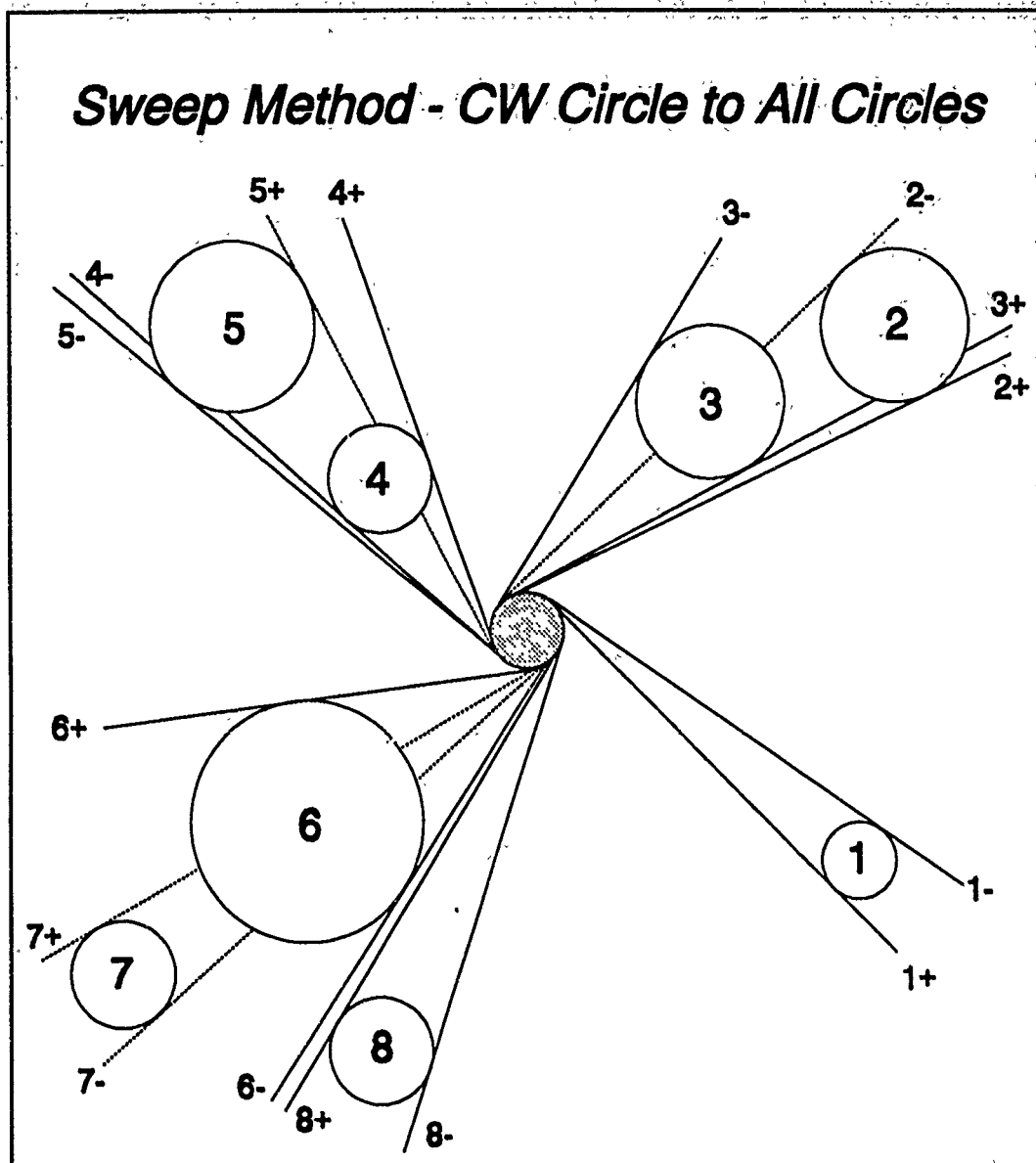
Figure 7.12 Sweep visibility determination from clockwise circle to all circles
