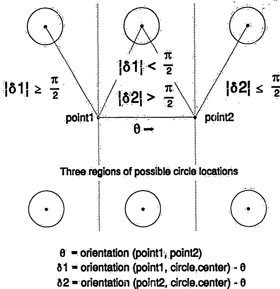
Figure 7.7 Determining point-to-point visibility in circle world.
