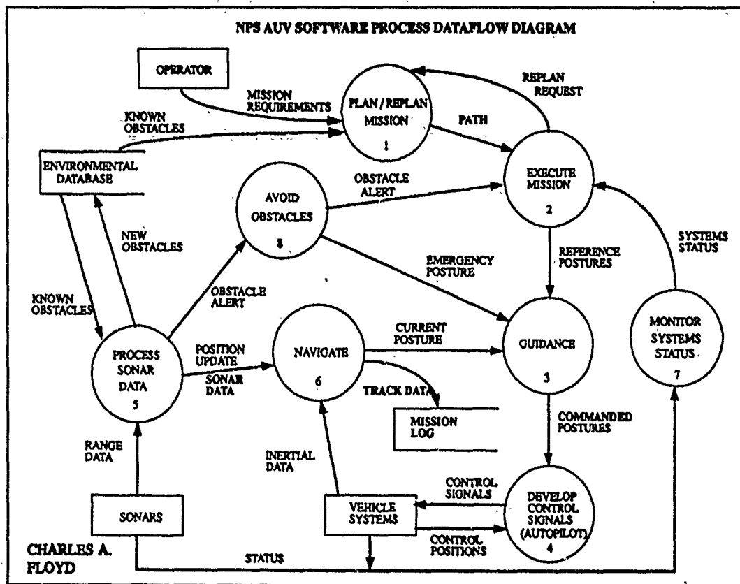
Figure 8.1 NPS AUV software process dataflow diagram
