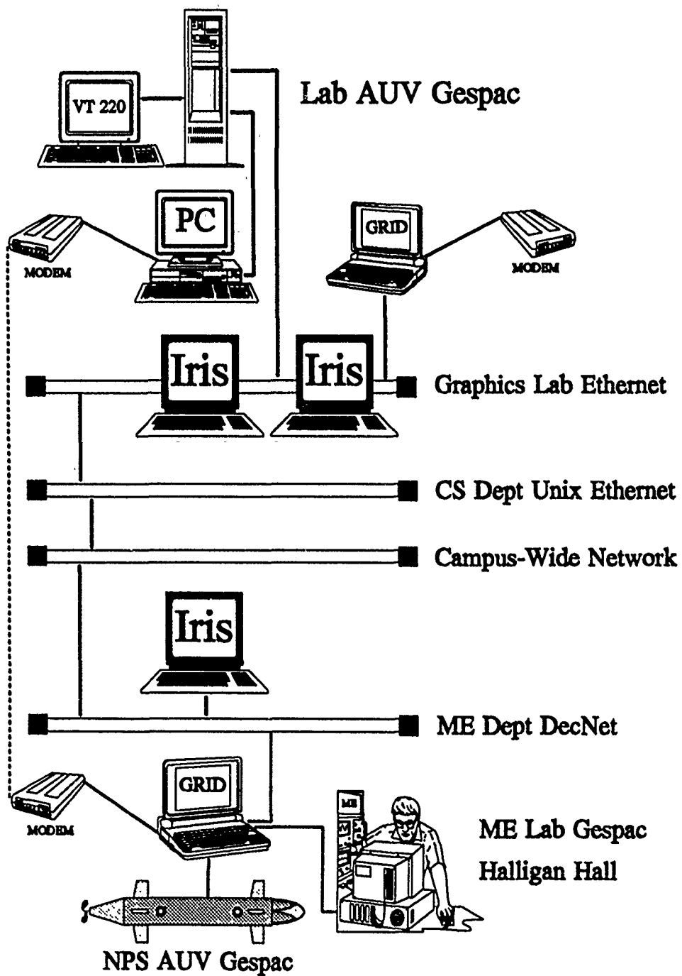
Figure 5.1 NPS AUV Integrated Simulator data network
