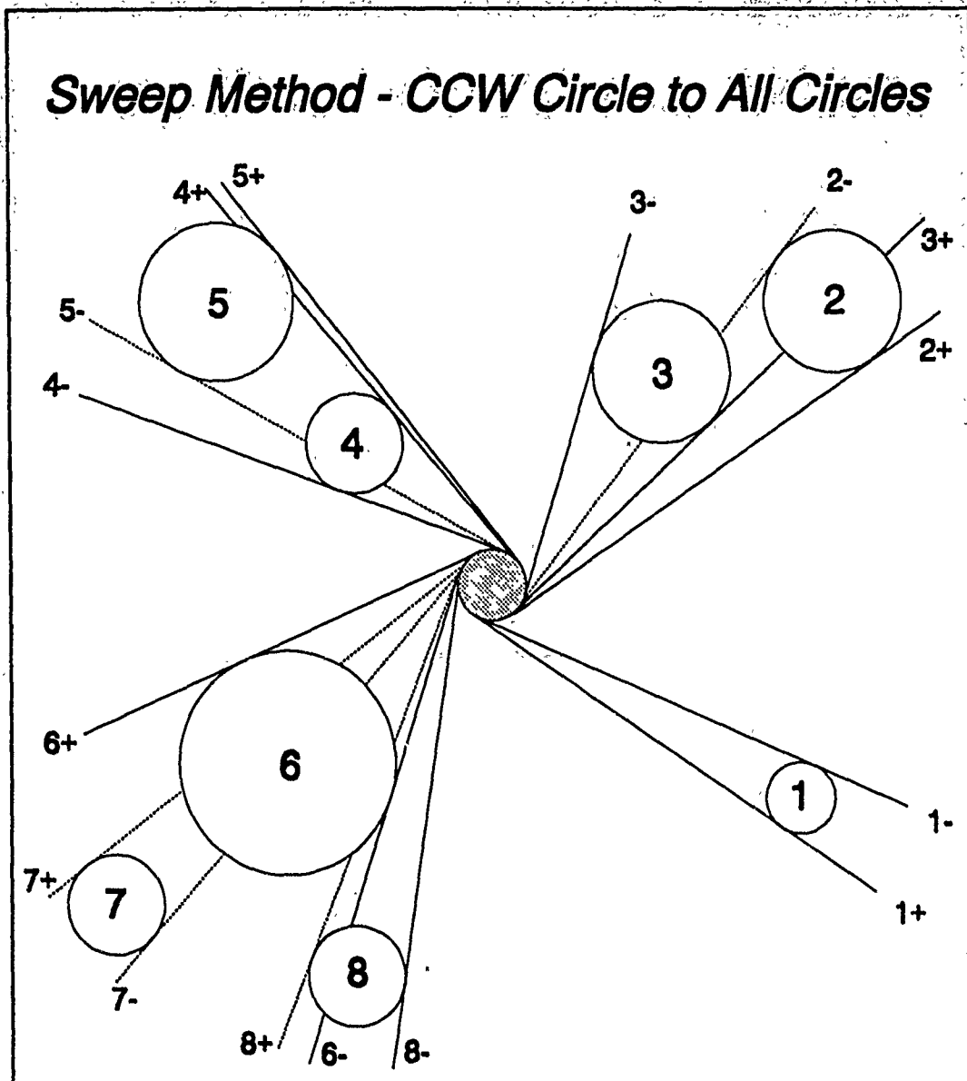
Figure 7.13 Sweep visibility determination from counter-clockwise circle to all circles
