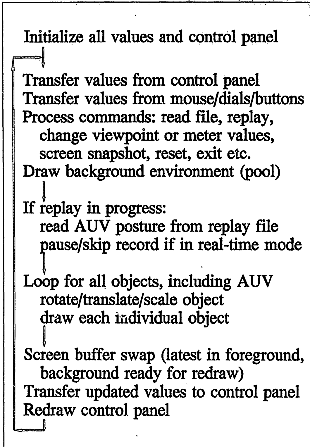
Figure B.1 NPS AUV graphics simulation program
