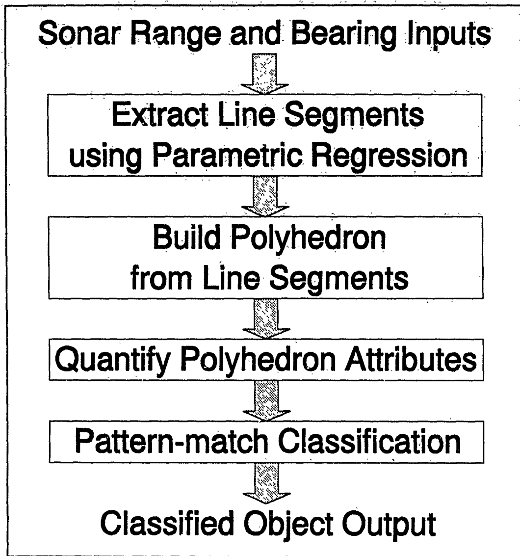
Figure 6.1 Autonomous sonar classification process diagram
