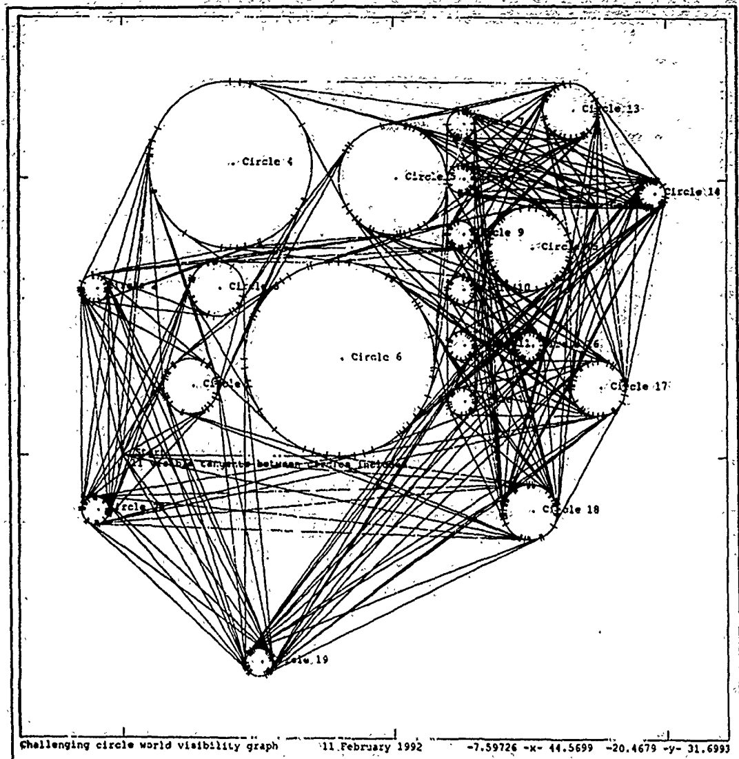
Figure 7.17 Challenging circle world visibility graph
