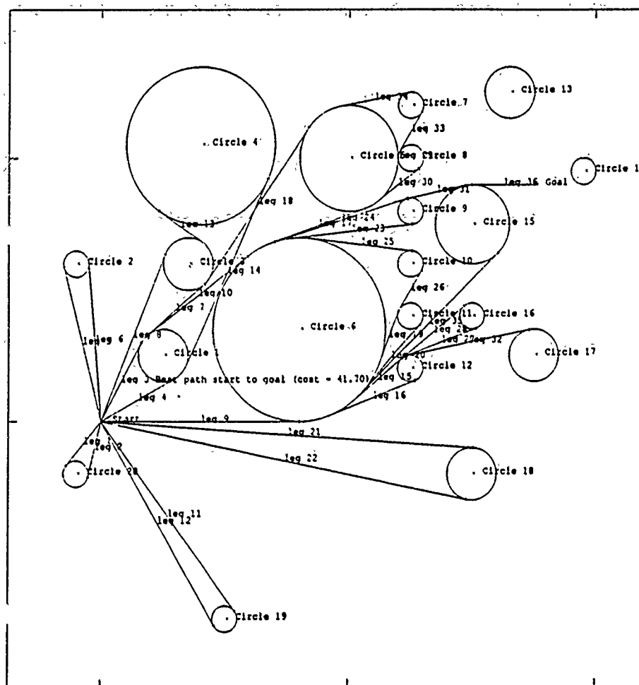
Figure 12: Result: Dijkstra's Algorithm
