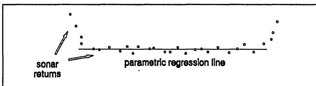
Figure 6.2 Typical parametric regression line fit
