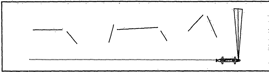
Figure 6.5 Examples of concave regression line segments
