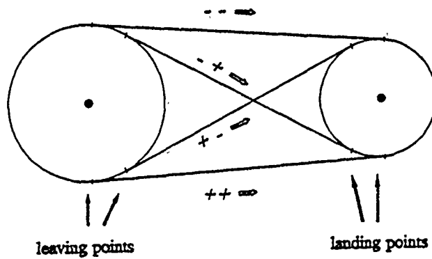
Figure 4: Tangents from Circle to Circle
