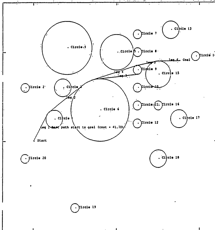
Figure 14: Result: A* Algorithm
