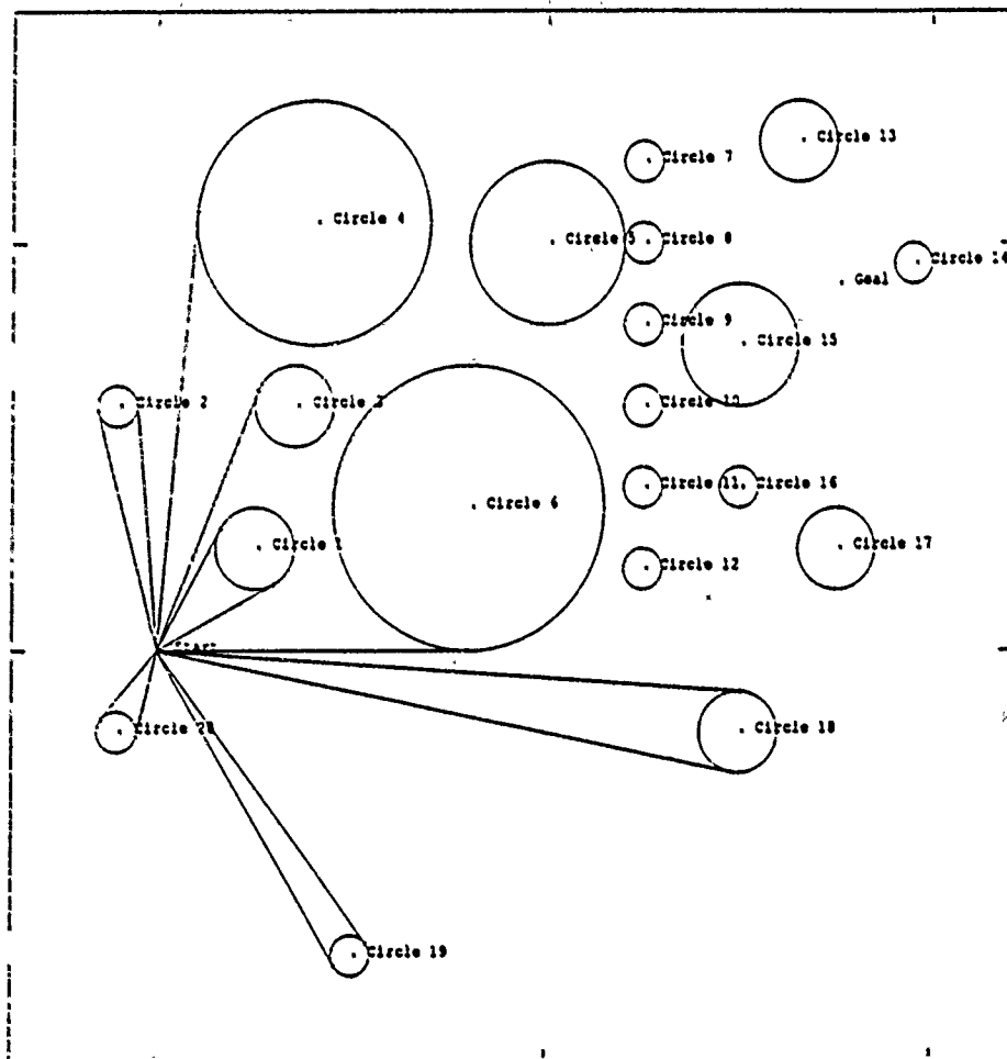
Figure 7: Tangents from Start
