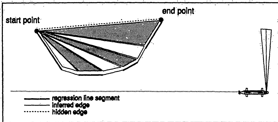
Figure 6.7 Summing triangle areas to determine polyhedron cross-sectional area
