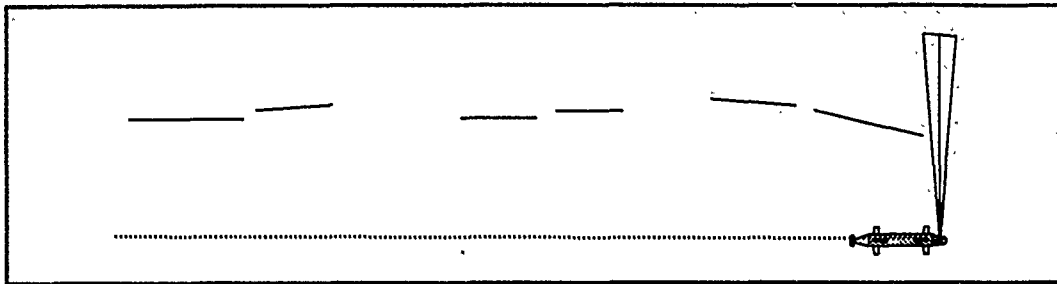
Figure 6.3 Examples of colinear regression line segments
