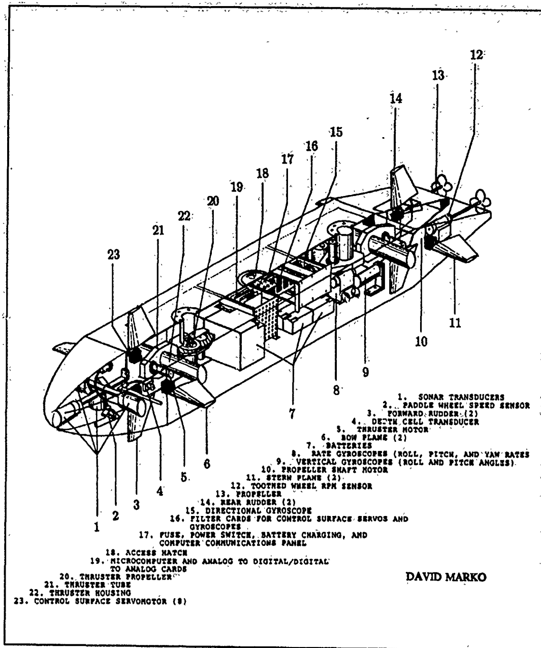
Figure 6.10 General schematic of NPS AUV
