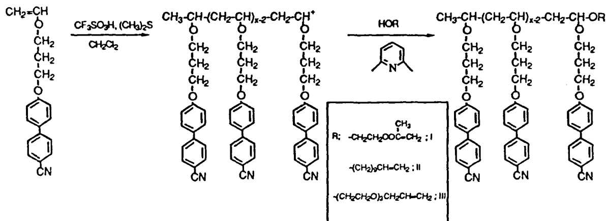
Scheme 1. Synthesis of Macromonomers
