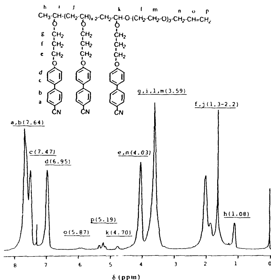
Figure 4. 200 MHz ^1\text{H} -NMR spectrum of poly(6-3)-III.
