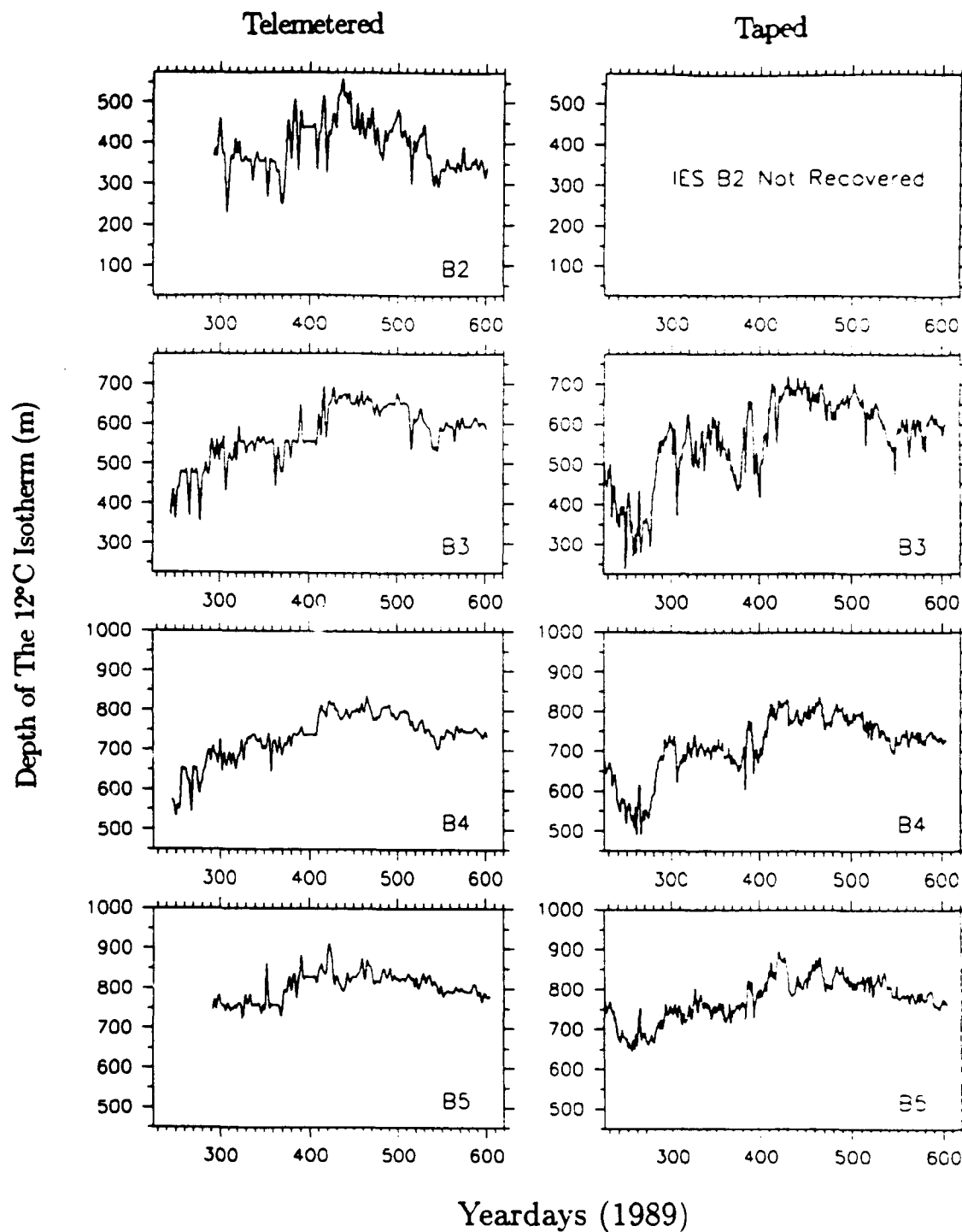
Figure 19: The column on the left shows the fully processed Z 12 records from the telemetered data. The column on the right shows the corresponding records from the data on the IES tapes. The Z 12 record from the tape data for IES B2 is not shown because the IES was not recovered.
