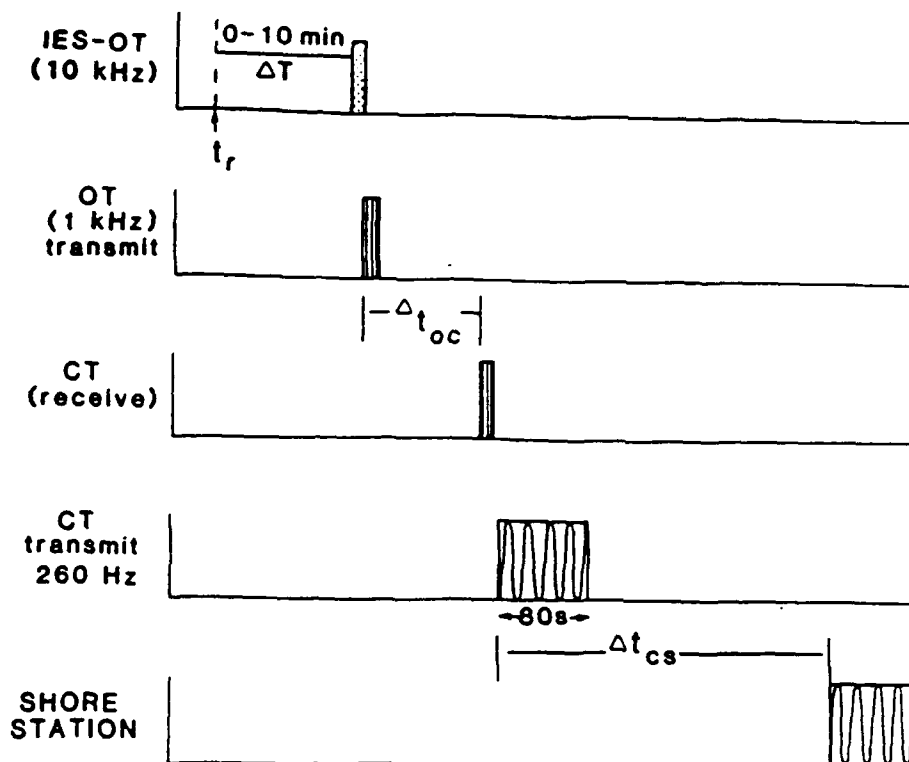
Figure 6: The timing of the delay encoded telemetered signal as it is relayed from an IES to Bermuda.
