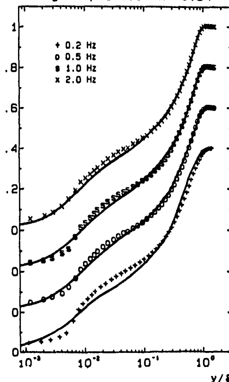
Figure 10. Comparison of computed and measured mean velocity profiles; high amplitude.
