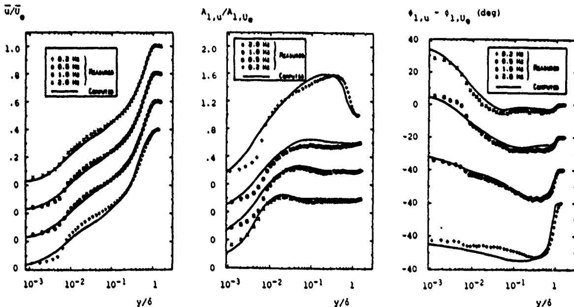
Fig. 7 Comparison of computed and measured mean velocity, A_{1,u} and phase profiles; high amplitude.
