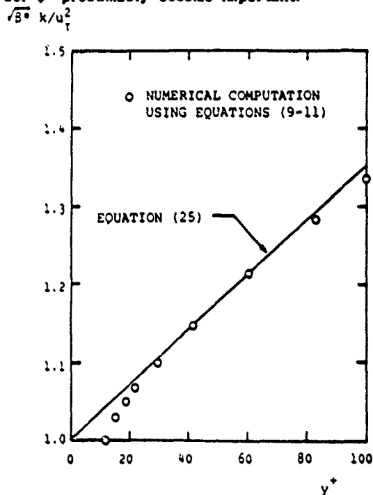
Figure 1. Deviation of computed turbulent energy from predicted near-wall behavior resulting from use of zeroth-order wall matching.
