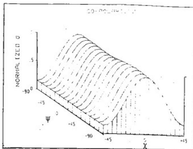
Figure 4 Co-Polarized Signature for Weeping Willow at 95 GHz
