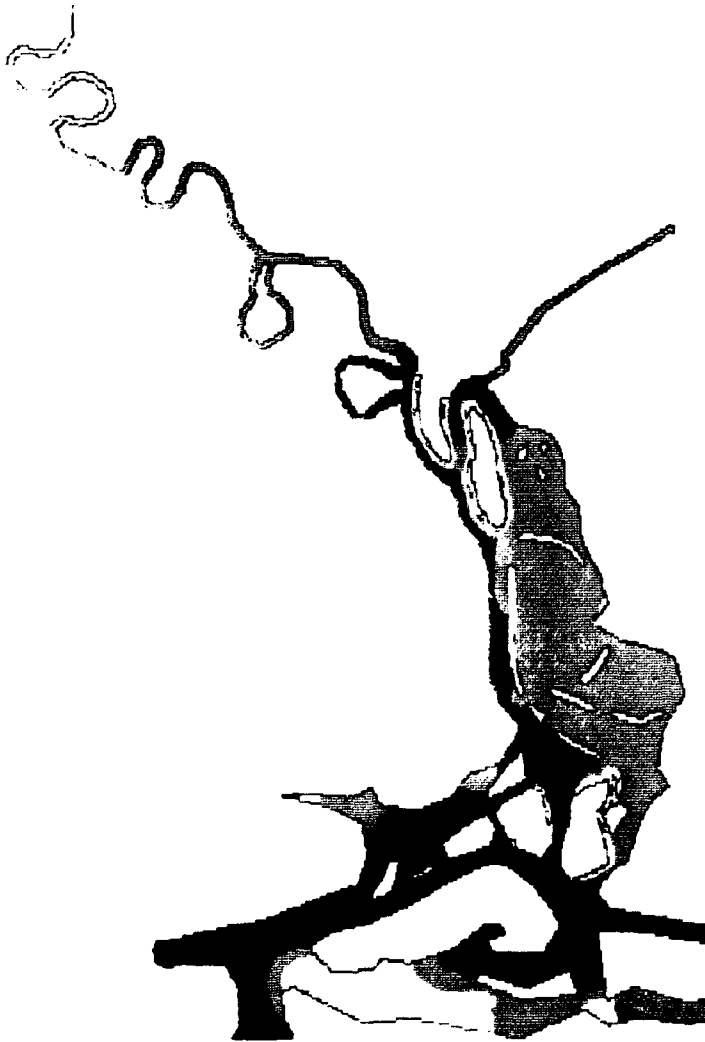
Figure 33. Tracer differences, Plan 2 - Base, low tide, Day 15
