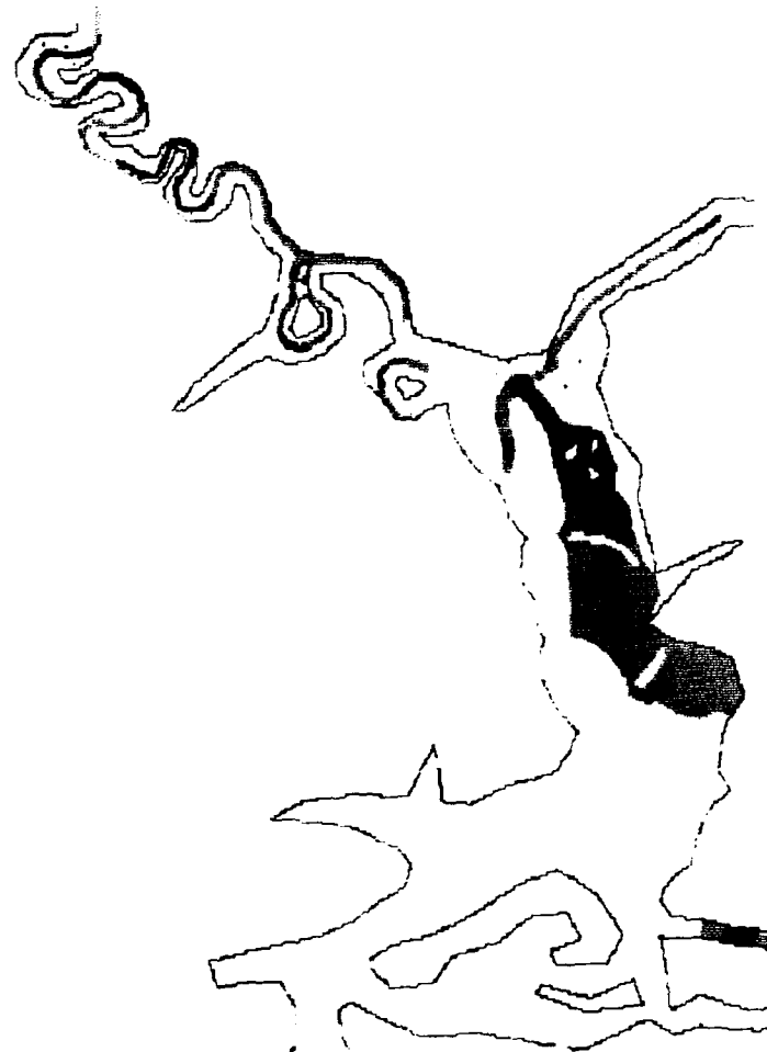
Figure 40. Tracer levels, Plan 3 Condition, high tide, Day 15
