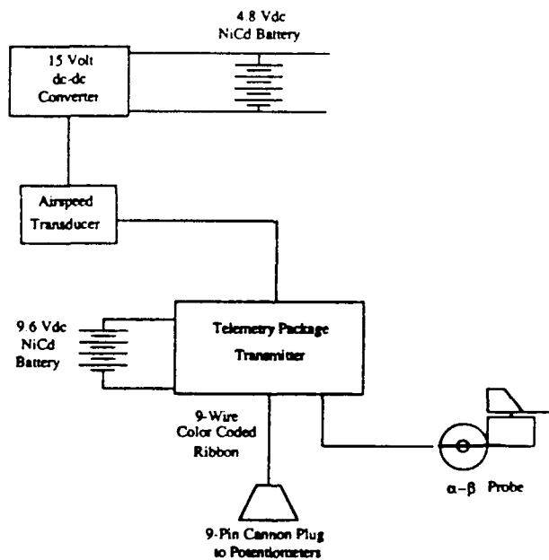
Figure 5: Data Acquisition System (Ref. 12)
