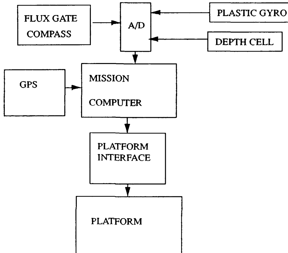
Figure 5: Interim Design
