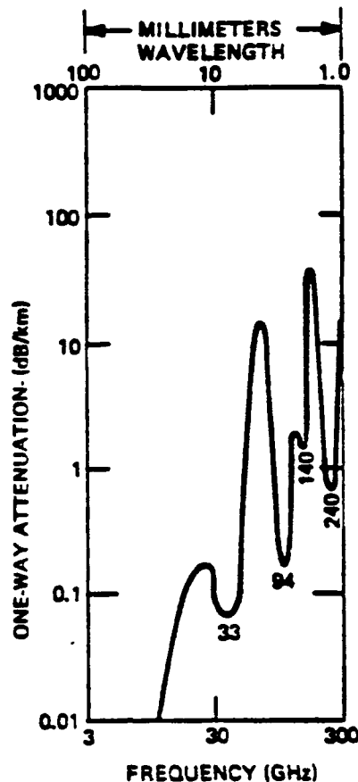
Figure 3. Prediction Chart in the Atmosphere for the Combined Effects of Oxygen and Water Vapor at Sea Level (Reprinted from Reference 2, page 33.)
