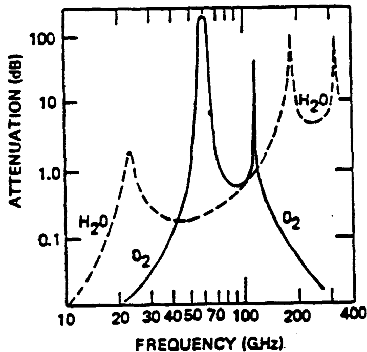
Figure 2. Prediction Chart for Atmospheric Attenuation of Oxygen and Water Vapor at Sea Level (Reprinted from Reference 2, page 32.)
