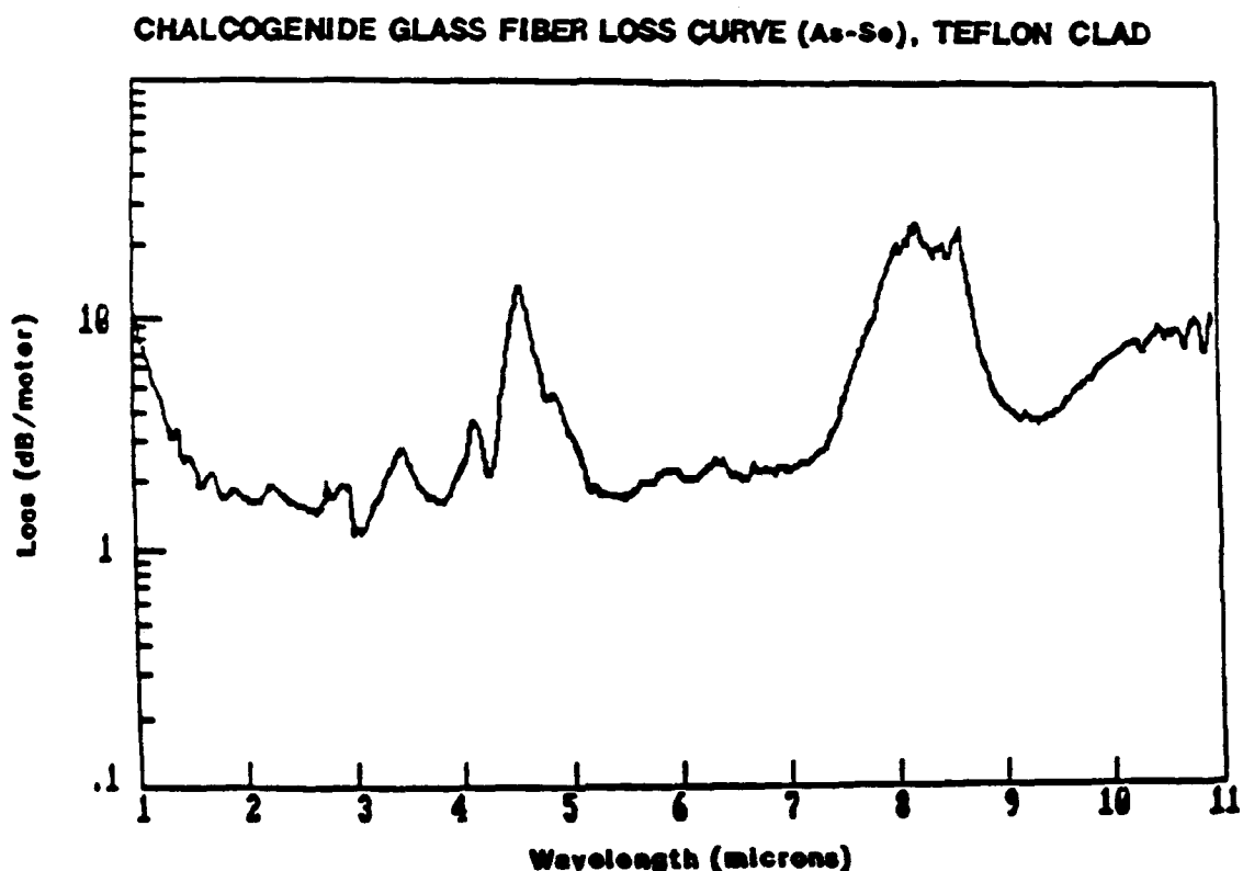
Figure 4. Chalcogenide Glass Fiber Loss Curve (As-Se), Teflon Clad (Reprinted from Reference 7, Figure 3.)
