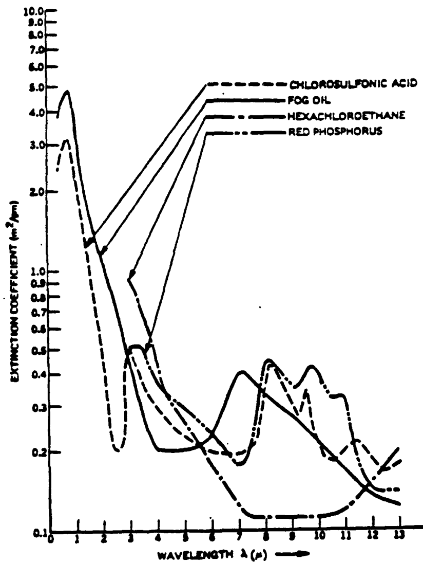
Figure 1. Smoke Extinction Coefficients (Reprinted from Reference 2, page 13.)
