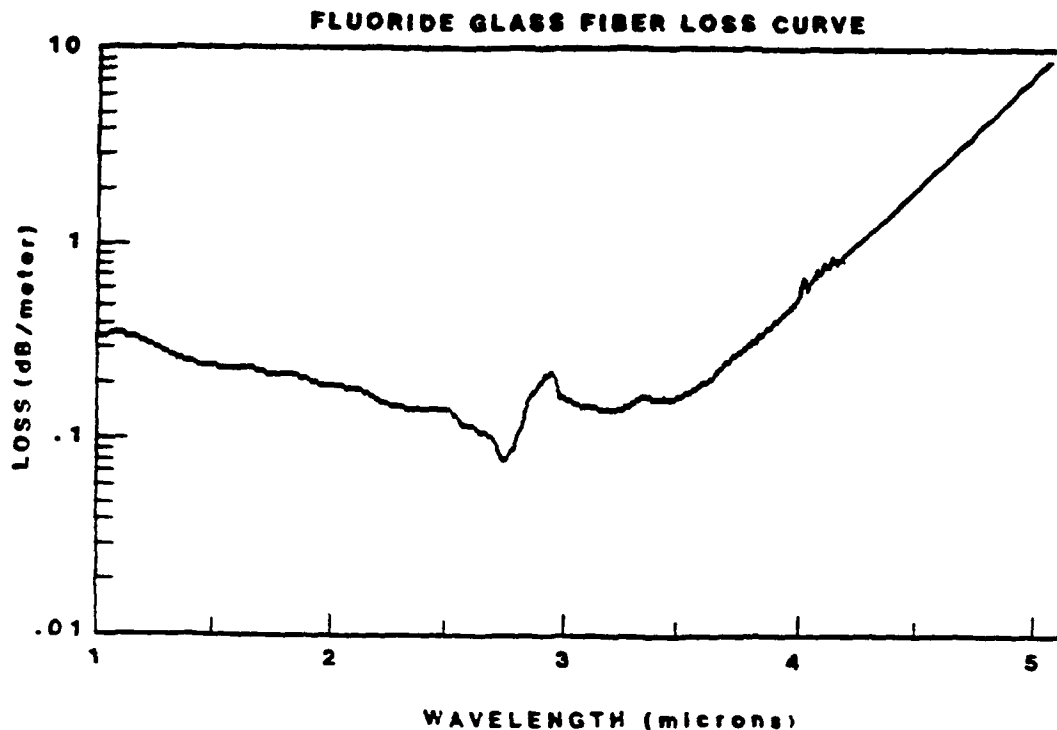
Figure 5. Fluoride Glass Fiber Loss Curve (Reprinted from Reference 7, Figure 1.)
