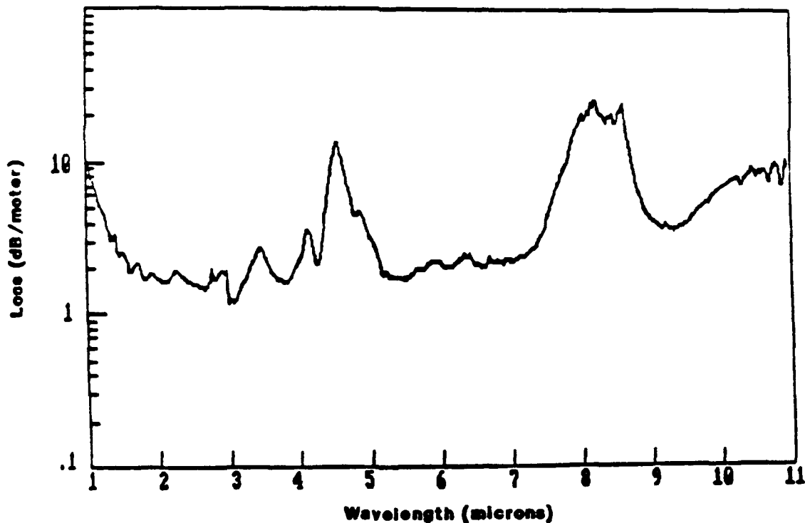
CHALCOGENIDE GLASS FIBER LOSS CURVE (As-Se), TEFLON CLAD
