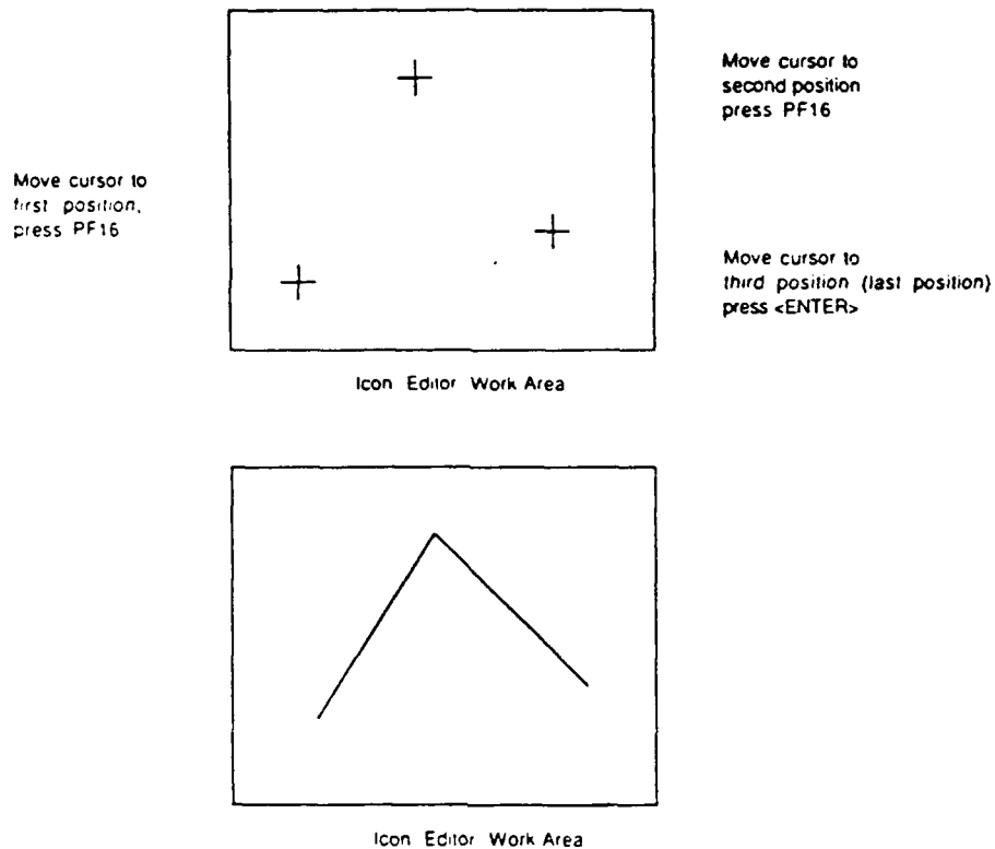
Figure 5-40 Polyline Primitive
