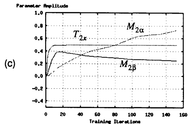
Figure 4: (a) The time evolution of the sample movement trajectory for both joints. (b) The training evolution of the end-of-movement position and velocity errors for both joints. (c) The training evolution of the adaptable parameters.
