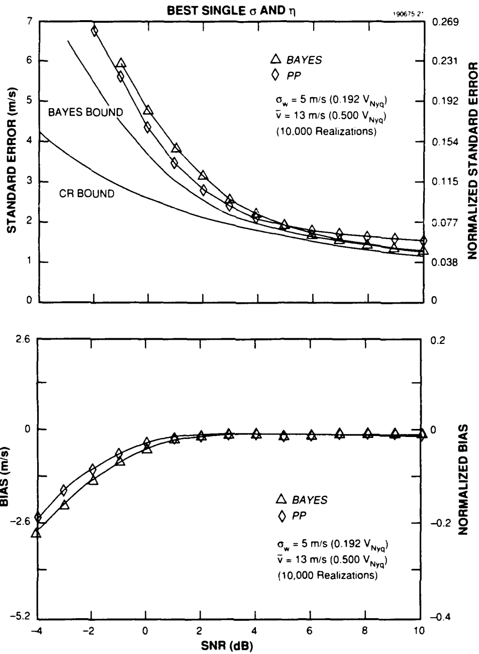
Figure 8. Bayes algorithm performance: suboptimal \sigma and \eta using best single-weighting coefficient set. (d) \bar{v} = 13 m/s, \sigma_w = 0.192 v_{Nyq} .
