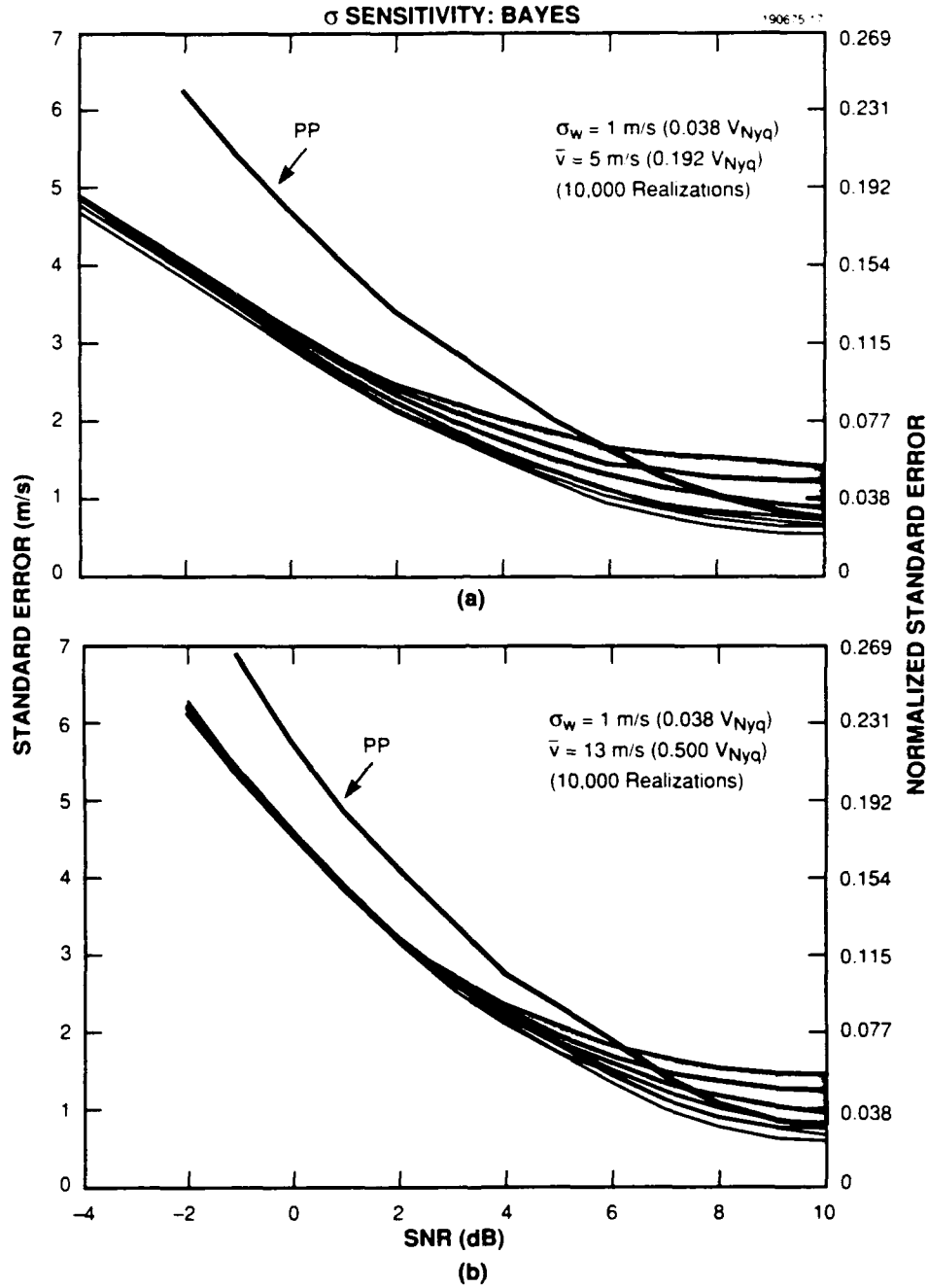
Figure 7. Bayes algorithm performance sensitivity: effect of spectrum width parameter \sigma . (a) \bar{v} = 5 m/s, \sigma_w = 0.038 v_{Nyq} . (b) \bar{v} = 13 m/s, \sigma_w = 0.038 v_{Nyq} .
