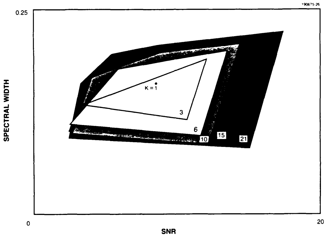
Figure 19. Set point convex hull with increasing K . Fundamental limitation on extent of set point convex hull is illustrated for a sequence with increasing K value.
