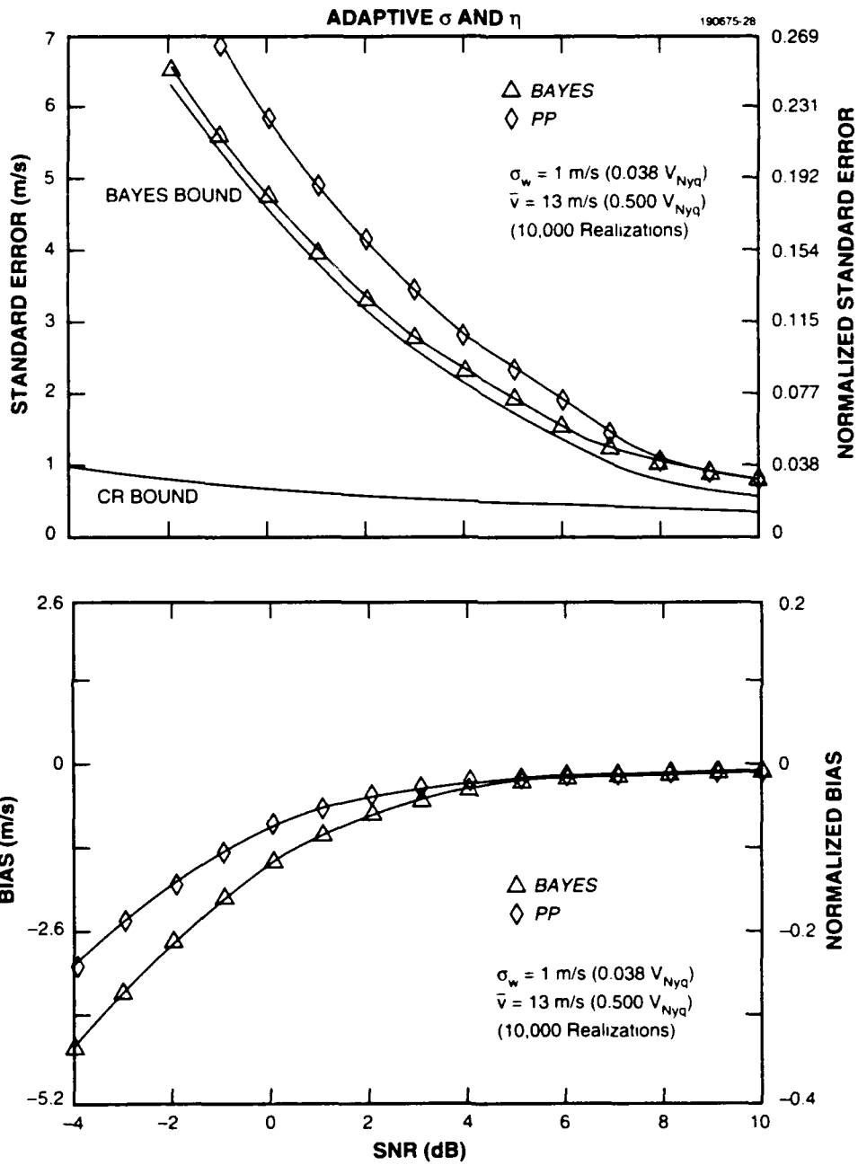
Figure 14. Bayes algorithm with adaptive \sigma and \eta : 15 compartment weighting coefficient set (1). (b) \bar{v} = 13 \text{ m/s} , \sigma_w = 0.038 v_{Nyq} .
