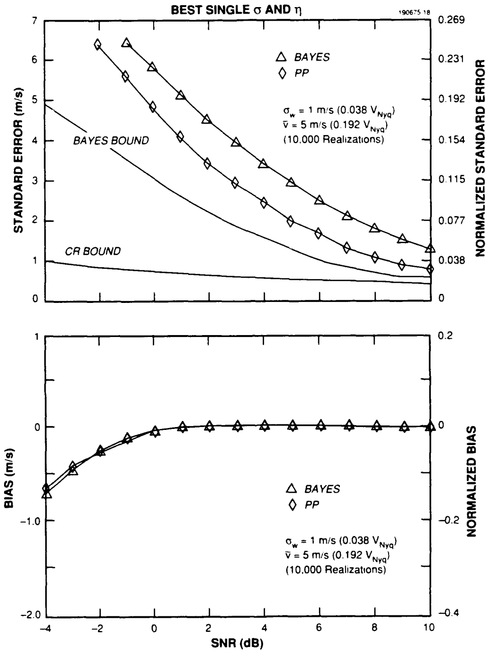
Figure 8. Bayes algorithm performance: suboptimal \sigma and \eta using best single-weighting coefficient set. (a) \bar{v} = 5 m/s, \sigma_w = 0.038 v_{Nyq} .
