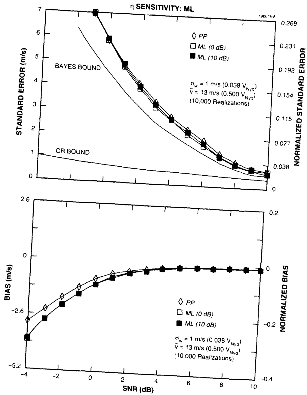
Figure 4. ML algorithm performance sensitivity: effect of signal-to-noise parameter \eta . (b) \bar{v} = 13 \text{ m/s} , \sigma_w = 0.038 v_{Nyq} .
