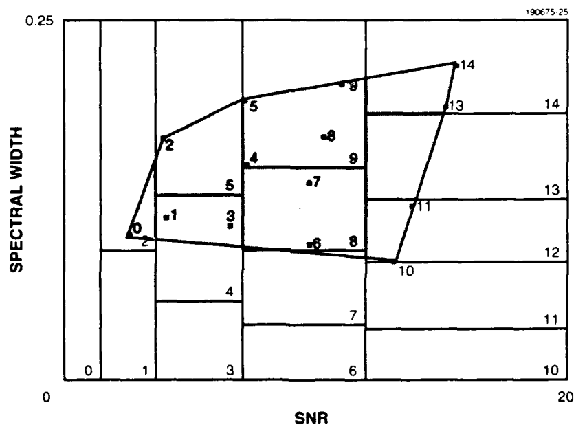
Figure 12. Optimum partition and set point locations.
