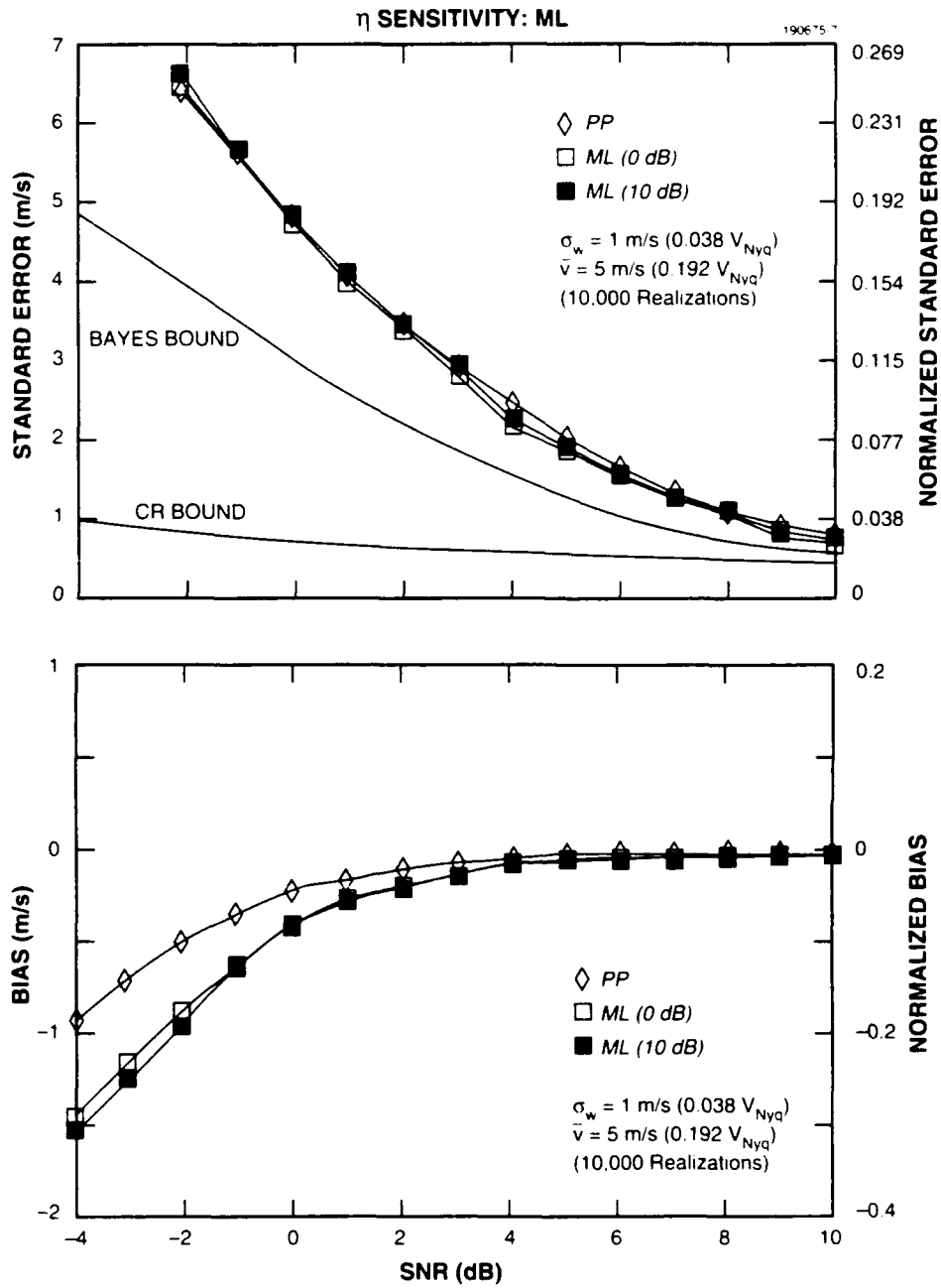
Figure 4. ML algorithm performance sensitivity: effect of signal-to-noise parameter \eta . (a) \bar{v} = 5 \text{ m/s} , \sigma_w = 0.038 v_{Nyq} .
