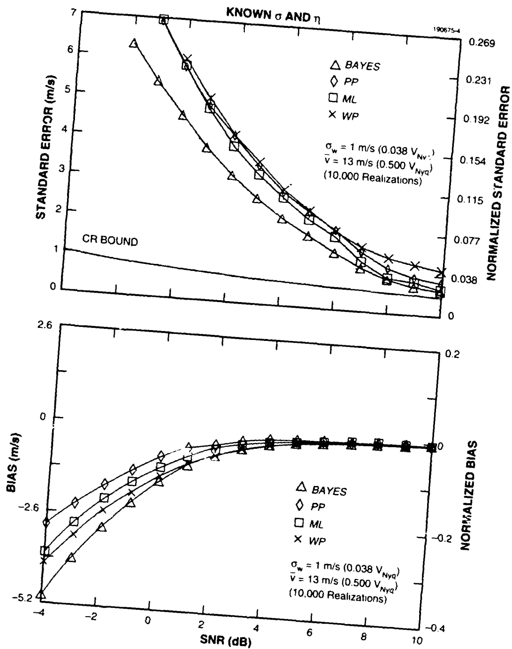
Figure 9. Optimal performance: standard error and bias results for nonzero velocities. (b) \bar{v} = 13 \text{ m/s} , \sigma_w = 0.038 v_{Nyq} .
