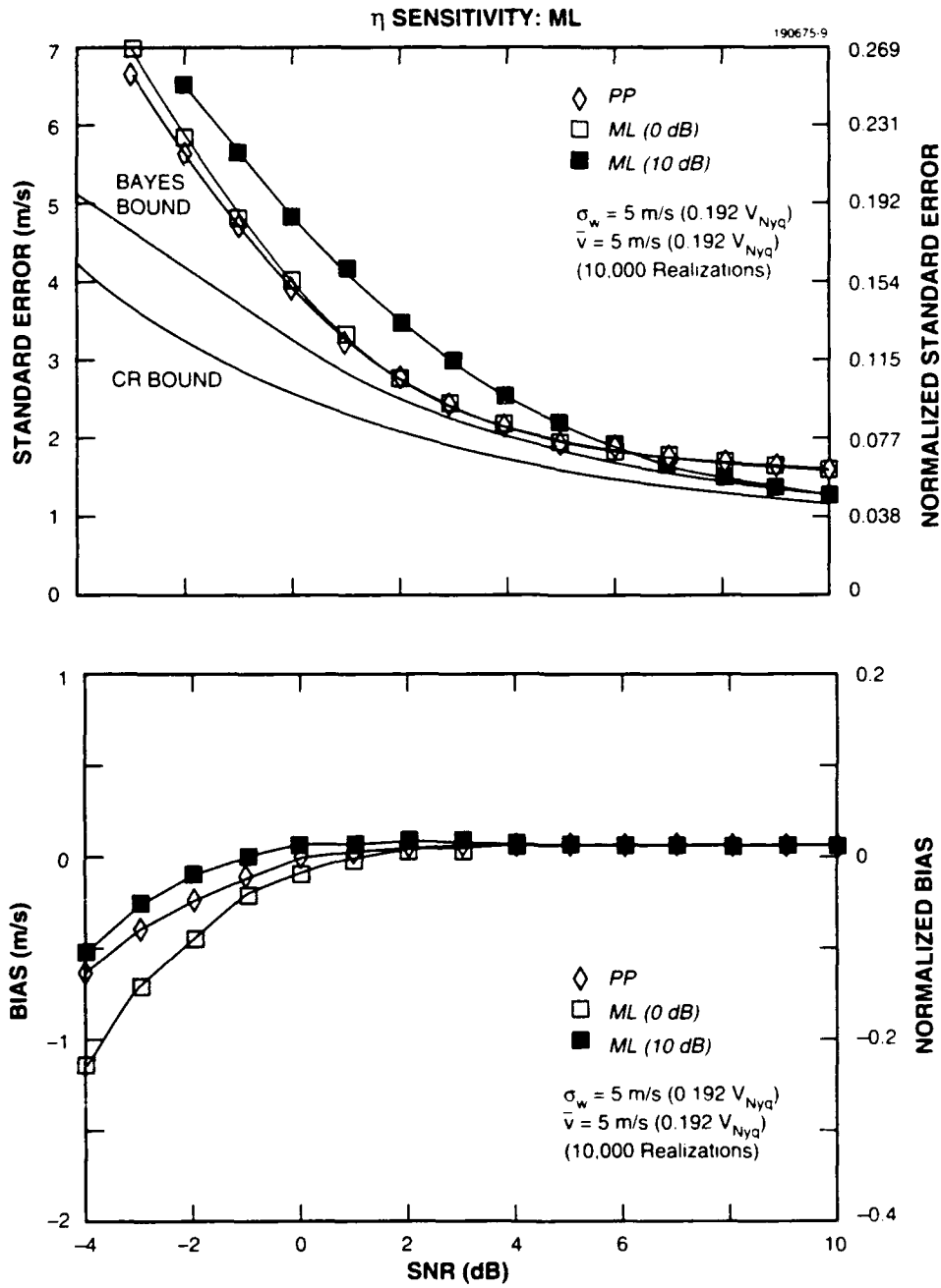
Figure 4. ML algorithm performance sensitivity: effect of signal-to-noise parameter \eta . (c) \bar{v} = 5 \text{ m/s} , \sigma_w = 0.192 v_{Nyq} .
