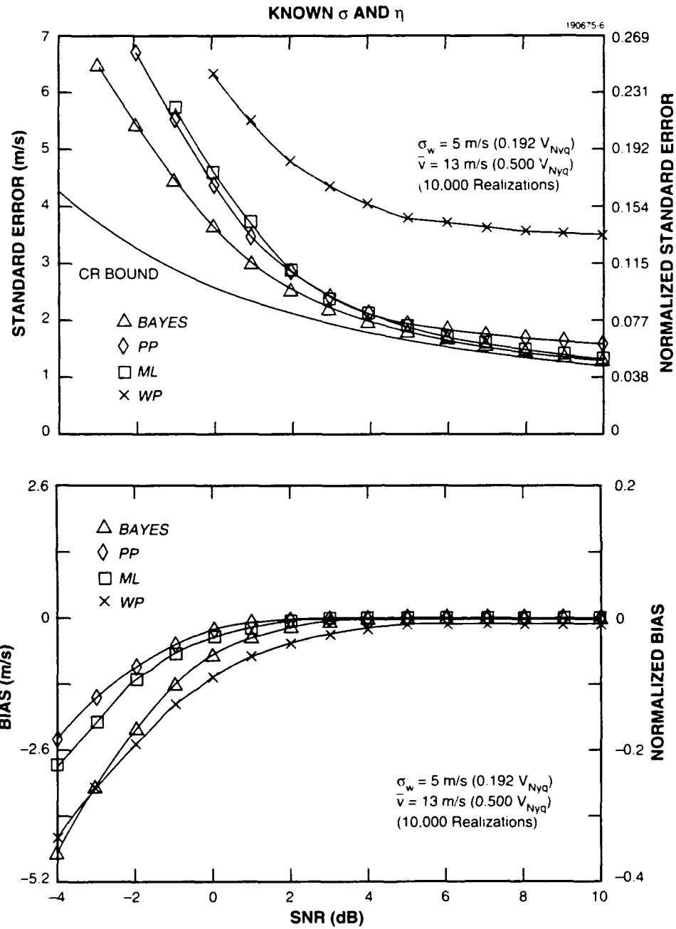
Figure 9. Optimal performance: standard error and bias results for nonzero velocities. (d) \bar{v} = 13 \text{ m/s} , \sigma_w = 0.192 v_{Nyq} .
