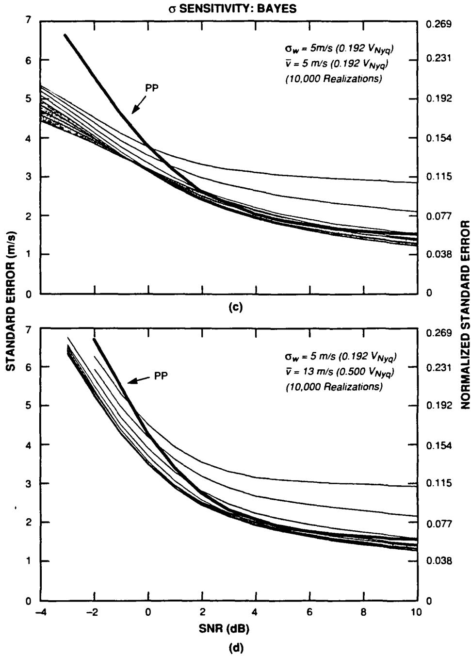
Figure 7. Bayes algorithm performance sensitivity: effect of spectrum width parameter \sigma . (c) \bar{v} = 5 \text{ m/s} , \sigma_w = 0.192 v_{Nyq} . (d) \bar{v} = 13 \text{ m/s} , \sigma_w = 0.192 v_{Nyq} .
