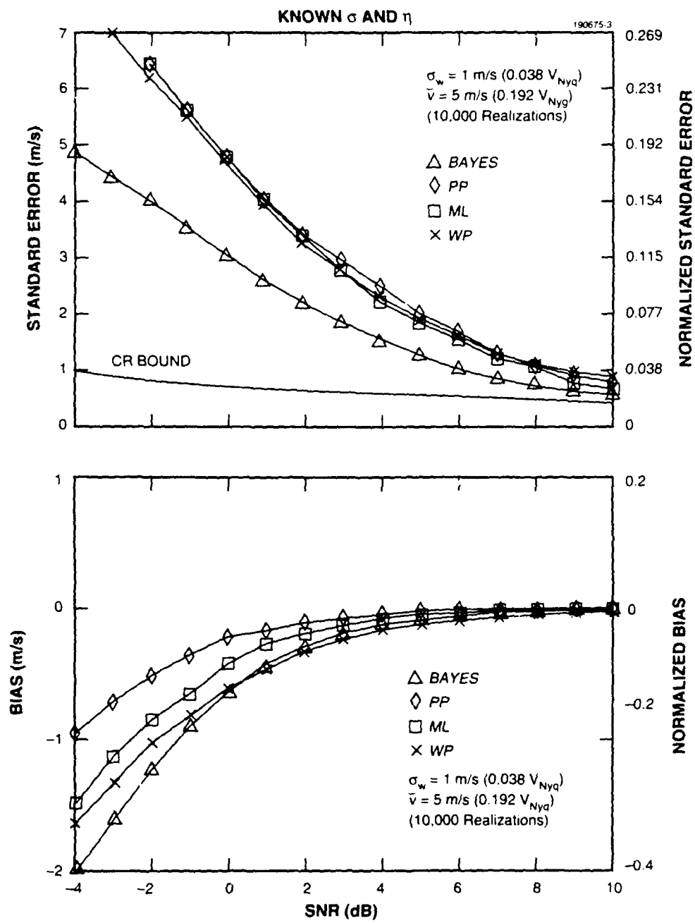
Figure 3. Optimal performance: standard error and bias results for nonzero velocities. (a) \bar{v} = 5 \text{ m/s} , \sigma_w = 0.038 v_{Nyq} .
