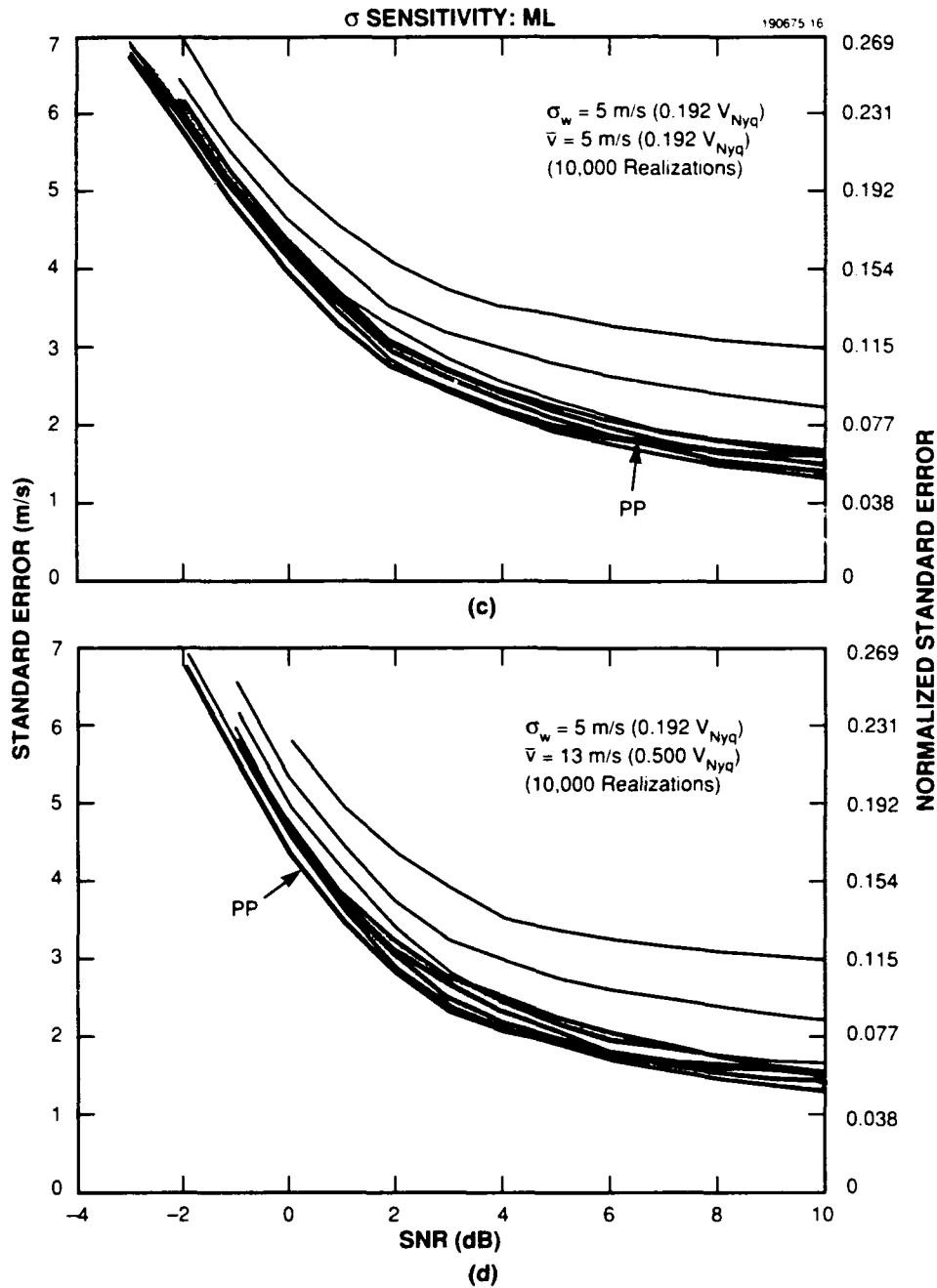
Figure 6. ML algorithm performance sensitivity: effect of spectrum width parameter \sigma . (c) \bar{v} = 5 \text{ m/s} , \sigma_w = 0.192 v_{Nyq} . (d) \bar{v} = 13 \text{ m/s} , \sigma_w = 0.192 v_{Nyq} .
