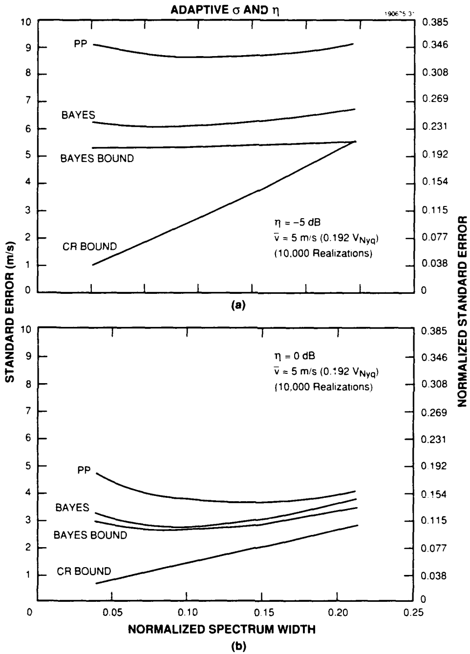
Figure 15. Bayes algorithm with adaptive \sigma and \eta : 15 compartment weighting coefficient set (II). (a) SNR = -5 dB. (b) SNR = 0 dB.
