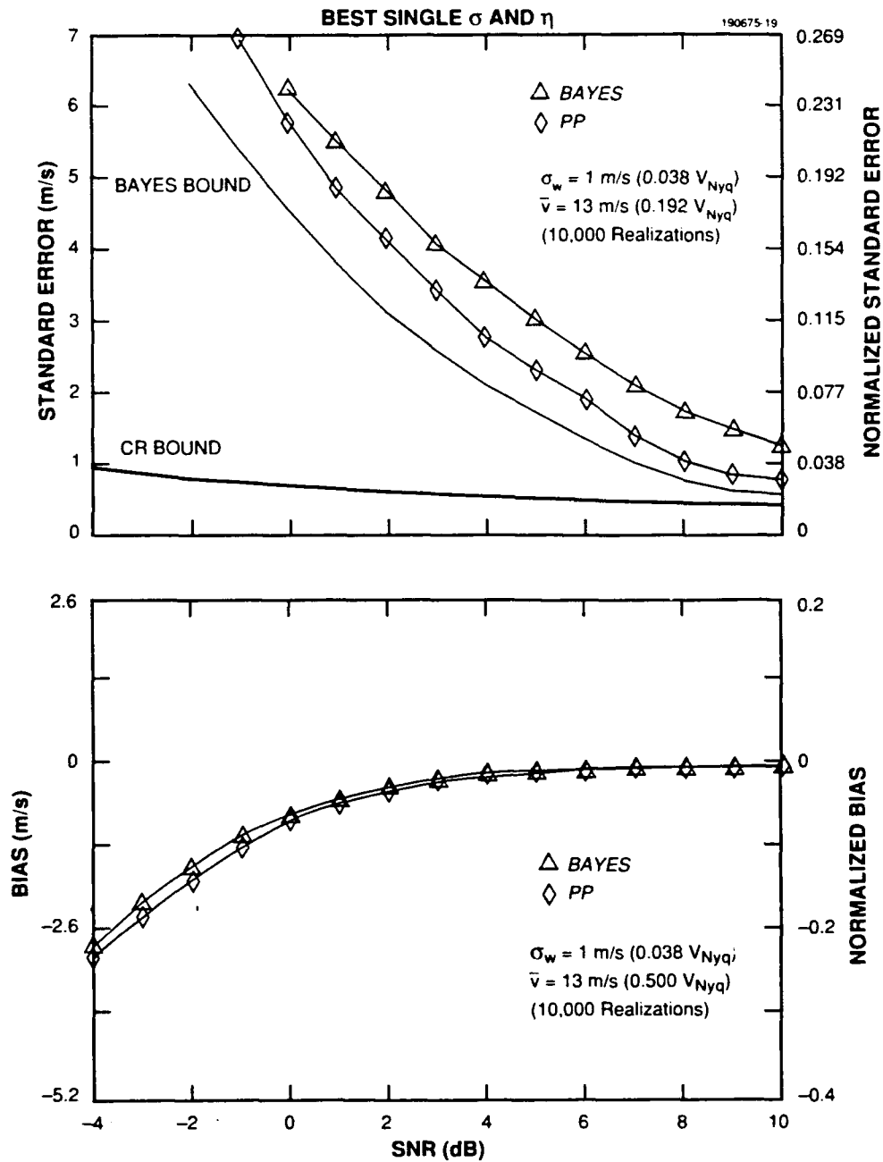
Figure 8. Bayes algorithm performance: suboptimal \sigma and \eta using best single-weighting coefficient set. (b) \bar{v} = 13 \text{ m/s} , \sigma_w = 0.038 v_{Nyq} .
