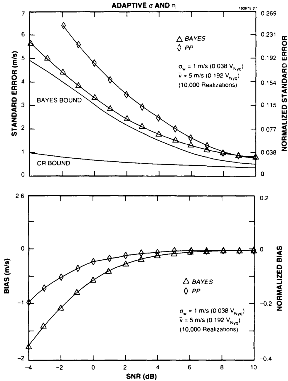
Figure 14. Bayes algorithm with adaptive \sigma and \eta : 15 compartment weighting coefficient set (I). (a) \bar{v} = 5 m/s, \sigma_w = 0.038 v_{Nyq} .
