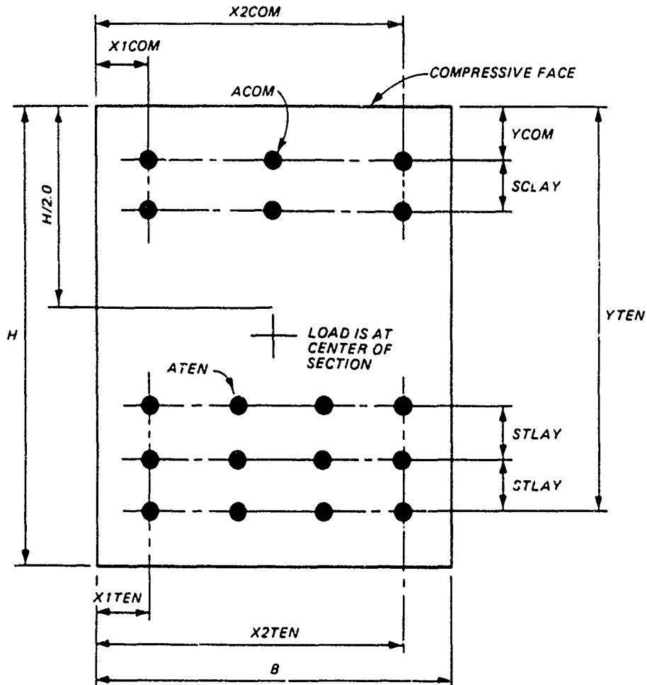
Figure 6. Beam design variables
