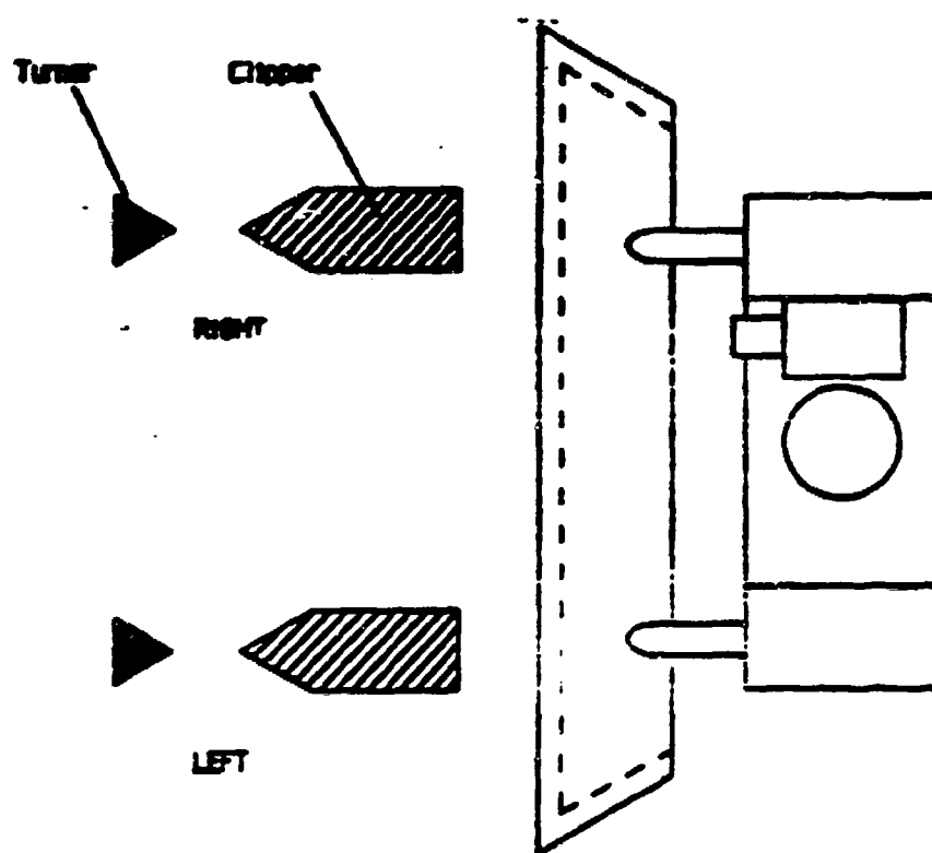
Figure 14. Top View of End-Effector Approaching Turning Device
