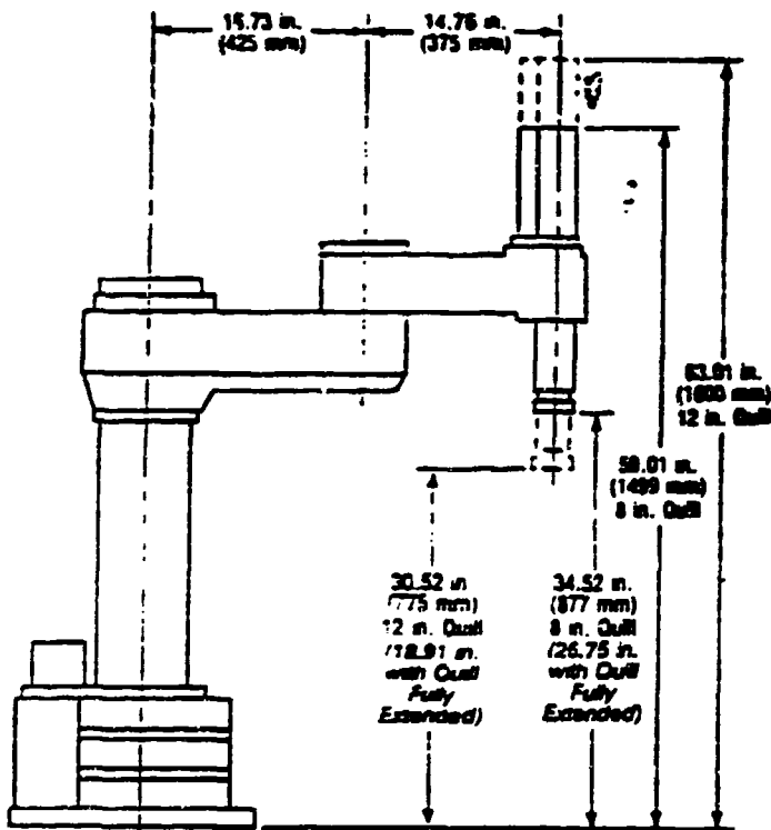
Manipulator (side view)
