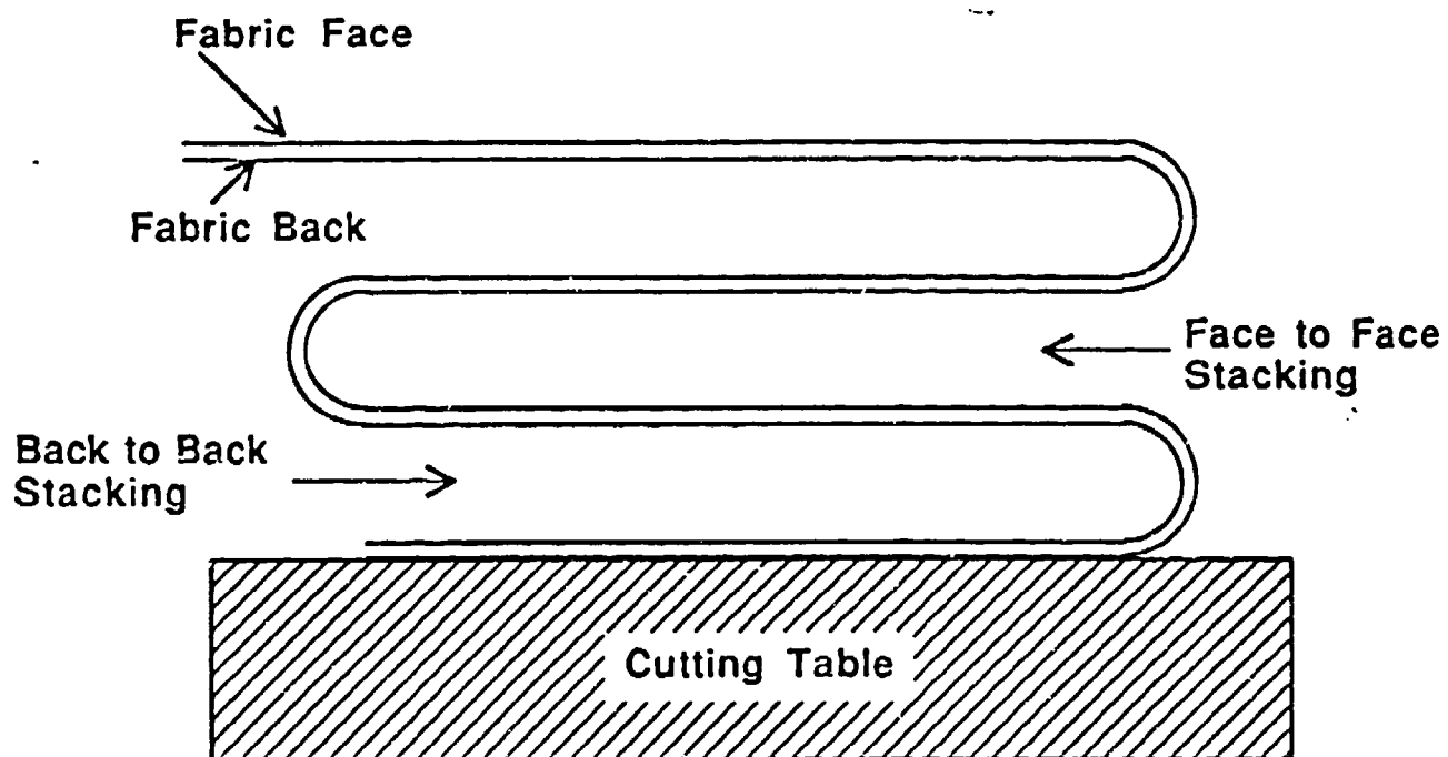
Figure 1. Typical spreading of fabric showing type of contact.
