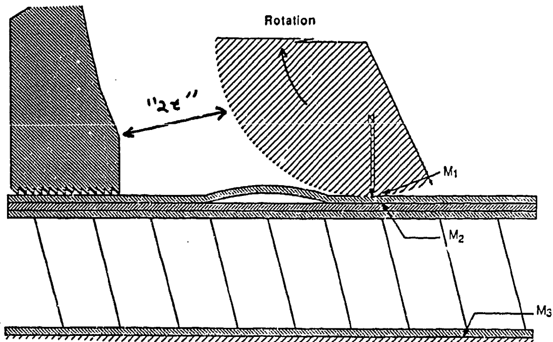
Figure 2. Illustration of the gap width between the wheel and the shoe (" 2t " is compressed 2-ply thickness).
