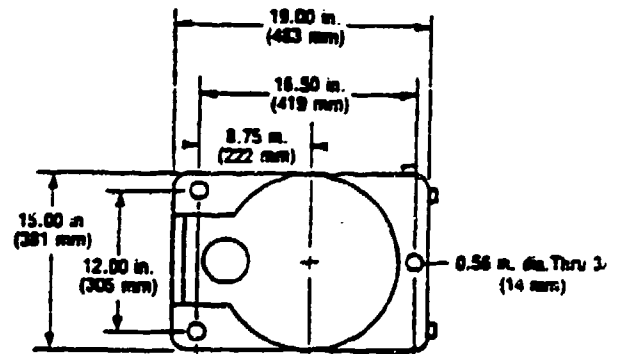
Manipulator Base (plan view)
