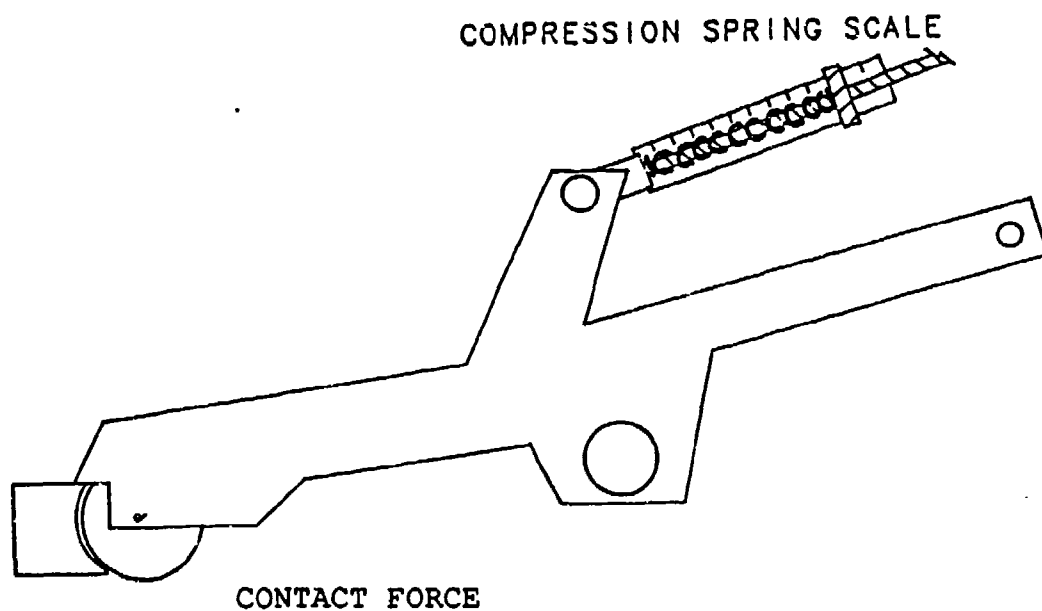
Figure 1. Clupicker compression spring adjustment for controlling fabric contact force.
