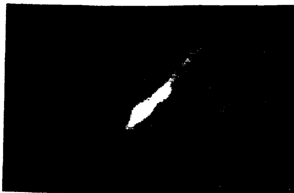
Fig. 14. Synchronous box-car image of a quarter-inch thick graphite-epoxy laminate that had been impacted by a ball bearing. Gate delay is 33 ms. Note indications of surface ply structure (45° lines), and near subsurface delamination (red area) caused by the impact.
