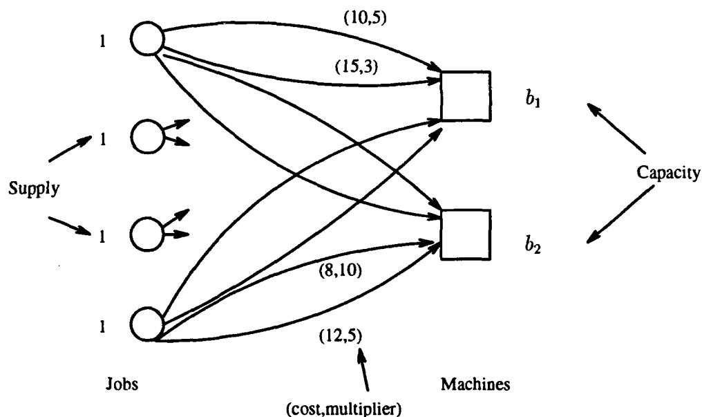
FIGURE 1. Generalized network for variable-speed problem
