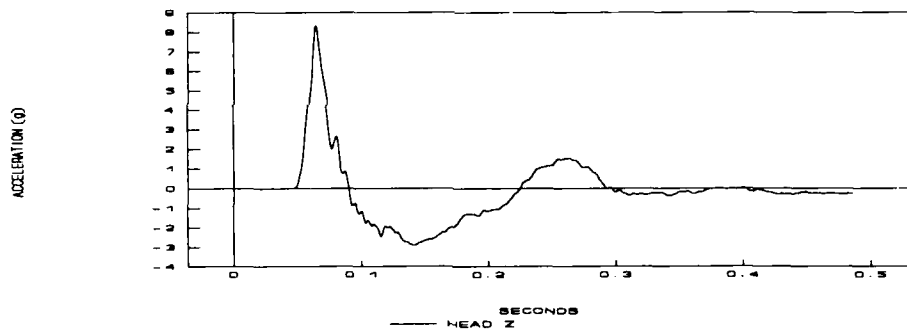
NBDL VERTICAL ACCELERATOR TEST - LZ0090 07 JULY 67
