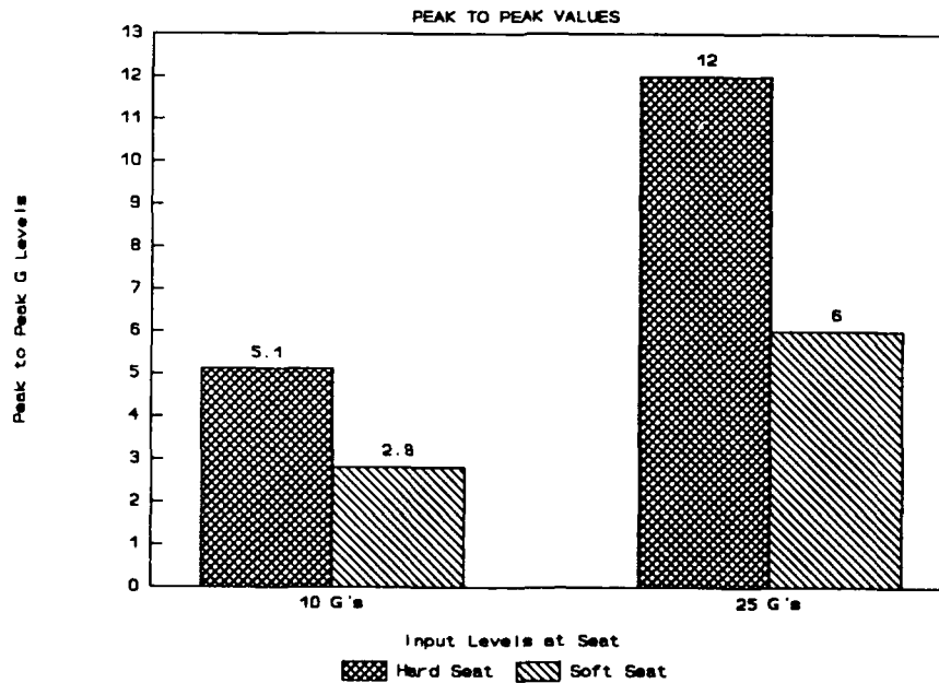
Figure 17. Head X Linear Acceleration.
