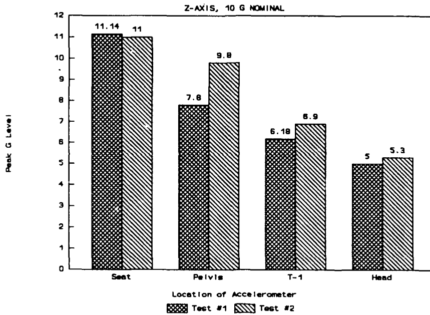
Figure 8. Hard Seat Repeatability.
