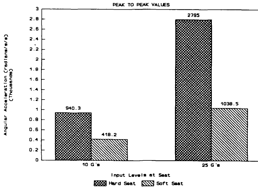
Figure 16. Head @Y Angular Acceleration.
