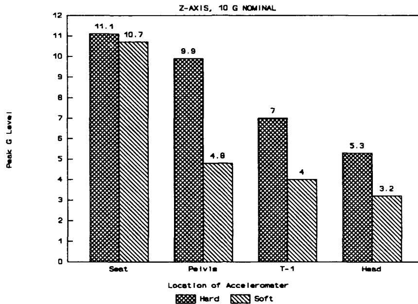
Figure 14. Hard vs. Soft Seat Comparison.
