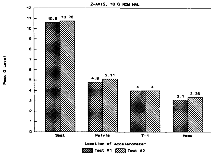
Figure 6. Soft Seat Repeatability.
