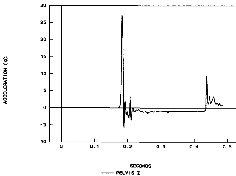
NBDL VERTICAL ACCELERATOR TEST - LZ0108 12 AUG 87
