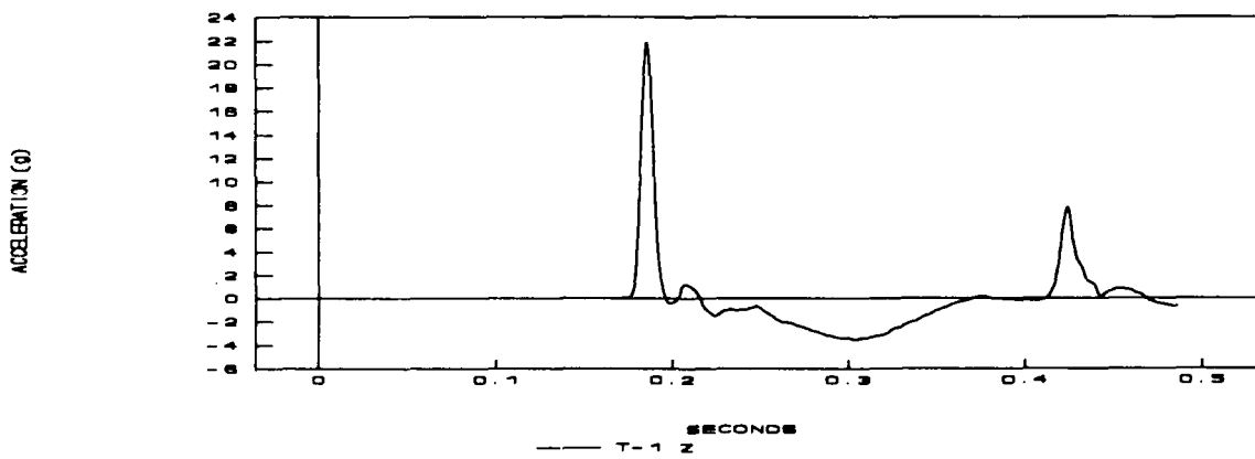
Figure 13. Shock Propagation through Pelvis and T-1 Hard Seat.
