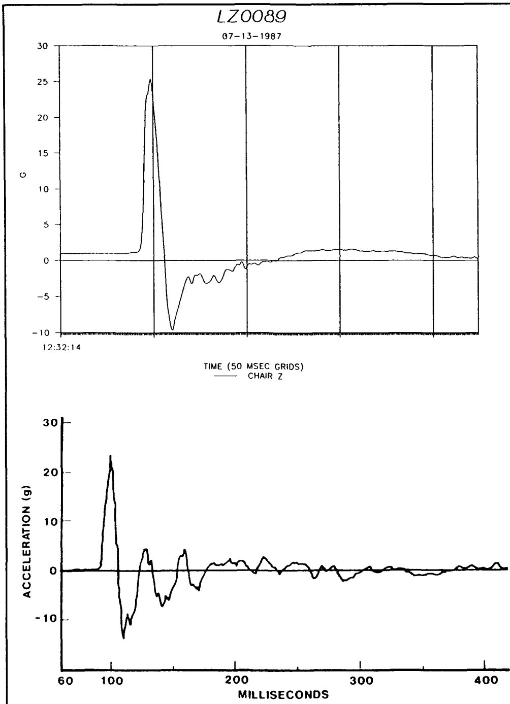
Figure 1. Comparisons of Shock Forces Measured on Vertical Accelerator (top) and USS YORKTOWN (CG-48).
