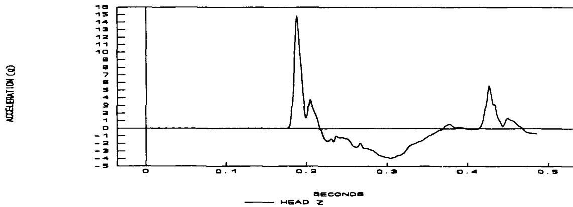
NBDL VERTICAL ACCELERATOR TEST - LZ0117 18 NOVEMBER 87
