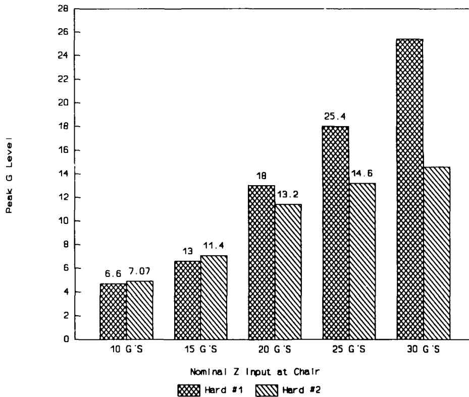
Figure 10. Hard Seat Pelvis X Comparison.
