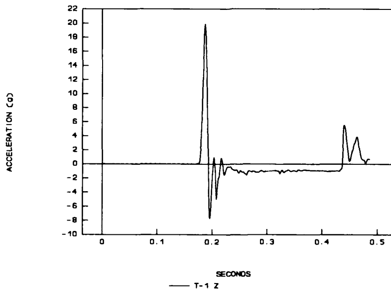
Figure 20. T-1 Z-axis Response to Actual and Simulated Shock Pulses.
