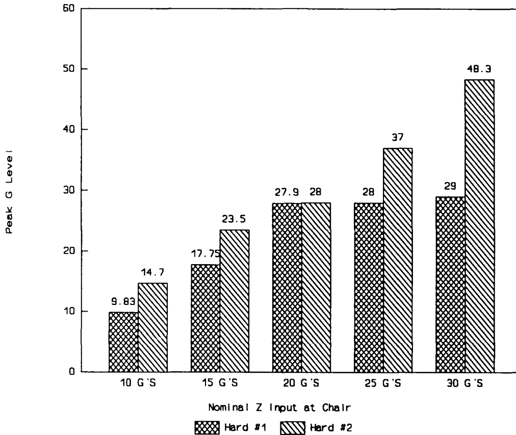
Figure 11. Hard Seat Pelvis Z Comparison.
