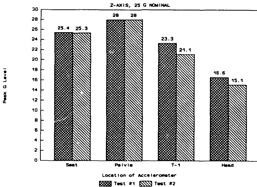
Figure 9. Hard Seat Repeatability.
