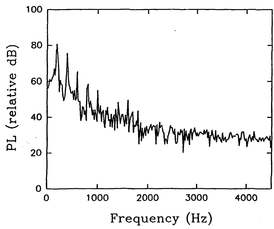
Figure 6(d) Pressure Distribution and Frequency Spectra Obtained at 2920 rpm at Location 4.
