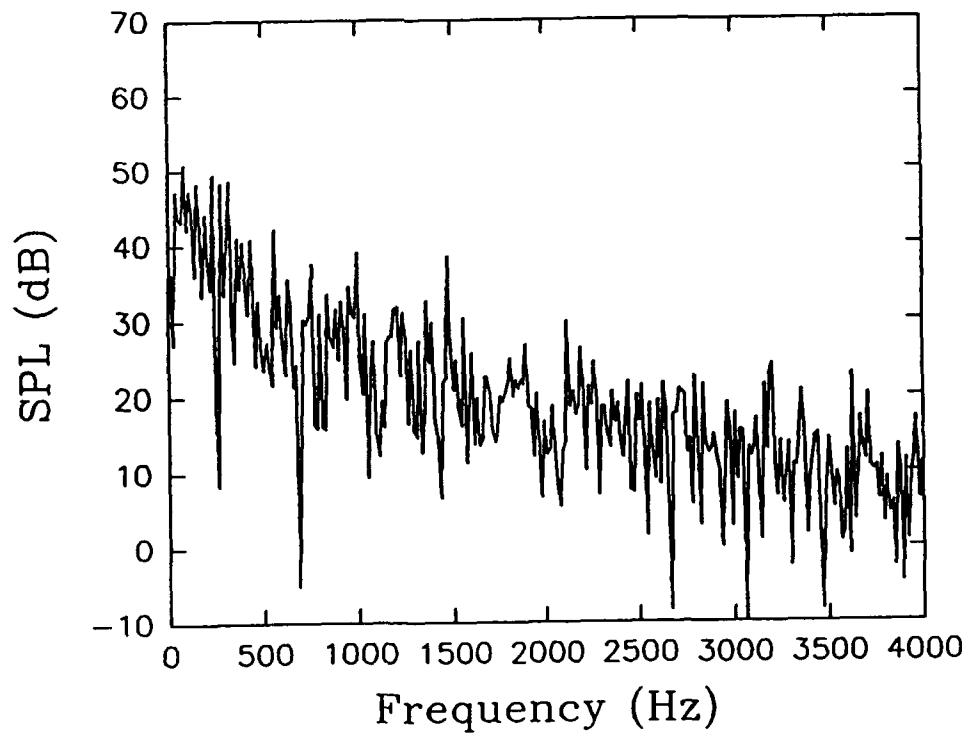
Figure 18(a) Airborne Noise Characteristics and Frequency Spectra Obtained with the Metal Casing and the aid of a Controller at 2340 rpm at Location 1.
