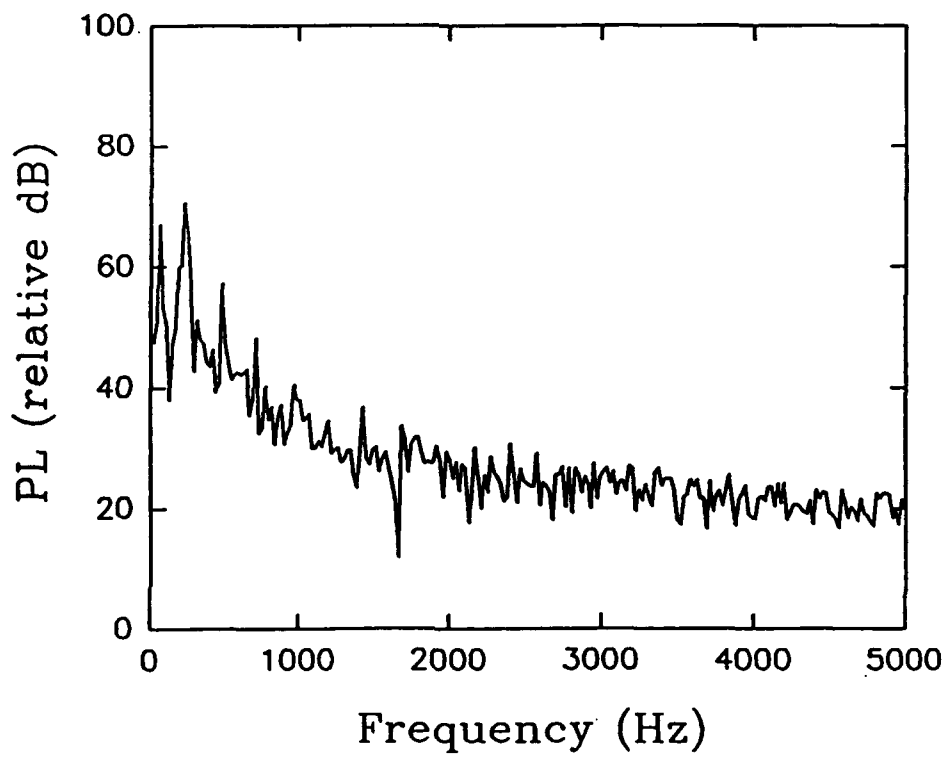
Figure 5(f) Pressure Distribution and Frequency Spectra Obtained at 3510 rpm at Location 6.
