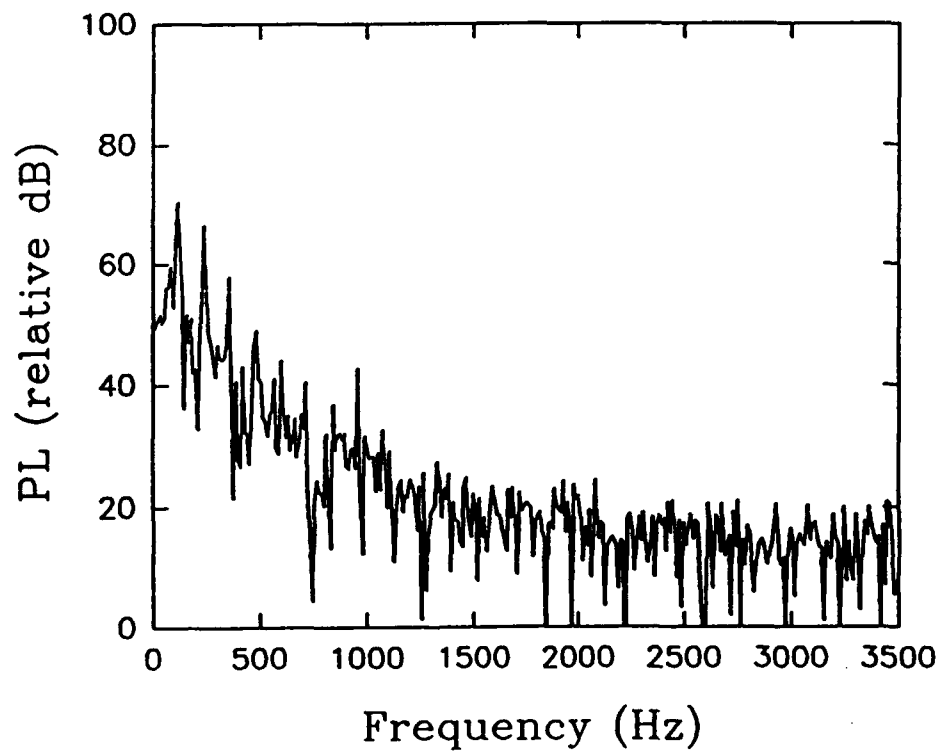
Figure 8(d) Pressure Distribution and Frequency Spectra Obtained at 1770 rpm at Location 4.
