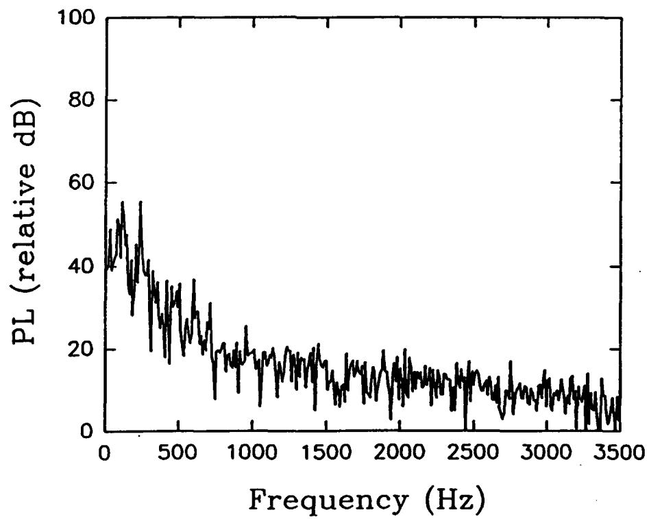
Figure 8(e) Pressure Distribution and Frequency Spectra Obtained at 1770 rpm at Location 5.
