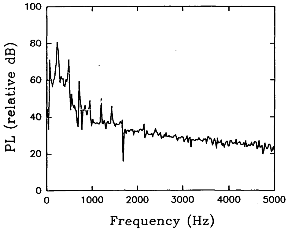
Figure 5(g) Pressure Distribution and Frequency Spectra Obtained at 3510 rpm at Location 7.
