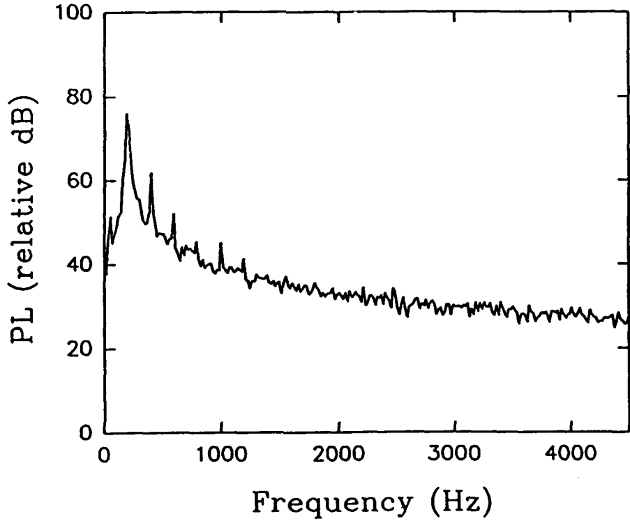
Figure 6(e) Pressure Distribution and Frequency Spectra Obtained at 2920 rpm at Location 5.
