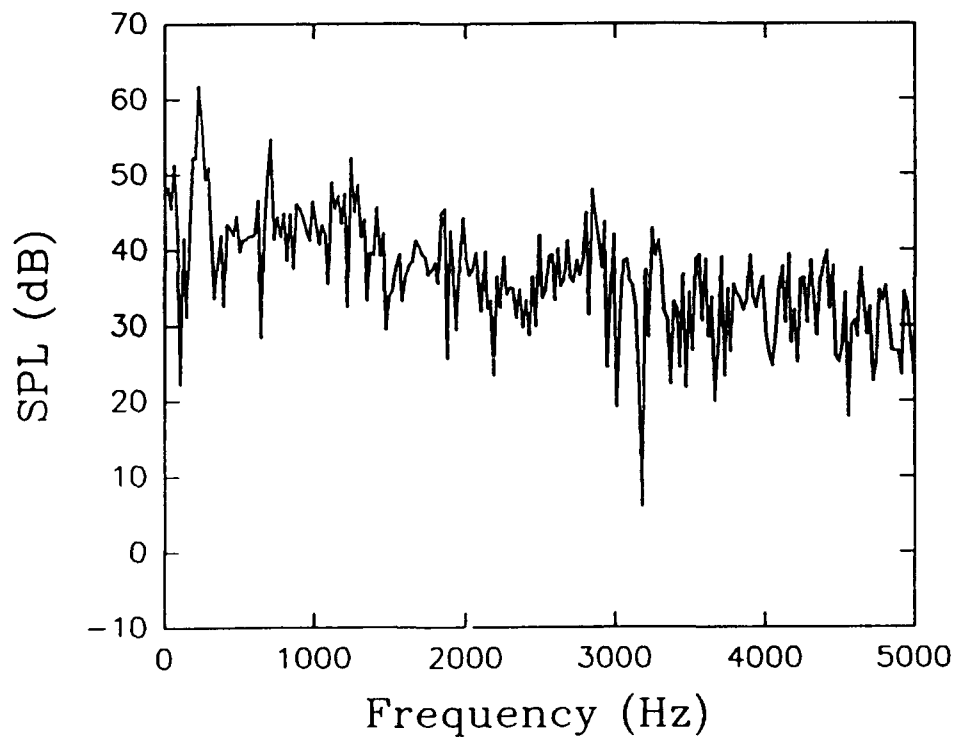
Figure 19(a) Instantaneous Airborne Noise Characteristics and Frequency Spectra Obtained with the Metal Casing and the aid of a Controller at 3510 rpm at Location 1.
