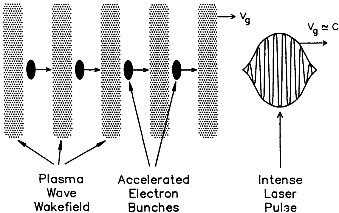
Fig. 2: Schematic of the laser wakefield accelerator (LWFA). The radiation (ponderomotive) force of an intense laser pulse drives plasma waves (wakefields) with phase velocities \simeq c which trap and accelerate trailing electron bunches.
