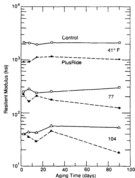
Figure 7. PlusRide: Resilient modulus vs aging time and test temperature (after Stewart and Mogawer 1988).
