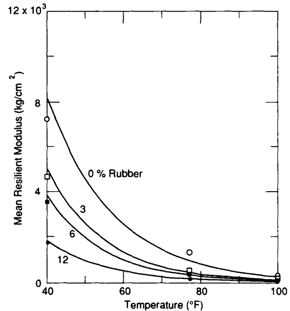
Figure 2. Mean resilient modulus for a 0.10-second load time of four mix designs based on the PlusRide concept.
